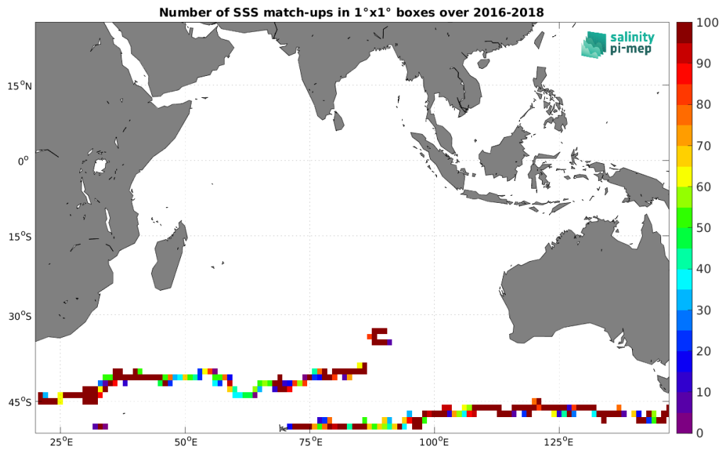
Figure 3: Number of SSS match-ups between Surface drifters SSS and the SMAP SSS L3 v5.0 - 8-Day running (JPL) SSS product for the Indian Ocean Pi-MEP region over 1^\circ \times 1^\circ boxes and for the full satellite product period.
