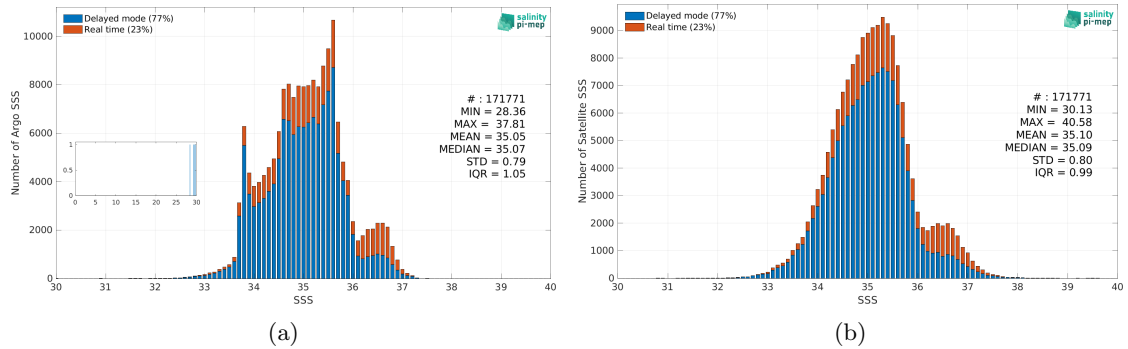
Figure 2: Histograms of SSS from Argo (a) and SMAP SSS L3 v5.0 - 8-Day running (JPL) (b) considering all match-up pairs per bins of 0.1 over the Indian Ocean Pi-MEP region and for the full satellite product period.
