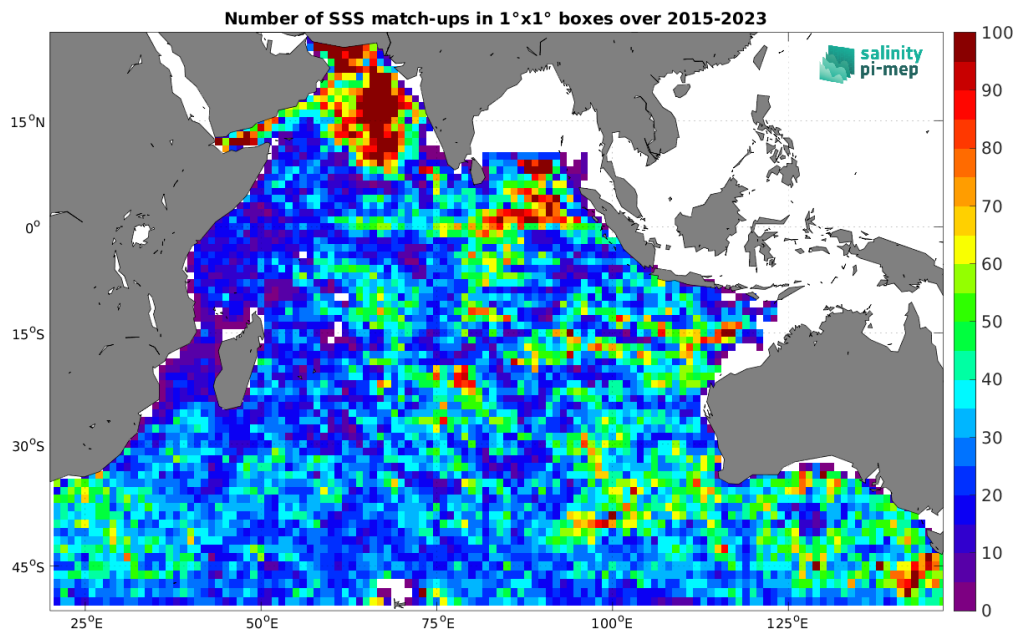
Figure 4: Number of SSS match-ups between Argo SSS and the SMAP SSS L3 v5.0 - 8-Day running (JPL) SSS product for the Indian Ocean Pi-MEP region over 1^\circ \times 1^\circ boxes and for the full satellite product period.
