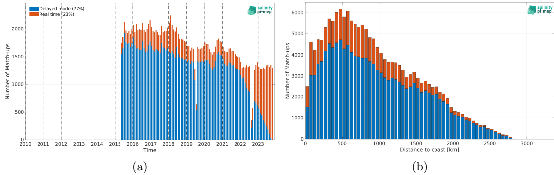
Figure 1: Number of match-ups between Argo and SMAP SSS L3 v5.0 - 8-Day running (JPL) SSS as a function of time (a) and as function of the distance to coast (b) over the Indian Ocean Pi-MEP region and for the full satellite product period.
