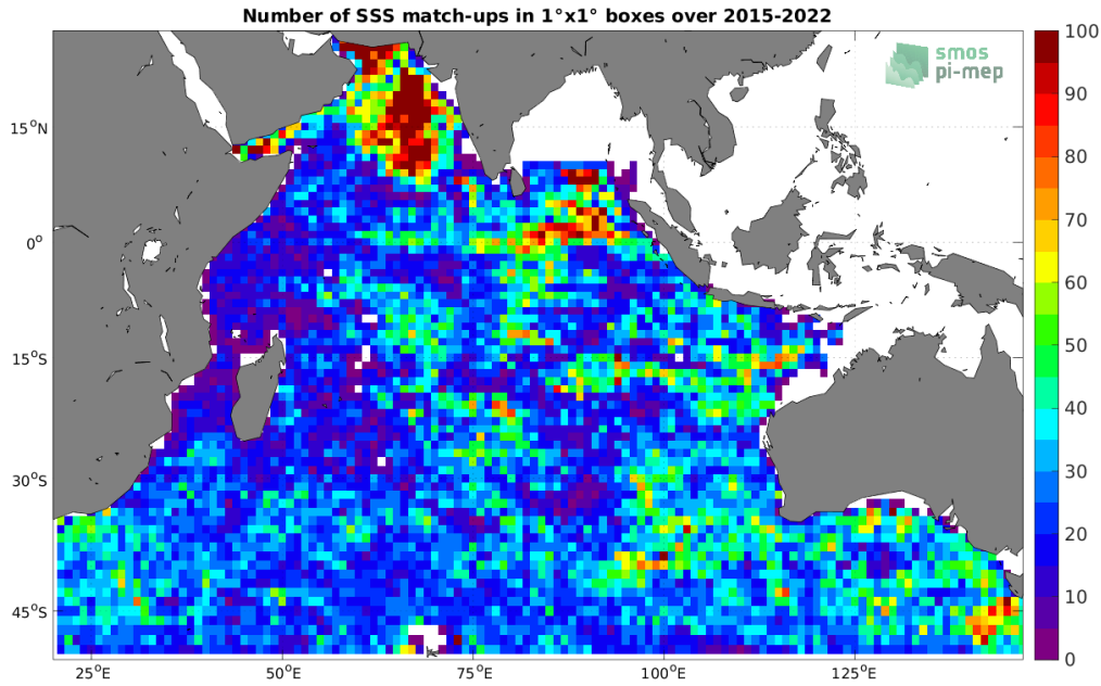
Figure 4: Number of SSS match-ups between Argo SSS and the SMAP SSS L3 v5.0 - 8-Day running (JPL) SSS product for the Indian Ocean Pi-MEP region over 1^\circ \times 1^\circ boxes and for the full satellite product period.
