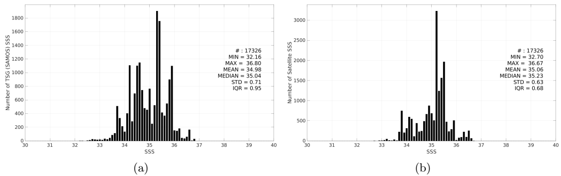
Figure 3: Histograms of SSS from TSG (SAMOS) (a) and SMAP SSS L3 v5.0 - Monthly (JPL) (b) considering all match-up pairs per bins of 0.1 over the Indian Ocean Pi-MEP region and for the full satellite product period.
