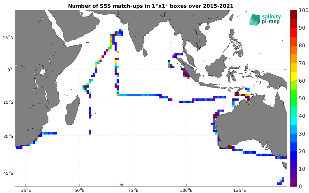
Figure 5: Number of SSS match-ups between TSG (SAMOS) SSS and the SMAP SSS L3 v5.0 - Monthly (JPL) SSS product for the Indian Ocean Pi-MEP region over 1^\circ \times 1^\circ boxes and for the full satellite product period.
