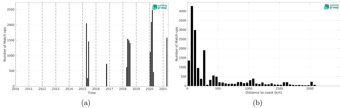
Figure 2: Number of match-ups between TSG (SAMOS) and SMAP SSS L3 v5.0 - Monthly (JPL) SSS as a function of time (a) and as function of the distance to coast (b) over the Indian Ocean Pi-MEP region and for the full satellite product period.
