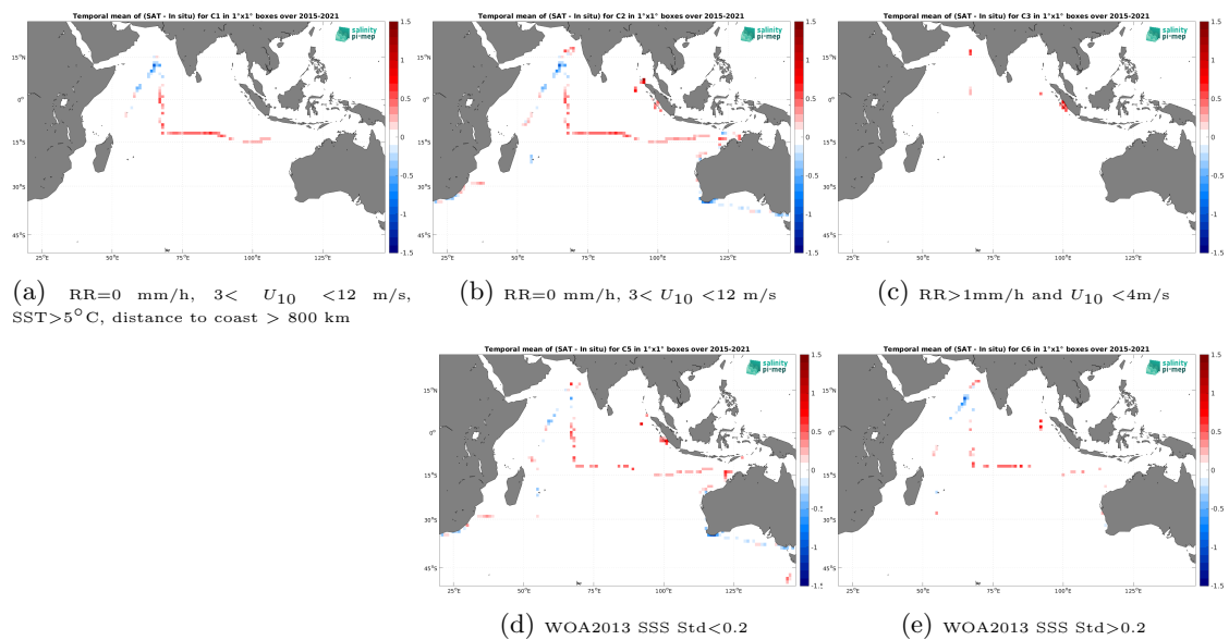
Figure 14: Temporal mean gridded over spatial boxes of size 1^\circ \times 1^\circ of \Delta SSS (SMAP SSS L3 v5.0 - Monthly (JPL) - TSG (SAMOS)) for 5 different subdatasets corresponding to: RR=0 mm/h, 3 < U_{10} < 12 m/s, SST > 5°C, distance to coast > 800 km (a), RR=0 mm/h, 3 < U_{10} < 12 m/s (b), RR > 1mm/h and U_{10} < 4 m/s (c), WOA2013 SSS Std < 0.2 (d), WOA2013 SSS Std > 0.2 (e).
