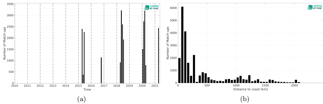
Figure 1: Number of match-ups between TSG (SAMOS) and SMAP SSS L3 v5.0 - Monthly (JPL) SSS as a function of time (a) and as function of the distance to coast (b) over the Indian Ocean Pi-MEP region and for the full satellite product period.
