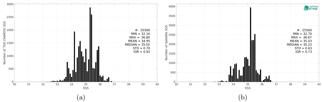
Figure 2: Histograms of SSS from TSG (SAMOS) (a) and SMAP SSS L3 v5.0 - Monthly (JPL) (b) considering all match-up pairs per bins of 0.1 over the Indian Ocean Pi-MEP region and for the full satellite product period.
