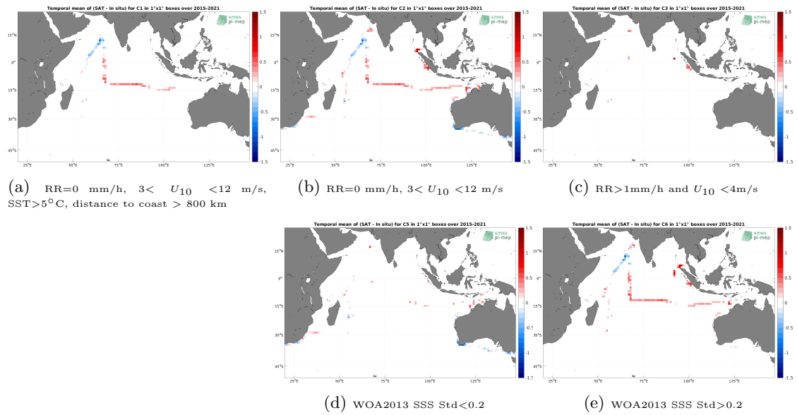
Figure 12: Temporal mean gridded over spatial boxes of size 1^\circ \times 1^\circ of \Delta SSS (SMAP SSS L3 v5.0 - Monthly (JPL) - TSG (SAMOS)) for 5 different subdatasets corresponding to:RR=0 mm/h, 3 < U_{10} < 12 m/s, SST >5^\circ C, distance to coast > 800 km (a), RR=0 mm/h, 3 < U_{10} < 12 m/s (b), RR >1 mm/h and U_{10} < 4 m/s (c), WOA2013 SSS Std <0.2 (d), WOA2013 SSS Std >0.2 (e).
