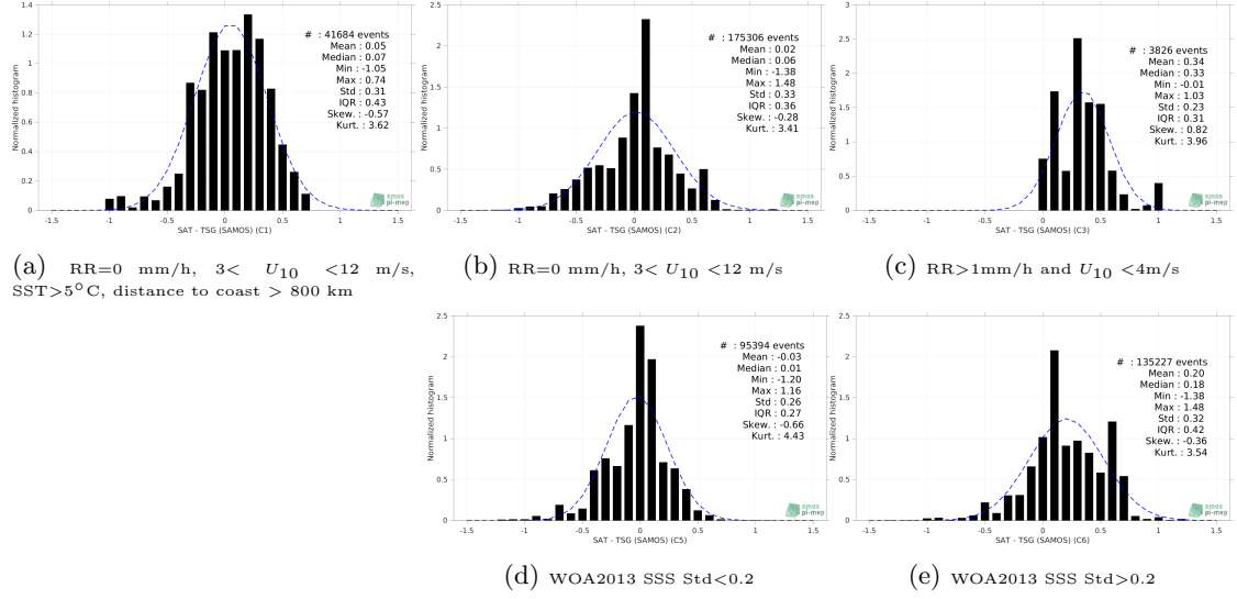
Figure 13: Normalized histogram of \Delta SSS (SMAP SSS L3 v5.0 - Monthly (JPL) - TSG (SAMOS)) for 5 different subdatasets corresponding to: RR=0 mm/h, 3 < U_{10} < 12 m/s, SST > 5°C, distance to coast > 800 km (a), RR=0 mm/h, 3 < U_{10} < 12 m/s (b), RR > 1mm/h and U_{10} < 4 m/s (c), WOA2013 SSS Std < 0.2 (d), WOA2013 SSS Std > 0.2 (e).
