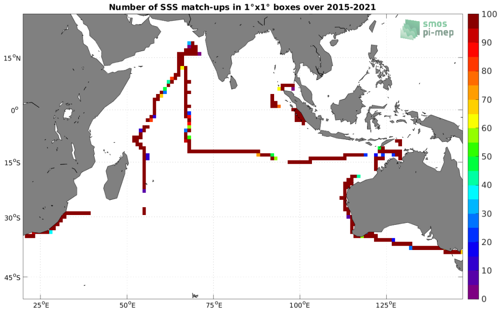
Figure 4: Number of SSS match-ups between TSG (SAMOS) SSS and the SMAP SSS L3 v5.0 - Monthly (JPL) SSS product for the Indian Ocean Pi-MEP region over 1^\circ \times 1^\circ boxes and for the full satellite product period.
