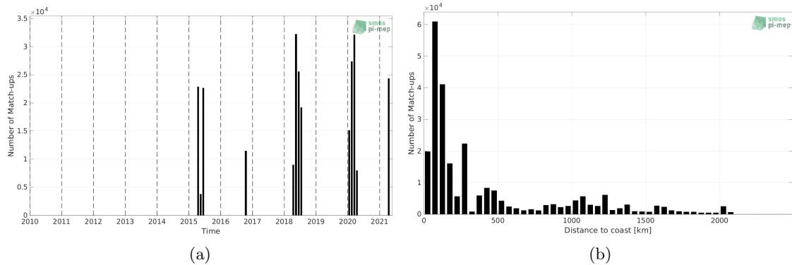
Figure 1: Number of match-ups between TSG (SAMOS) and SMAP SSS L3 v5.0 - Monthly (JPL) SSS as a function of time (a) and as function of the distance to coast (b) over the Indian Ocean Pi-MEP region and for the full satellite product period.
