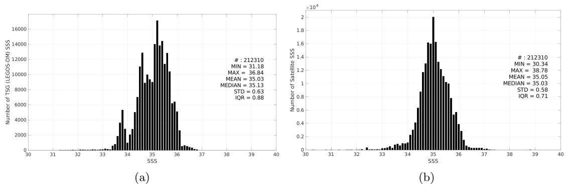
Figure 3: Histograms of SSS from TSG (LEGOS-DM) (a) and SMAP SSS L3 v5.0 - Monthly (JPL) (b) considering all match-up pairs per bins of 0.1 over the Indian Ocean Pi-MEP region and for the full satellite product period.
