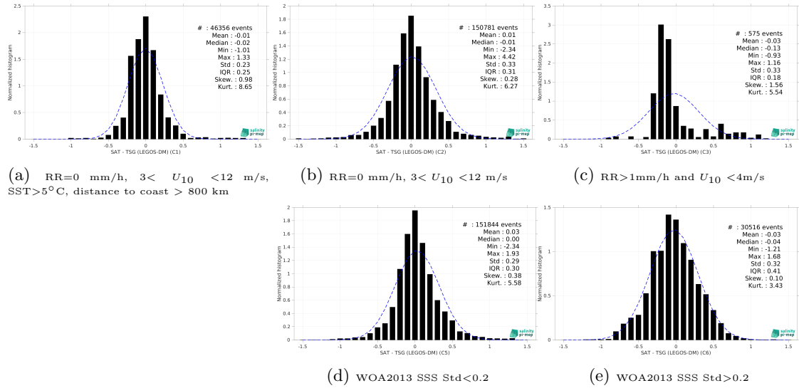
Figure 15: Normalized histogram of \Delta SSS (SMAP SSS L3 v5.0 - Monthly (JPL) - TSG (LEGOS-DM)) for 5 different subdatasets corresponding to: RR=0 mm/h, 3 < U_{10} < 12 m/s, SST>5°C, distance to coast > 800 km (a), RR=0 mm/h, 3 < U_{10} < 12 m/s (b), RR>1mm/h and U_{10} < 4 m/s (c), WOA2013 SSS Std<0.2 (d), WOA2013 SSS Std>0.2 (e).
