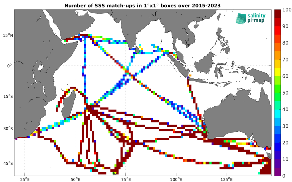
Figure 5: Number of SSS match-ups between TSG (LEGOS-DM) SSS and the SMAP SSS L3 v5.0 - Monthly (JPL) SSS product for the Indian Ocean Pi-MEP region over 1^\circ \times 1^\circ boxes and for the full satellite product period.
