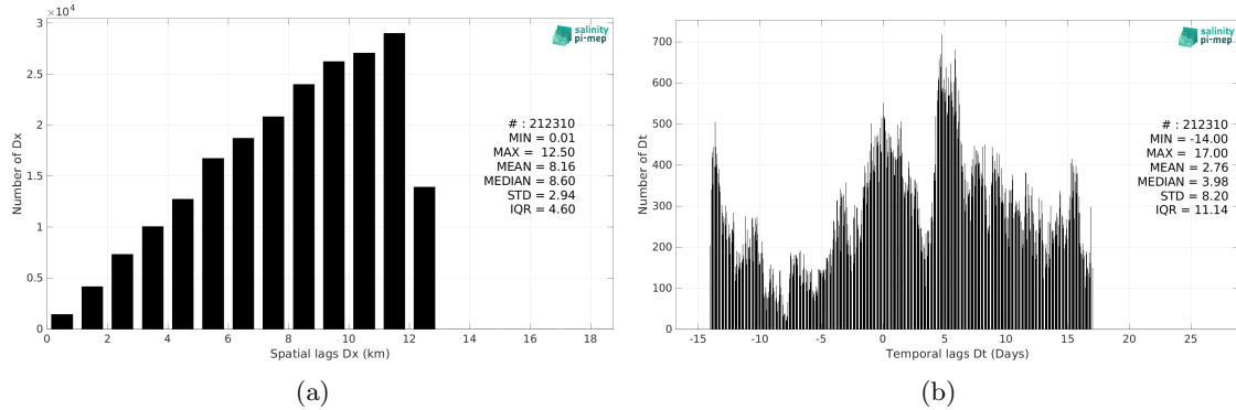
Figure 6: Histograms of the spatial (a) and temporal (b) lags between the location/time of the TSG (LEGOS-DM) measurement and the date of the corresponding SMAP SSS L3 v5.0 - Monthly (JPL) SSS pixel.
