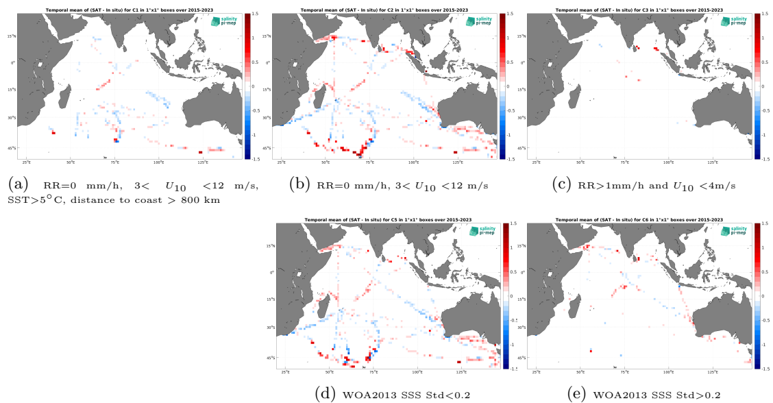
Figure 14: Temporal mean gridded over spatial boxes of size 1^\circ \times 1^\circ of \Delta SSS (SMAP SSS L3 v5.0 - Monthly (JPL) - TSG (LEGOS-DM)) for 5 different subdatasets corresponding to: RR=0 mm/h, 3 < U_{10} < 12 m/s, SST > 5^\circ\text{C} , distance to coast > 800 km (a), RR=0 mm/h, 3 < U_{10} < 12 m/s (b), RR > 1 mm/h and U_{10} < 4 m/s (c), WOA2013 SSS Std < 0.2 (d), WOA2013 SSS Std > 0.2 (e).
