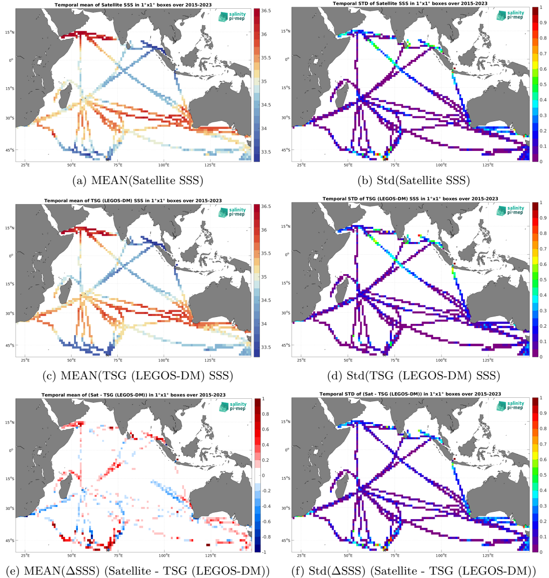
Figure 7: Temporal mean (left) and Std (right) of SSS from SMAP SSS L3 v5.0 - Monthly (JPL) (top), TSG (LEGOS-DM) (middle), and of \Delta SSS (Satellite - TSG (LEGOS-DM)). Only match-up pairs are used to generate these maps.
