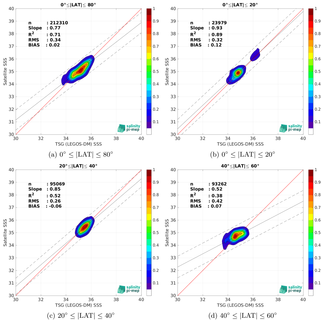
Figure 10: Contour maps of the concentration of SMAP SSS L3 v5.0 - Monthly (JPL) SSS (y-axis) versus TSG (LEGOS-DM) SSS (x-axis) at match-up pairs for different latitude bands. For each plot, the red line shows x=y . The black thin and dashed lines indicate a linear fit through the data cloud and the \pm 95\% confidence levels, respectively. The number match-up pairs n , the slope and R^2 coefficient of the linear fit, the root mean square (RMS) and the mean bias between satellite and in situ data are indicated for each latitude band in each plots.
