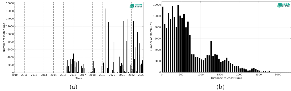
Figure 2: Number of match-ups between TSG (LEGOS-DM) and SMAP SSS L3 v5.0 - Monthly (JPL) SSS as a function of time (a) and as function of the distance to coast (b) over the Indian Ocean Pi-MEP region and for the full satellite product period.
