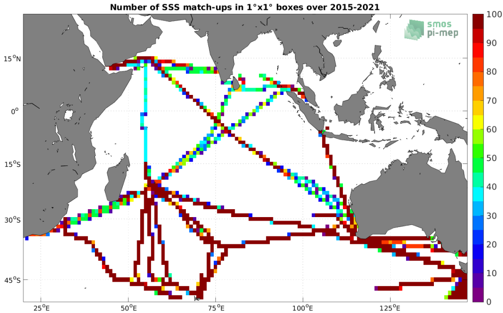
Figure 4: Number of SSS match-ups between TSG (LEGOS-DM) SSS and the SMAP SSS L3 v5.0 - Monthly (JPL) SSS product for the Indian Ocean Pi-MEP region over 1^\circ \times 1^\circ boxes and for the full satellite product period.
