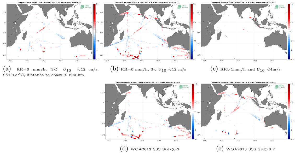
Figure 12: Temporal mean gridded over spatial boxes of size 1^\circ \times 1^\circ of \Delta SSS (SMAP SSS L3 v5.0 - Monthly (JPL) - TSG (LEGOS-DM)) for 5 different subdatasets corresponding to: RR=0 mm/h, 3 < U_{10} < 12 m/s, SST > 5^\circ\text{C} , distance to coast > 800 km (a), RR=0 mm/h, 3 < U_{10} < 12 m/s (b), RR > 1\text{mm/h} and U_{10} < 4\text{m/s} (c), WOA2013 SSS Std < 0.2 (d), WOA2013 SSS Std > 0.2 (e).
