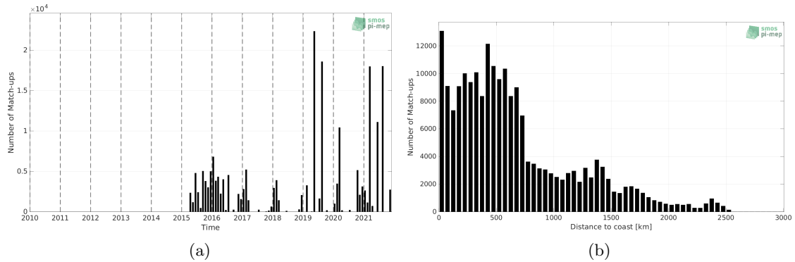
Figure 1: Number of match-ups between TSG (LEGOS-DM) and SMAP SSS L3 v5.0 - Monthly (JPL) SSS as a function of time (a) and as function of the distance to coast (b) over the Indian Ocean Pi-MEP region and for the full satellite product period.
