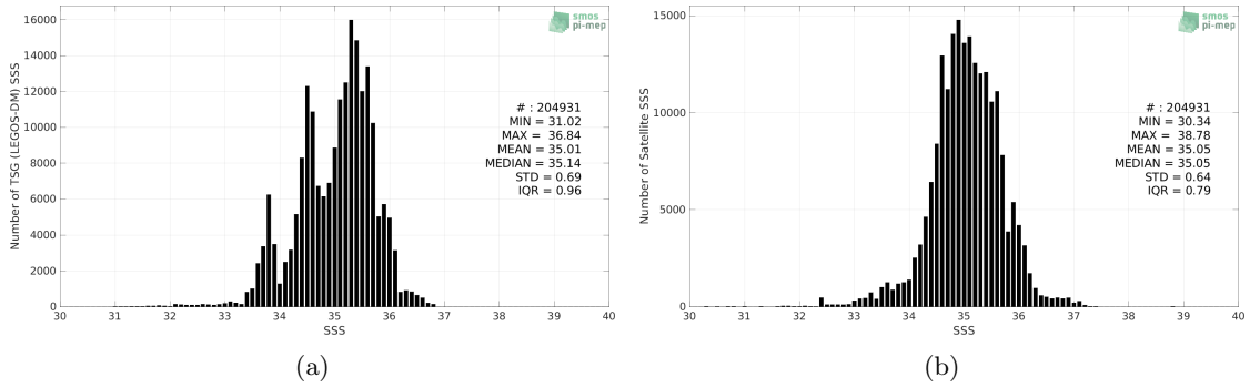
Figure 2: Histograms of SSS from TSG (LEGOS-DM) (a) and SMAP SSS L3 v5.0 - Monthly (JPL) (b) considering all match-up pairs per bins of 0.1 over the Indian Ocean Pi-MEP region and for the full satellite product period.
