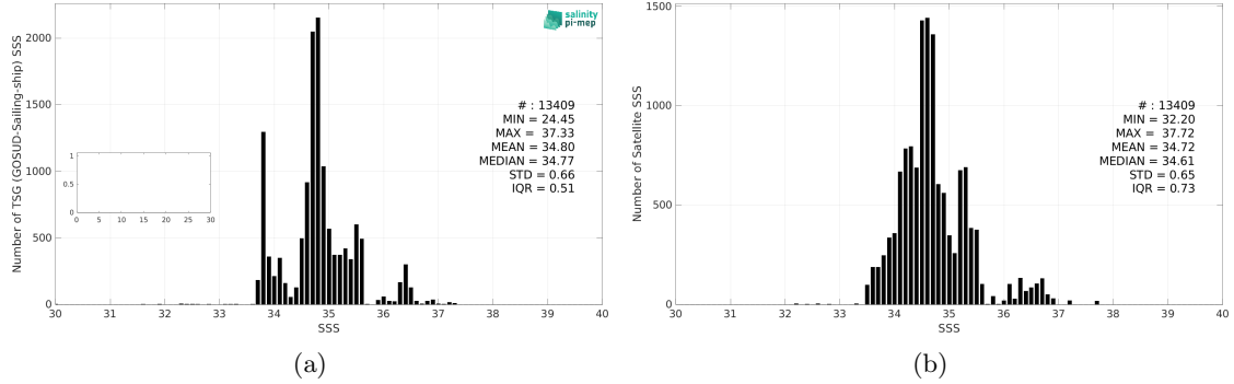
Figure 3: Histograms of SSS from TSG (GOSUD-Sailing-ship) (a) and SMAP SSS L3 v5.0 - Monthly (JPL) (b) considering all match-up pairs per bins of 0.1 over the Indian Ocean Pi-MEP region and for the full satellite product period.
