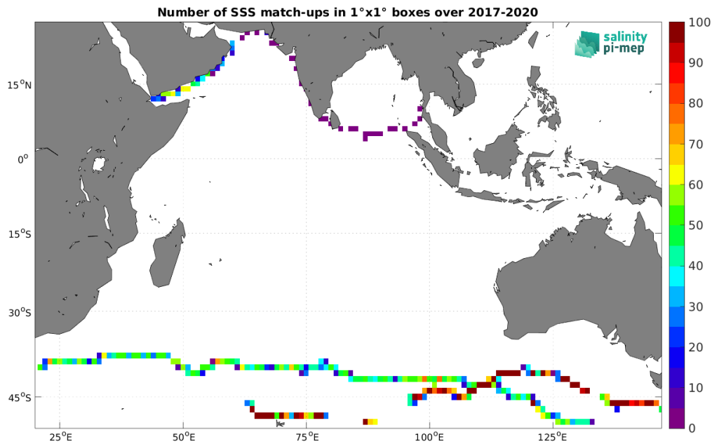
Figure 5: Number of SSS match-ups between TSG (GOSUD-Sailing-ship) SSS and the SMAP SSS L3 v5.0 - Monthly (JPL) SSS product for the Indian Ocean Pi-MEP region over 1^\circ \times 1^\circ boxes and for the full satellite product period.
