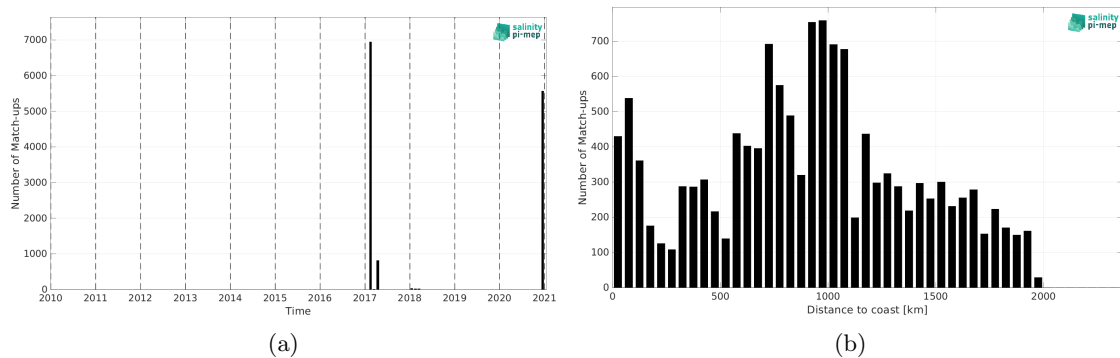
Figure 2: Number of match-ups between TSG (GOSUD-Sailing-ship) and SMAP SSS L3 v5.0 - Monthly (JPL) SSS as a function of time (a) and as function of the distance to coast (b) over the Indian Ocean Pi-MEP region and for the full satellite product period.
