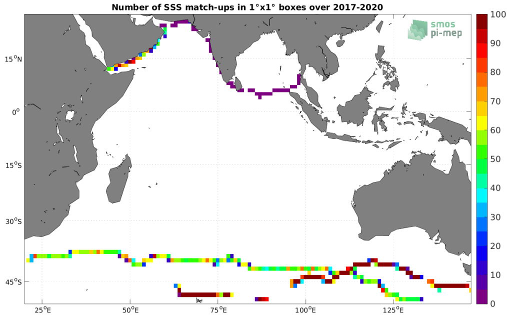
Figure 4: Number of SSS match-ups between TSG (GOSUD-Sailing-ship) SSS and the SMAP SSS L3 v5.0 - Monthly (JPL) SSS product for the Indian Ocean Pi-MEP region over 1^\circ \times 1^\circ boxes and for the full satellite product period.
