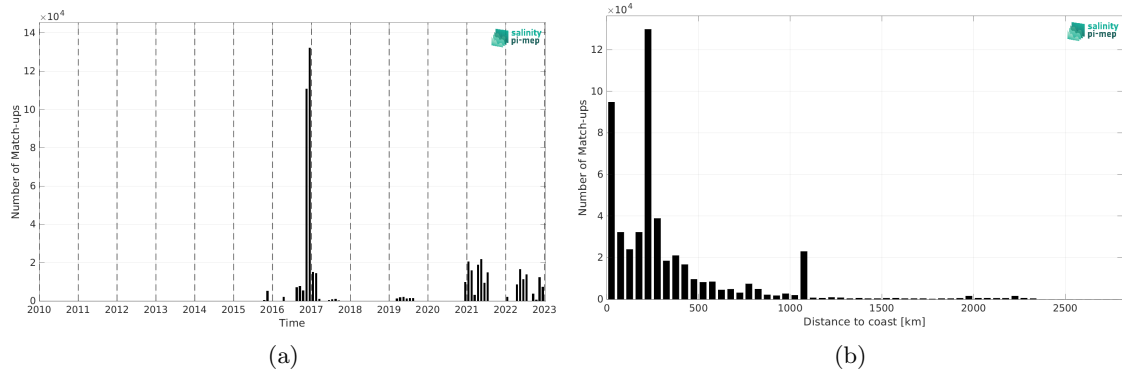
Figure 2: Number of match-ups between TSG (GOSUD-Research-vessel) and SMAP SSS L3 v5.0 - Monthly (JPL) SSS as a function of time (a) and as function of the distance to coast (b) over the Indian Ocean Pi-MEP region and for the full satellite product period.
