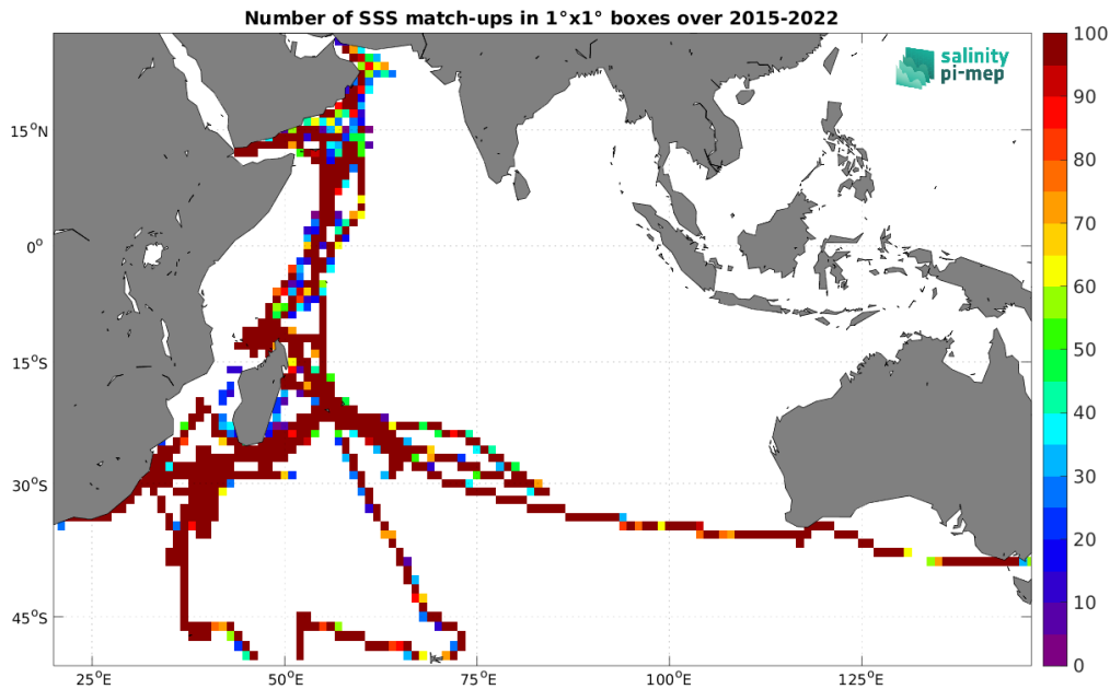
Figure 5: Number of SSS match-ups between TSG (GOSUD-Research-vessel) SSS and the SMAP SSS L3 v5.0 - Monthly (JPL) SSS product for the Indian Ocean Pi-MEP region over 1^\circ \times 1^\circ boxes and for the full satellite product period.
