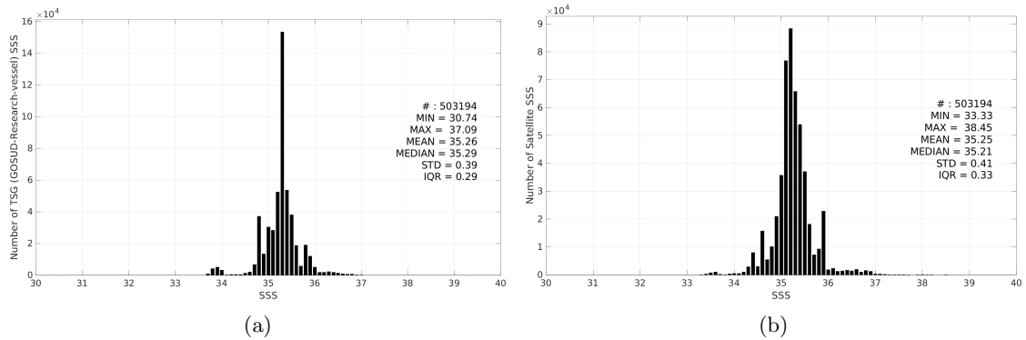
Figure 3: Histograms of SSS from TSG (GOSUD-Research-vessel) (a) and SMAP SSS L3 v5.0 - Monthly (JPL) (b) considering all match-up pairs per bins of 0.1 over the Indian Ocean Pi-MEP region and for the full satellite product period.
