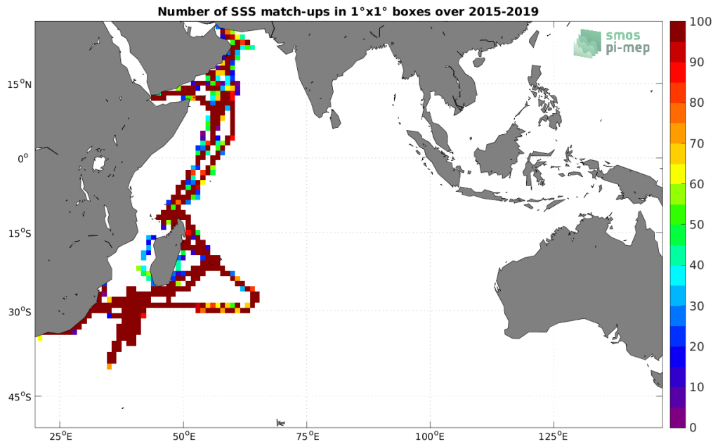
Figure 4: Number of SSS match-ups between TSG (GOSUD-Research-vessel) SSS and the SMAP SSS L3 v5.0 - Monthly (JPL) SSS product for the Indian Ocean Pi-MEP region over 1^\circ \times 1^\circ boxes and for the full satellite product period.
