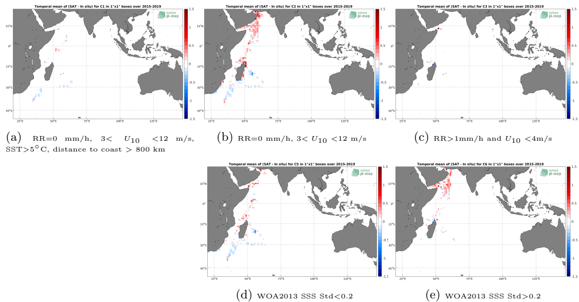
Figure 12: Temporal mean gridded over spatial boxes of size 1^\circ \times 1^\circ of \Delta\text{SSS} (SMAP SSS L3 v5.0 - Monthly (JPL) - TSG (GOSUD-Research-vessel)) for 5 different subdatasets corresponding to:RR=0 mm/h, 3 < U_{10} < 12 m/s, SST>5°C, distance to coast > 800 km (a), RR=0 mm/h, 3 < U_{10} < 12 m/s (b), RR>1mm/h and U_{10} < 4 m/s (c), WOA2013 SSS Std<0.2 (d), WOA2013 SSS Std>0.2 (e).
