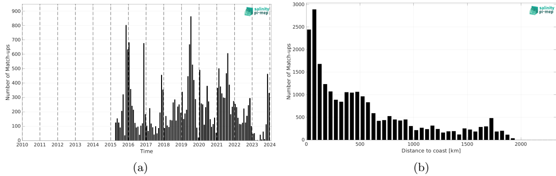
Figure 2: Number of match-ups between Marine mammals and SMAP SSS L3 v5.0 - Monthly (JPL) SSS as a function of time (a) and as function of the distance to coast (b) over the Indian Ocean Pi-MEP region and for the full satellite product period.
