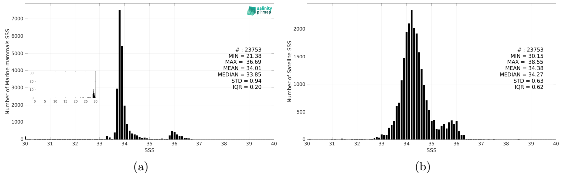
Figure 3: Histograms of SSS from Marine mammals (a) and SMAP SSS L3 v5.0 - Monthly (JPL) (b) considering all match-up pairs per bins of 0.1 over the Indian Ocean Pi-MEP region and for the full satellite product period.
