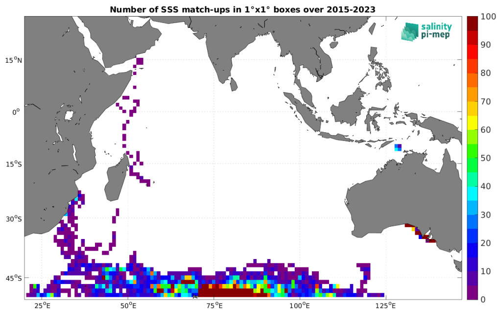
Figure 5: Number of SSS match-ups between Marine mammals SSS and the SMAP SSS L3 v5.0 - Monthly (JPL) SSS product for the Indian Ocean Pi-MEP region over 1^\circ \times 1^\circ boxes and for the full satellite product period.
