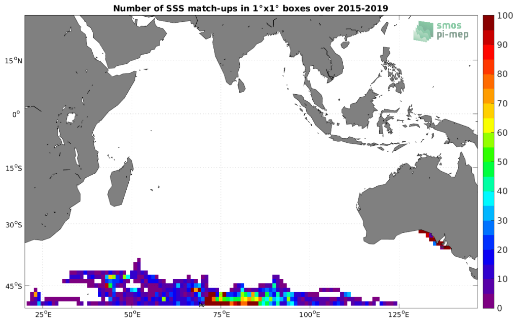
Figure 4: Number of SSS match-ups between Marine mammals SSS and the SMAP SSS L3 v5.0 - Monthly (JPL) SSS product for the Indian Ocean Pi-MEP region over 1^\circ \times 1^\circ boxes and for the full satellite product period.
