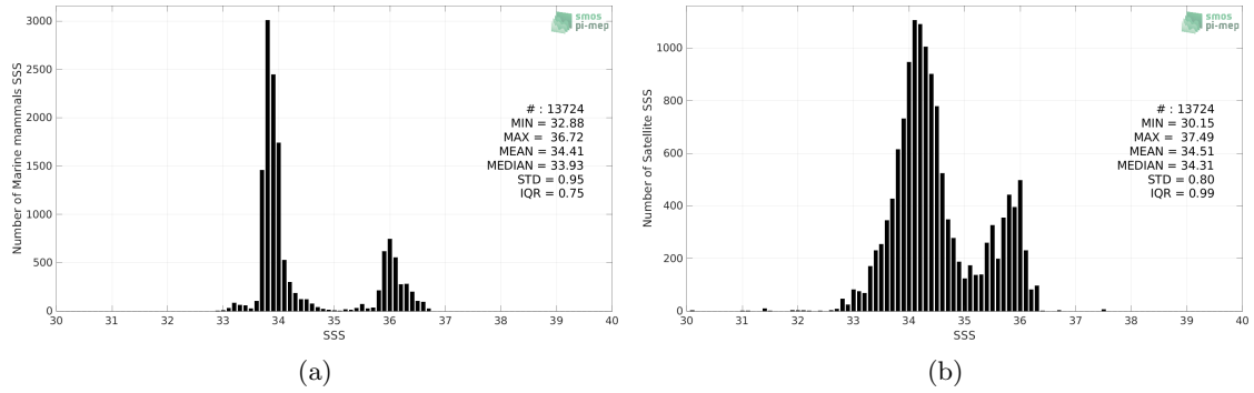
Figure 2: Histograms of SSS from Marine mammals (a) and SMAP SSS L3 v5.0 - Monthly (JPL) (b) considering all match-up pairs per bins of 0.1 over the Indian Ocean Pi-MEP region and for the full satellite product period.
