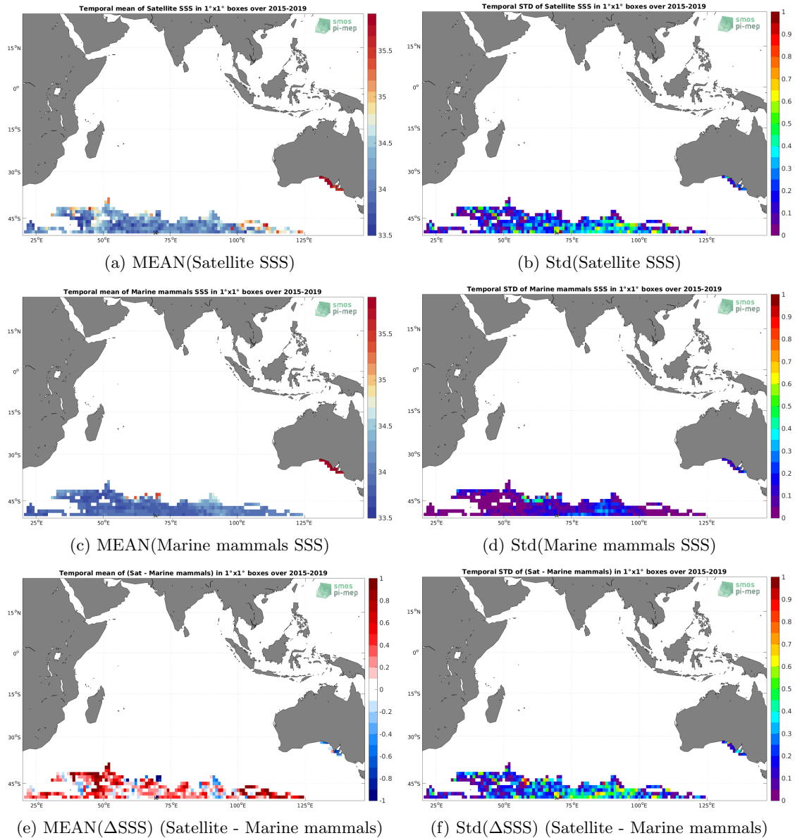
Figure 6: Temporal mean (left) and Std (right) of SSS from SMAP SSS L3 v5.0 - Monthly (JPL) (top), Marine mammals (middle), and of \Delta SSS (Satellite - Marine mammals). Only match-up pairs are used to generate these maps.
