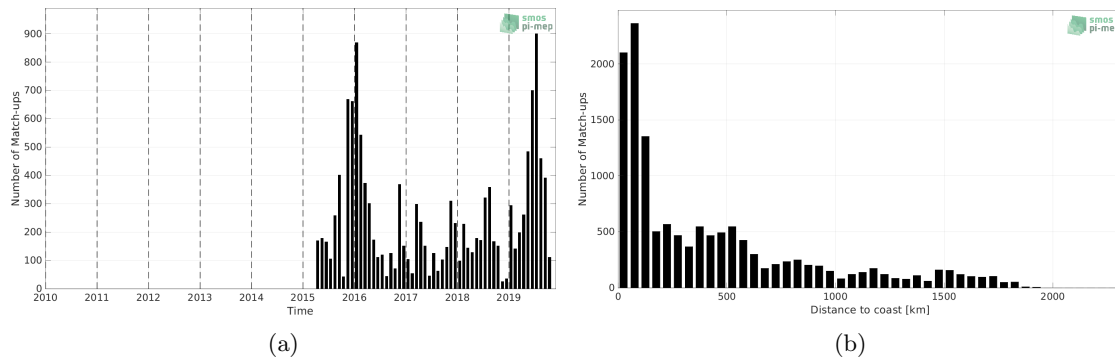
Figure 1: Number of match-ups between Marine mammals and SMAP SSS L3 v5.0 - Monthly (JPL) SSS as a function of time (a) and as function of the distance to coast (b) over the Indian Ocean Pi-MEP region and for the full satellite product period.
