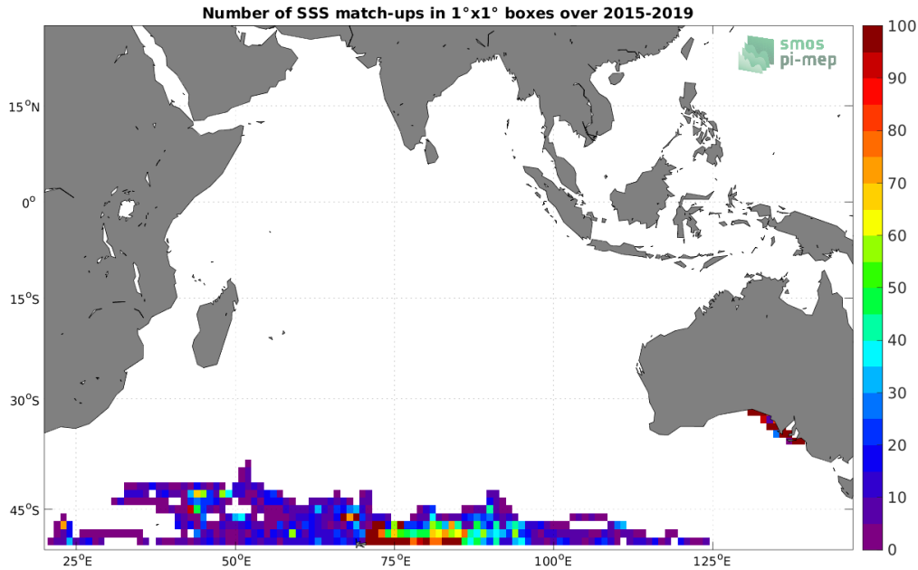
Figure 4: Number of SSS match-ups between Marine mammals SSS and the SMAP SSS L3 v5.0 - Monthly (JPL) SSS product for the Indian Ocean Pi-MEP region over 1^\circ \times 1^\circ boxes and for the full satellite product period.
