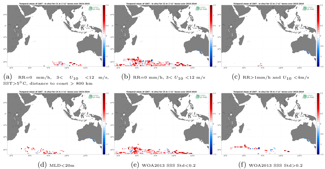
Figure 12: Temporal mean gridded over spatial boxes of size 1^\circ \times 1^\circ of \Delta SSS (SMAP SSS L3 v5.0 - Monthly (JPL) - Marine mammals) for 6 different subdatasets corresponding to:RR=0 mm/h, 3 < U_{10} < 12 m/s, SST >5^\circ C, distance to coast > 800 km (a), RR=0 mm/h, 3 < U_{10} < 12 m/s (b), RR >1 mm/h and U_{10} < 4 m/s (c),MLD <20 m (d),WOA2013 SSS Std <0.2 (e),WOA2013 SSS Std >0.2 (f).
