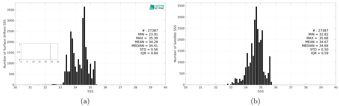
Figure 3: Histograms of SSS from Surface drifters (a) and SMAP SSS L3 v5.0 - Monthly (JPL) (b) considering all match-up pairs per bins of 0.1 over the Indian Ocean Pi-MEP region and for the full satellite product period.
