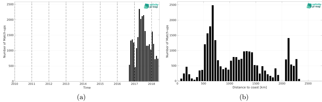
Figure 2: Number of match-ups between Surface drifters and SMAP SSS L3 v5.0 - Monthly (JPL) SSS as a function of time (a) and as function of the distance to coast (b) over the Indian Ocean Pi-MEP region and for the full satellite product period.
