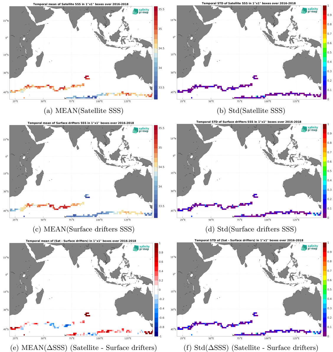
Figure 6: Temporal mean (left) and Std (right) of SSS from SMAP SSS L3 v5.0 - Monthly (JPL) (top), Surface drifters (middle), and of \Delta SSS (Satellite - Surface drifters). Only match-up pairs are used to generate these maps.
