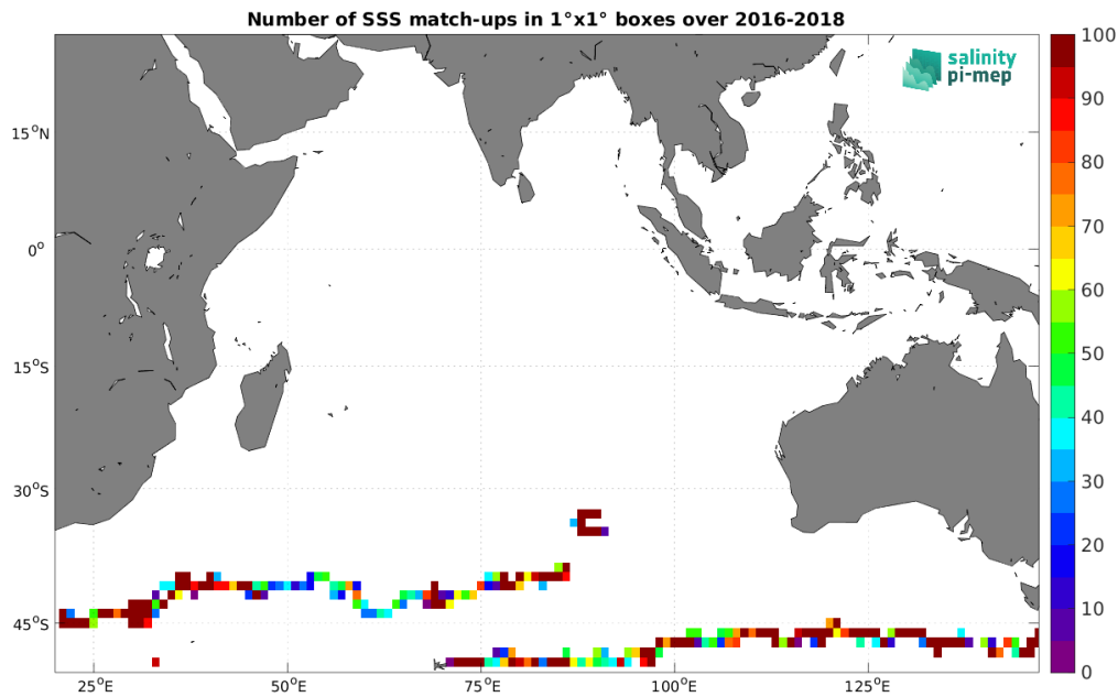
Figure 4: Number of SSS match-ups between Surface drifters SSS and the SMAP SSS L3 v5.0 - Monthly (JPL) SSS product for the Indian Ocean Pi-MEP region over 1^\circ \times 1^\circ boxes and for the full satellite product period.
