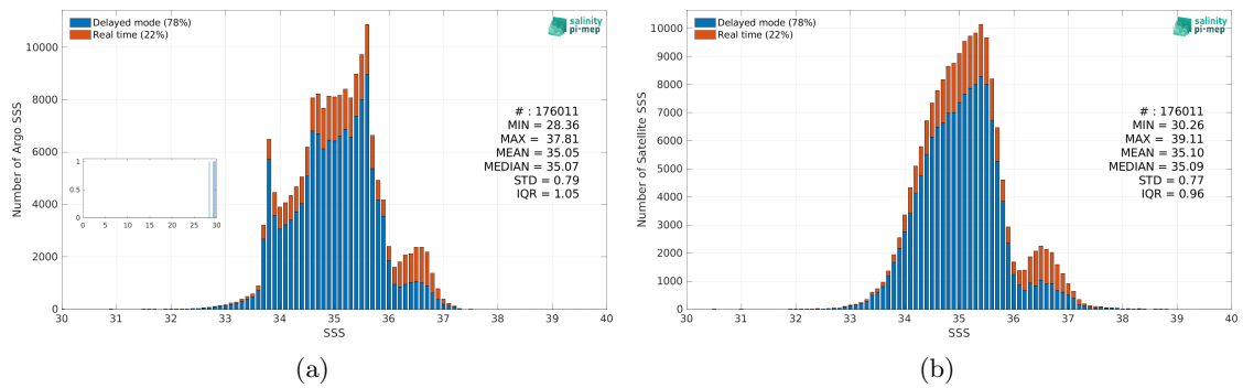
Figure 2: Histograms of SSS from Argo (a) and SMAP SSS L3 v5.0 - Monthly (JPL) (b) considering all match-up pairs per bins of 0.1 over the Indian Ocean Pi-MEP region and for the full satellite product period.
