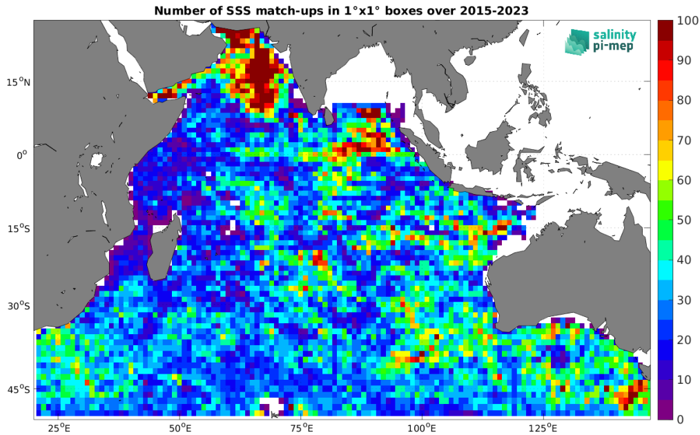
Figure 4: Number of SSS match-ups between Argo SSS and the SMAP SSS L3 v5.0 - Monthly (JPL) SSS product for the Indian Ocean Pi-MEP region over 1^\circ \times 1^\circ boxes and for the full satellite product period.
