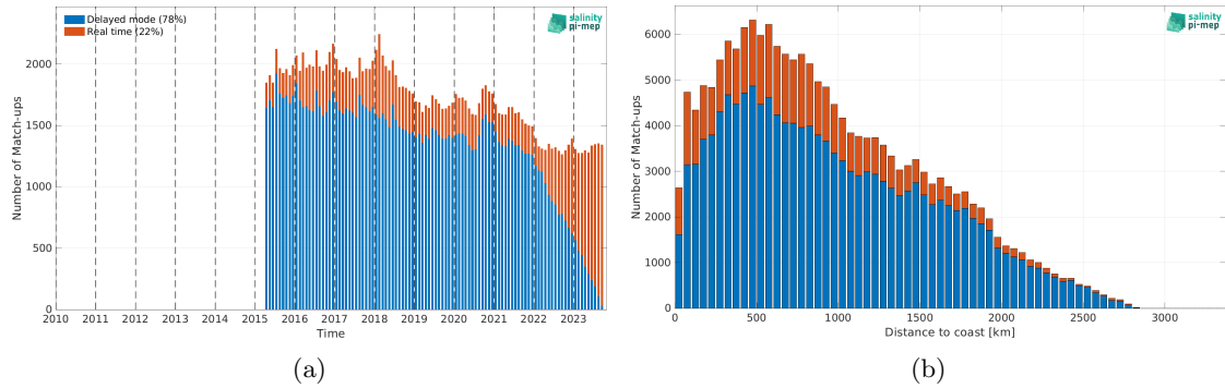
Figure 1: Number of match-ups between Argo and SMAP SSS L3 v5.0 - Monthly (JPL) SSS as a function of time (a) and as function of the distance to coast (b) over the Indian Ocean Pi-MEP region and for the full satellite product period.
