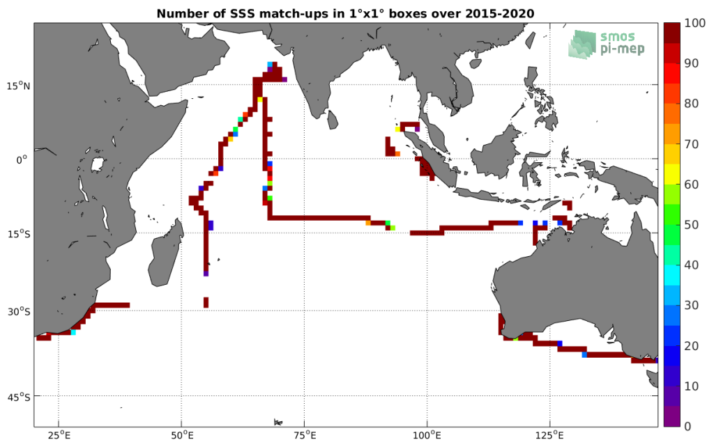
Figure 4: Number of SSS match-ups between TSG-SAMOS SSS and the SMAP-L3-JPL-V4.3-8DAY-RUNNING-60KM SSS product for the Indian Ocean Pi-MEP region over 1°x1° boxes and for the full satellite product period.
