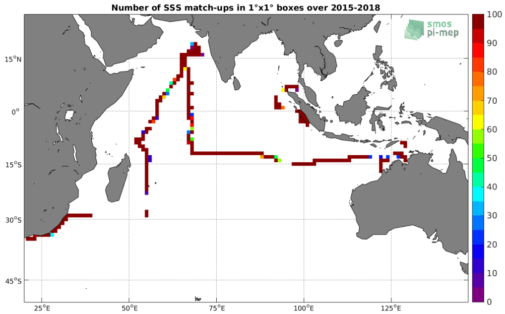
Figure 4: Number of SSS match-ups between TSG-SAMOS SSS and the SMAP-L3-JPL-V4.3-8DAY-RUNNING-60KM SSS product for the Indian Ocean Pi-MEP region over 1°x1° boxes and for the full satellite product period.
