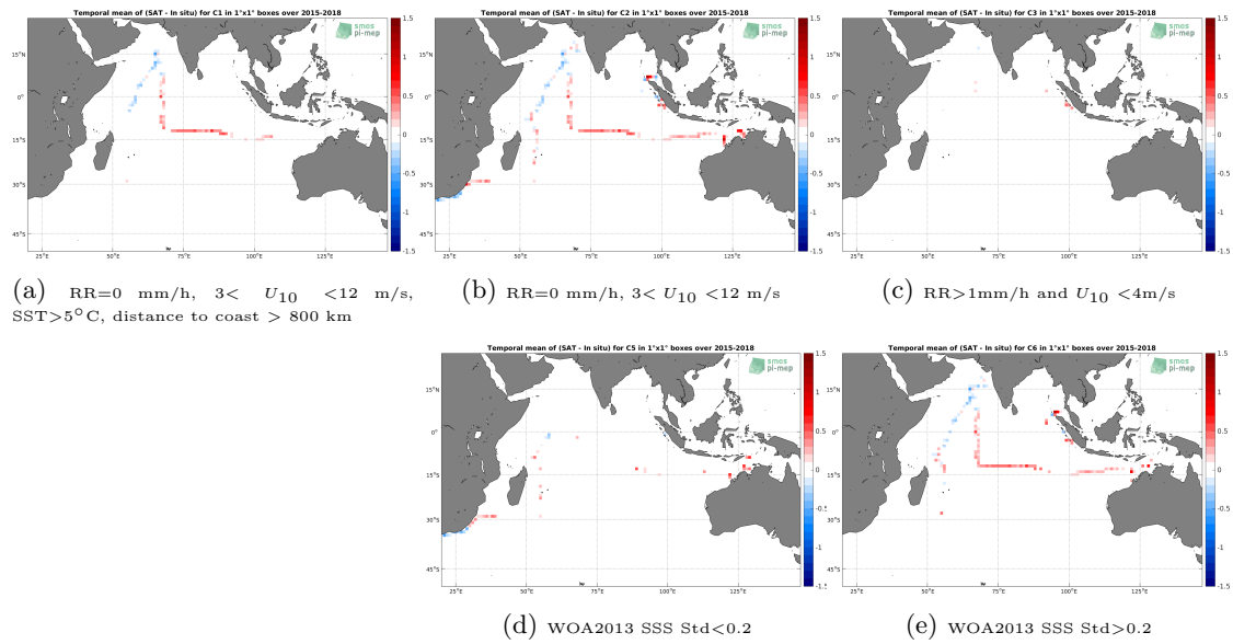
Figure 12: Temporal mean gridded over spatial boxes of size 1^\circ \times 1^\circ of \Delta SSS (SMAP-L3-JPL-V4.3-8DAY-RUNNING-60KM - TSG-SAMOS) for 5 different subdatasets corresponding to:RR=0 mm/h, 3 < U_{10} < 12 m/s, SST >5^\circ C, distance to coast > 800 km (a), RR=0 mm/h, 3 < U_{10} < 12 m/s (b), RR >1 mm/h and U_{10} < 4 m/s (c), WOA2013 SSS Std <0.2 (d), WOA2013 SSS Std >0.2 (e).
