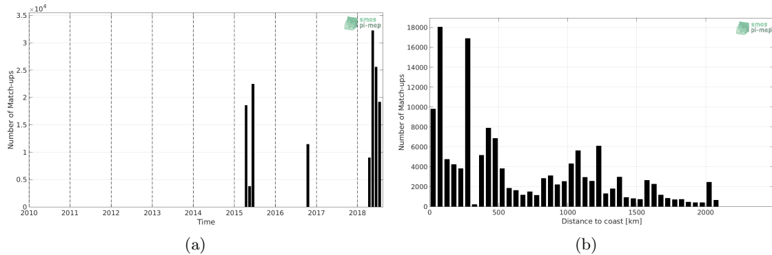
Figure 1: Number of match-ups between TSG-SAMOS and SMAP-L3-JPL-V4.3-8DAY-RUNNING-60KM SSS as a function of time (a) and as function of the distance to coast (b) over the Indian Ocean Pi-MEP region and for the full satellite product period.
