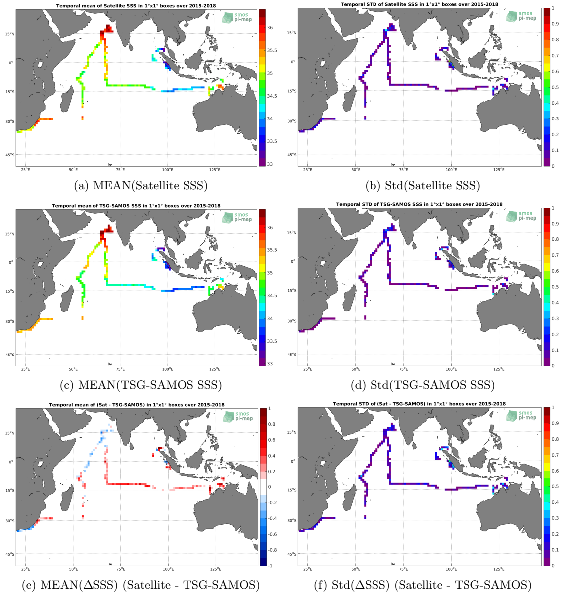
Figure 6: Temporal mean (left) and Std (right) of SSS from SMAP-L3-JPL-V4.3-8DAY-RUNNING-60KM (top), TSG-SAMOS (middle), and of \Delta SSS (Satellite - TSG-SAMOS). Only match-up pairs are used to generate these maps.
