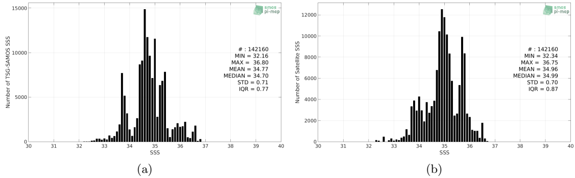
Figure 2: Histograms of SSS from TSG-SAMOS (a) and SMAP-L3-JPL-V4.3-8DAY-RUNNING-60KM (b) considering all match-up pairs per bins of 0.1 over the Indian Ocean Pi-MEP region and for the full satellite product period.
