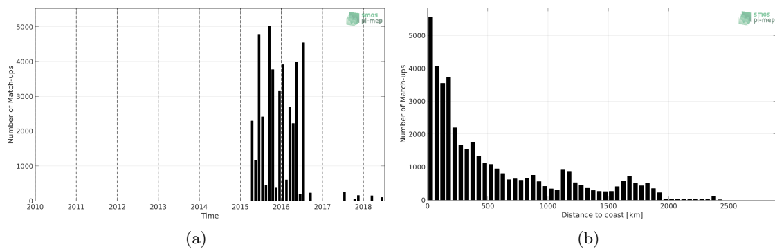
Figure 1: Number of match-ups between TSG-LEGOS-DM and SMAP-L3-JPL-V4.3-8DAY-RUNNING-60KM SSS as a function of time (a) and as function of the distance to coast (b) over the Indian Ocean Pi-MEP region and for the full satellite product period.
