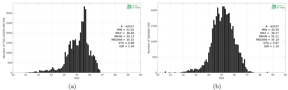
Figure 2: Histograms of SSS from TSG-LEGOS-DM (a) and SMAP-L3-JPL-V4.3-8DAY-RUNNING-60KM (b) considering all match-up pairs per bins of 0.1 over the Indian Ocean Pi-MEP region and for the full satellite product period.
