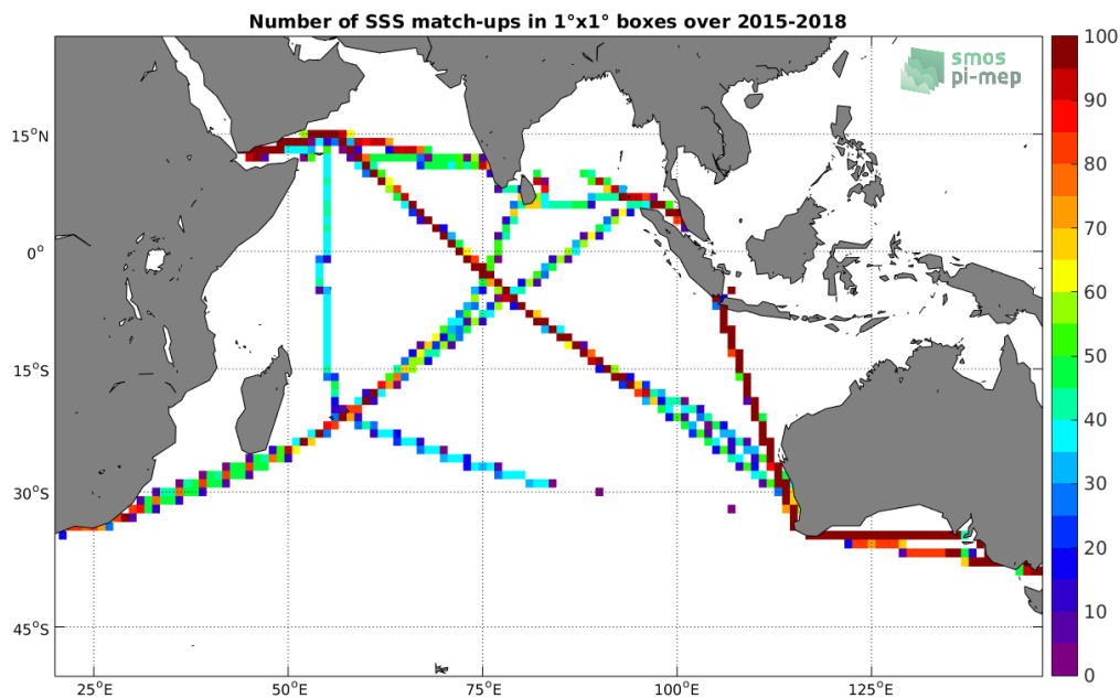
Figure 4: Number of SSS match-ups between TSG-LEGOS-DM SSS and the SMAP-L3-JPL-V4.3-8DAY-RUNNING-60KM SSS product for the Indian Ocean Pi-MEP region over 1^\circ \times 1^\circ boxes and for the full satellite product period.
