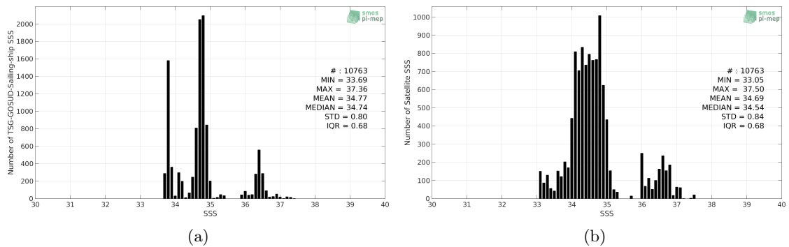
Figure 2: Histograms of SSS from TSG-GOSUD-Sailing-ship (a) and SMAP-L3-JPL-V4.3-8DAY-RUNNING-60KM (b) considering all match-up pairs per bins of 0.1 over the Indian Ocean Pi-MEP region and for the full satellite product period.
