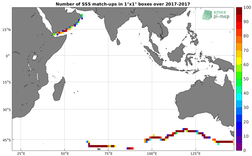
Figure 4: Number of SSS match-ups between TSG-GOSUD-Sailing-ship SSS and the SMAP-L3-JPL-V4.3-8DAY-RUNNING-60KM SSS product for the Indian Ocean Pi-MEP region over 1°x1° boxes and for the full satellite product period.
