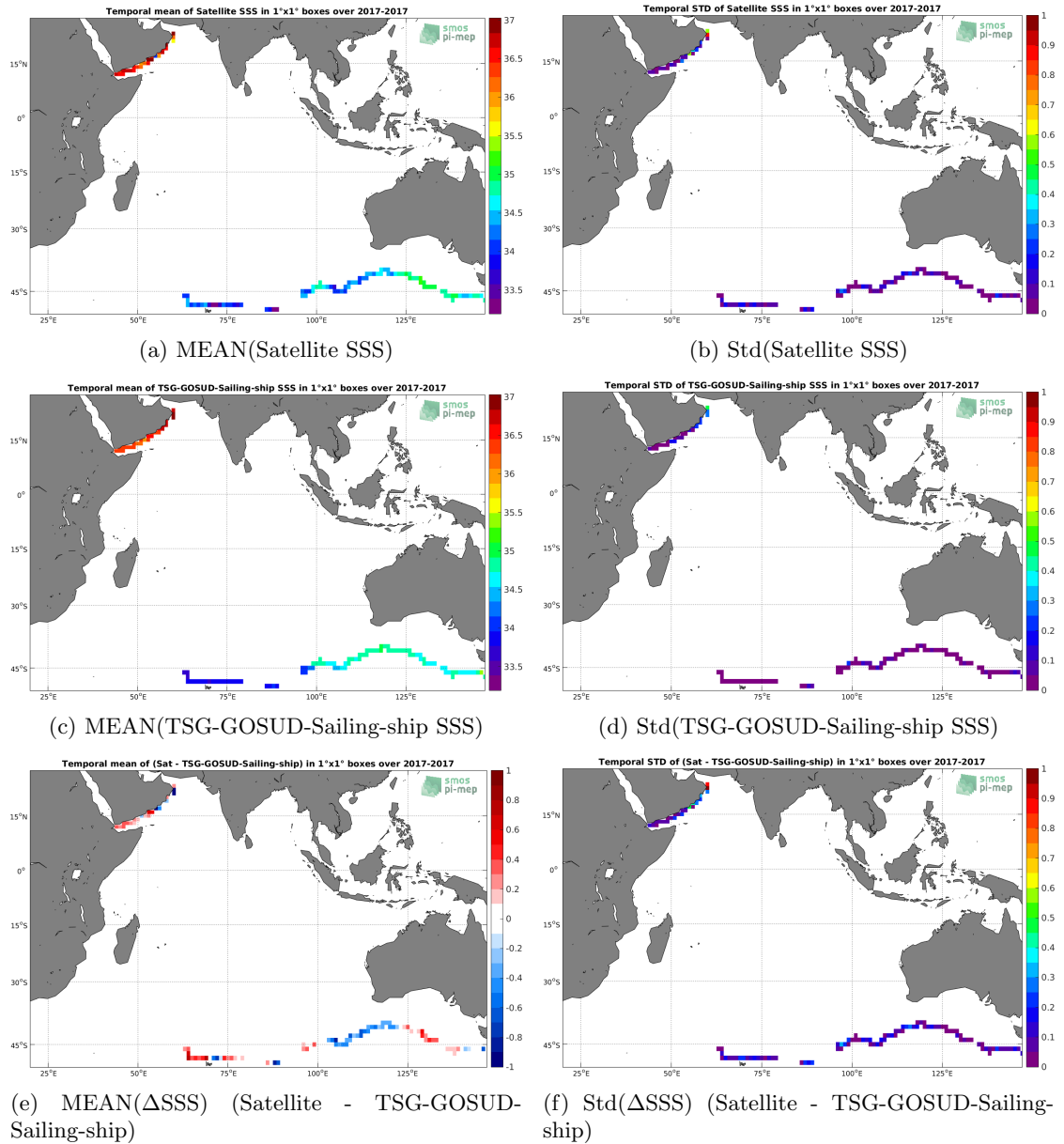
Figure 6: Temporal mean (left) and Std (right) of SSS from SMAP-L3-JPL-V4.3-8DAY-RUNNING-60KM (top), TSG-GOSUD-Sailing-ship (middle), and of \Delta SSS (Satellite - TSG-GOSUD-Sailing-ship). Only match-up pairs are used to generate these maps.
