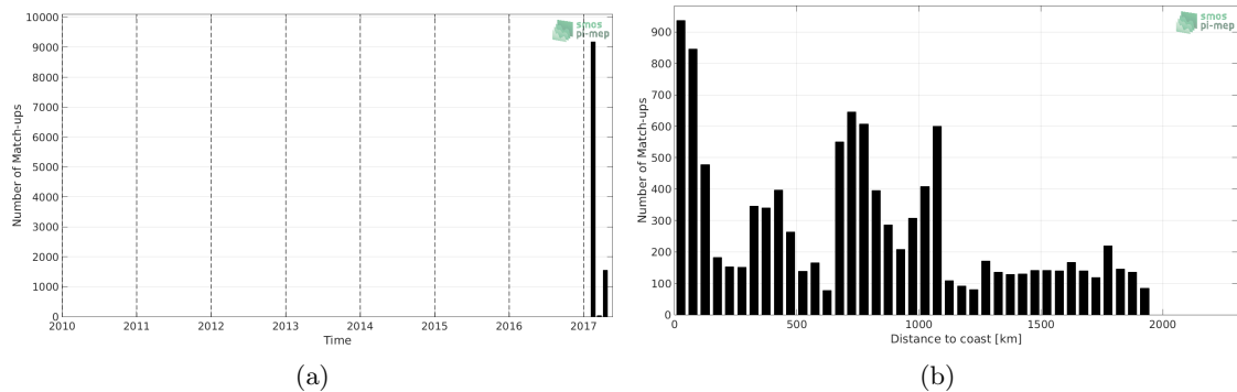
Figure 1: Number of match-ups between TSG-GOSUD-Sailing-ship and SMAP-L3-JPL-V4.3-8DAY-RUNNING-60KM SSS as a function of time (a) and as function of the distance to coast (b) over the Indian Ocean Pi-MEP region and for the full satellite product period.
