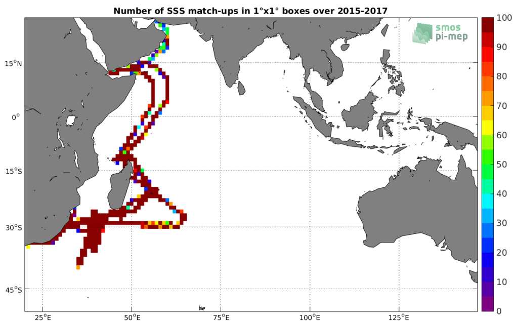
Figure 4: Number of SSS match-ups between TSG-GOSUD-Research-vessel SSS and the SMAP-L3-JPL-V4.3-8DAY-RUNNING-60KM SSS product for the Indian Ocean Pi-MEP region over 1°x1° boxes and for the full satellite product period.
