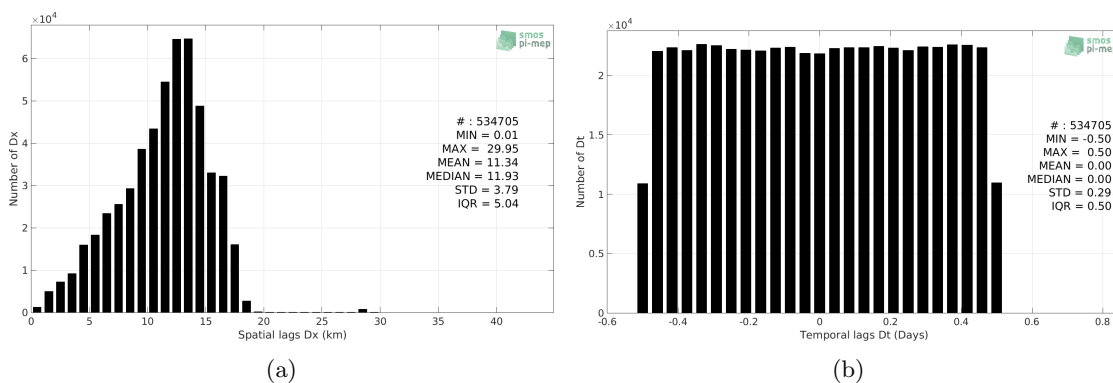
Figure 5: Histograms of the spatial (a) and temporal (b) lags between the time of the TSG-GOSUD-Research-vessel measurements and the date of the corresponding SMAP-L3-JPL-V4.3-8DAY-RUNNING-60KM SSS product.
