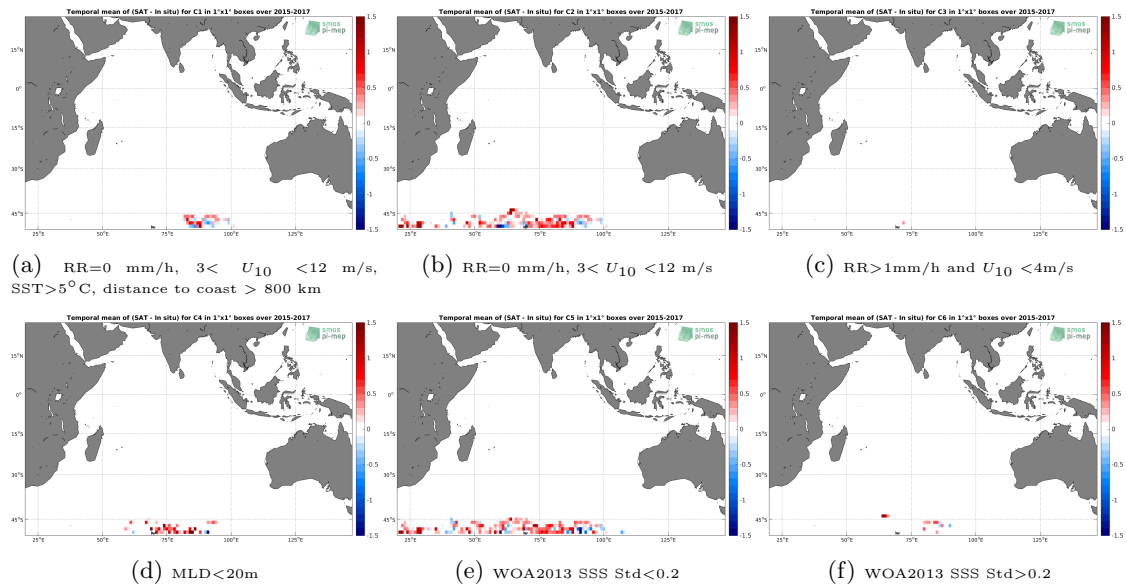
Figure 12: Temporal mean gridded over spatial boxes of size 1^{\circ}\times 1^{\circ} of \Delta\text{SSS} (SMAP-L3-JPL-V4.3-8DAY-RUNNING-60KM - Sea mammals) for 6 different subdatasets corresponding to:RR=0 mm/h, 3 < U_{10} < 12 m/s, SST >5^{\circ}\text{C} , distance to coast > 800 km (a), RR=0 mm/h, 3 < U_{10} < 12 m/s (b), RR >1 mm/h and U_{10} < 4 m/s (c),MLD <20 m (d),WOA2013 SSS Std <0.2 (e),WOA2013 SSS Std >0.2 (f).
