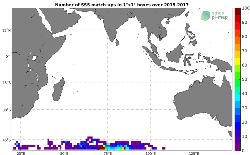
Figure 4: Number of SSS match-ups between Sea mammals SSS and the SMAP-L3-JPL-V4.3-8DAY-RUNNING-60KM SSS product for the Indian Ocean Pi-MEP region over 1°x1° boxes and for the full satellite product period.
