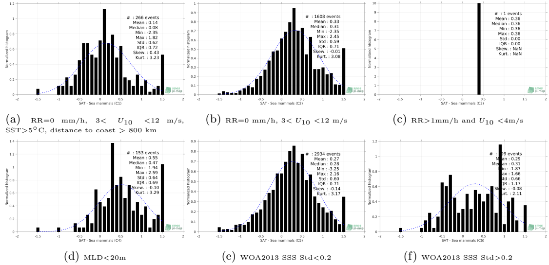
Figure 13: Normalized histogram of \Delta SSS (SMAP-L3-JPL-V4.3-8DAY-RUNNING-60KM - Sea mammals) for 6 different subdatasets corresponding to: RR=0 mm/h, 3 < U_{10} < 12 m/s, SST>5°C, distance to coast > 800 km (a), RR=0 mm/h, 3 < U_{10} < 12 m/s (b), RR>1mm/h and U_{10} < 4 m/s (c), MLD<20m (d), WOA2013 SSS Std<0.2 (e), WOA2013 SSS Std>0.2 (f).
