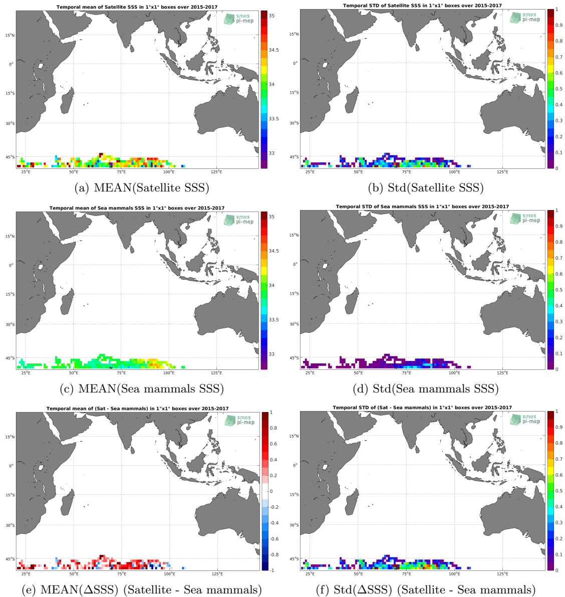
Figure 6: Temporal mean (left) and Std (right) of SSS from SMAP-L3-JPL-V4.3-8DAY-RUNNING-60KM (top), Sea mammals (middle), and of \Delta SSS (Satellite - Sea mammals). Only match-up pairs are used to generate these maps.
