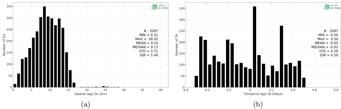
Figure 5: Histograms of the spatial (a) and temporal (b) lags between the time of the Sea mammals measurements and the date of the corresponding SMAP-L3-JPL-V4.3-8DAY-RUNNING-60KM SSS product.
