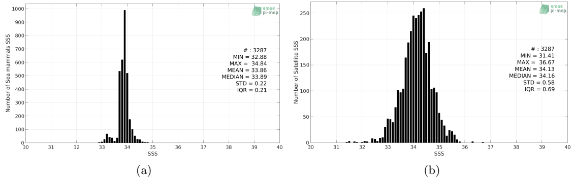
Figure 2: Histograms of SSS from Sea mammals (a) and SMAP-L3-JPL-V4.3-8DAY-RUNNING-60KM (b) considering all match-up pairs per bins of 0.1 over the Indian Ocean Pi-MEP region and for the full satellite product period.
