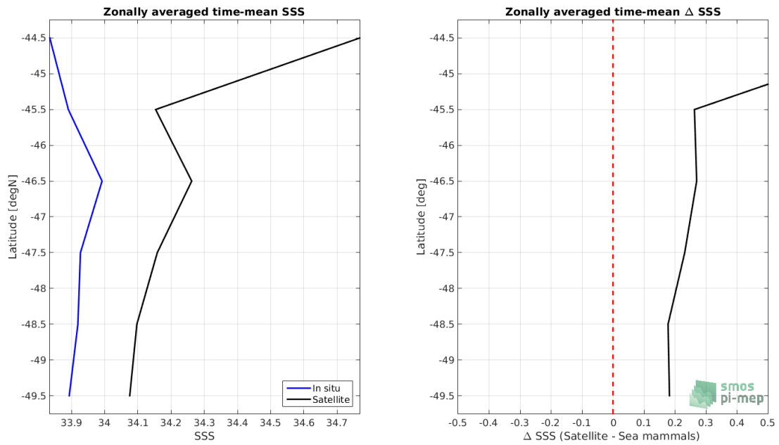
Figure 8: Left panel: Zonal mean SSS from SMAP-L3-JPL-V4.3-8DAY-RUNNING-60KM satellite product (black) and from Sea mammals (blue). Right panel: Zonal mean of \Delta SSS (Satellite - Sea mammals) for all the collected Pi-MEP match-up pairs estimated over the full satellite product period.
