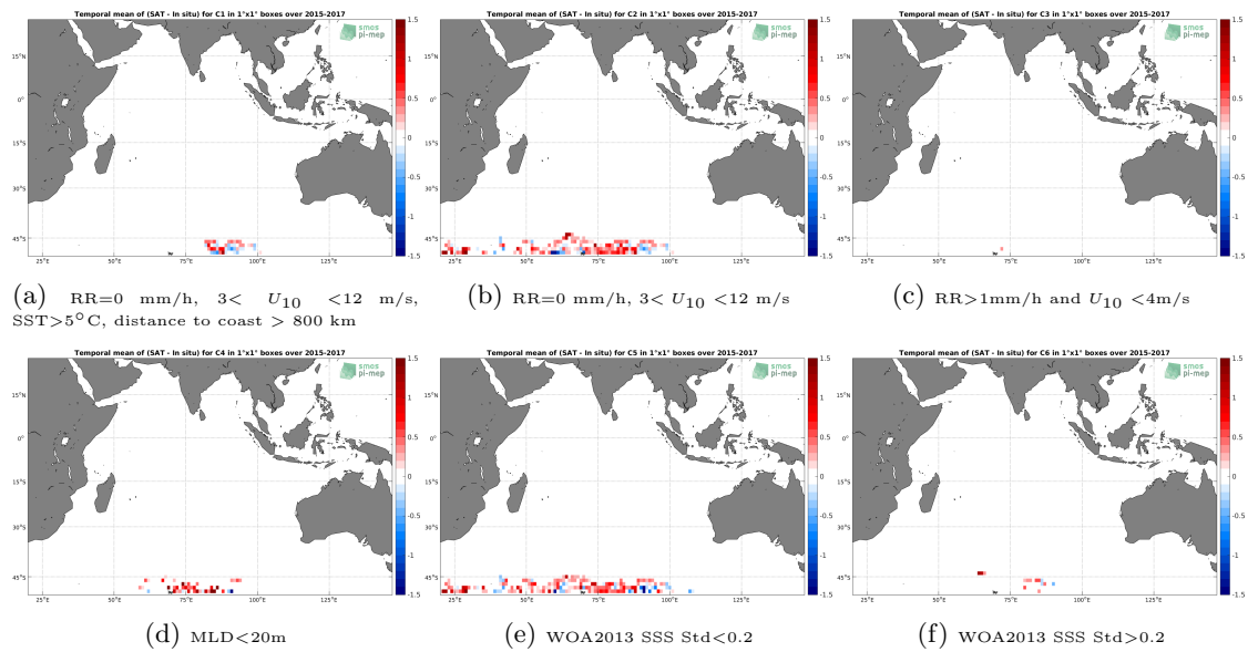
Figure 12: Temporal mean gridded over spatial boxes of size 1^\circ \times 1^\circ of \Delta SSS (SMAP-L3-JPL-V4.3-8DAY-RUNNING-60KM - Sea mammals) for 6 different subdatasets corresponding to:RR=0 mm/h, 3 < U_{10} < 12 m/s, SST >5^\circ C, distance to coast > 800 km (a), RR=0 mm/h, 3 < U_{10} < 12 m/s (b), RR >1 mm/h and U_{10} < 4 m/s (c),MLD <20 m (d),WOA2013 SSS Std <0.2 (e),WOA2013 SSS Std >0.2 (f).
