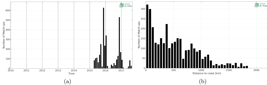
Figure 1: Number of match-ups between Sea mammals and SMAP-L3-JPL-V4.3-8DAY-RUNNING-60KM SSS as a function of time (a) and as function of the distance to coast (b) over the Indian Ocean Pi-MEP region and for the full satellite product period.
