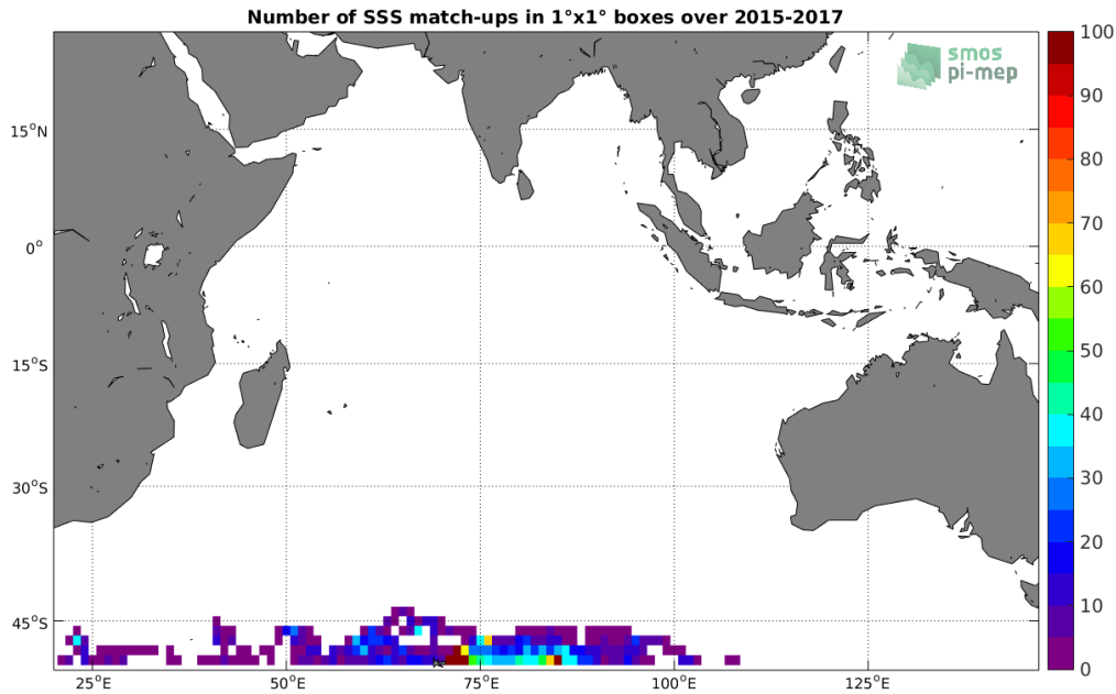
Figure 4: Number of SSS match-ups between Sea mammals SSS and the SMAP-L3-JPL-V4.3-8DAY-RUNNING-60KM SSS product for the Indian Ocean Pi-MEP region over 1°x1° boxes and for the full satellite product period.
