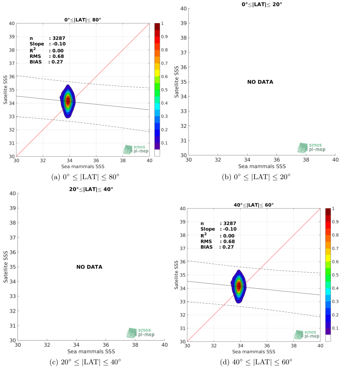
Figure 9: Contour maps of the concentration of SMAP-L3-JPL-V4.3-8DAY-RUNNING-60KM SSS (y-axis) versus Sea mammals SSS (x-axis) at match-up pairs for different latitude bands. For each plot, the red line shows x=y . The black thin and dashed lines indicate a linear fit through the data cloud and the \pm 95\% confidence levels, respectively. The number match-up pairs n , the slope and R^2 coefficient of the linear fit, the root mean square (RMS) and the mean bias between satellite and in situ data are indicated for each latitude band in each plots.
