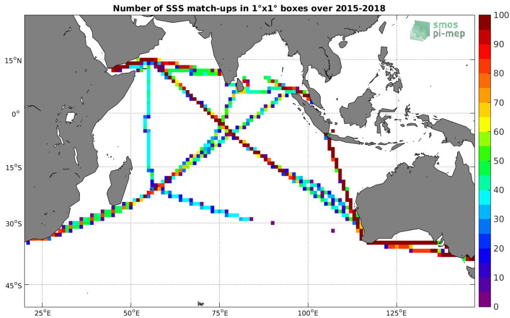
Figure 4: Number of SSS match-ups between TSG-LEGOS-DM SSS and the SMAP-L3-JPL-V4.3-MONTHLY-60KM SSS product for the Indian Ocean Pi-MEP region over 1^\circ \times 1^\circ boxes and for the full satellite product period.
