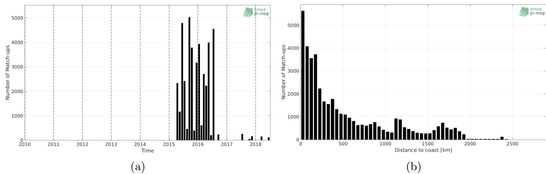
Figure 1: Number of match-ups between TSG-LEGOS-DM and SMAP-L3-JPL-V4.3-MONTHLY-60KM SSS as a function of time (a) and as function of the distance to coast (b) over the Indian Ocean Pi-MEP region and for the full satellite product period.
