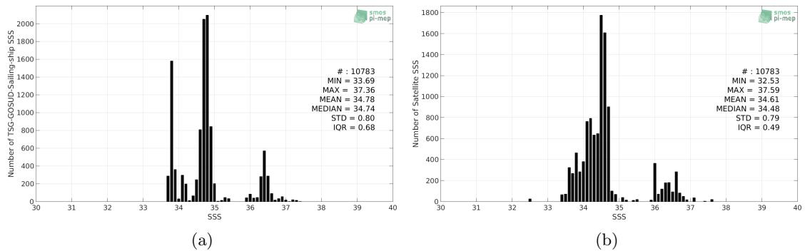
Figure 2: Histograms of SSS from TSG-GOSUD-Sailing-ship (a) and SMAP-L3-JPL-V4.3-MONTHLY-60KM (b) considering all match-up pairs per bins of 0.1 over the Indian Ocean Pi-MEP region and for the full satellite product period.
