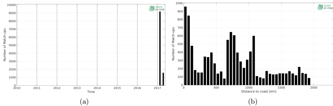
Figure 1: Number of match-ups between TSG-GOSUD-Sailing-ship and SMAP-L3-JPL-V4.3-MONTHLY-60KM SSS as a function of time (a) and as function of the distance to coast (b) over the Indian Ocean Pi-MEP region and for the full satellite product period.
