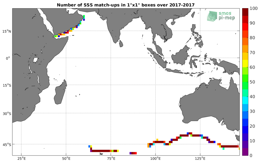
Figure 4: Number of SSS match-ups between TSG-GOSUD-Sailing-ship SSS and the SMAP-L3-JPL-V4.3-MONTHLY-60KM SSS product for the Indian Ocean Pi-MEP region over 1°x1° boxes and for the full satellite product period.
