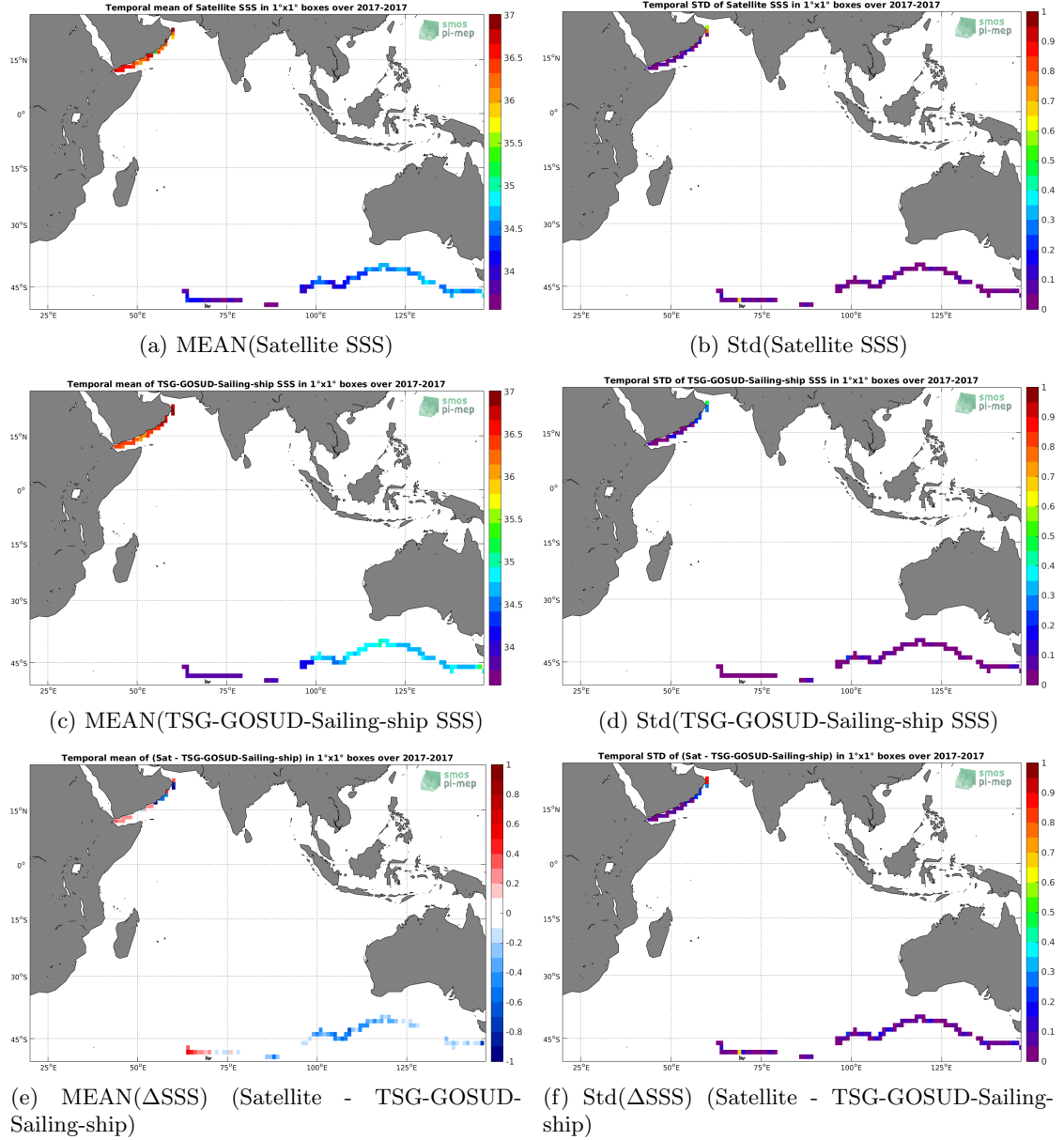
Figure 6: Temporal mean (left) and Std (right) of SSS from SMAP-L3-JPL-V4.3-MONTHLY-60KM (top), TSG-GOSUD-Sailing-ship (middle), and of \Delta SSS (Satellite - TSG-GOSUD-Sailing-ship). Only match-up pairs are used to generate these maps.
