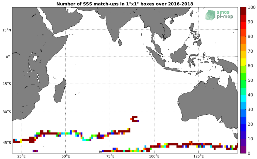
Figure 3: Number of SSS match-ups between Surface drifters SSS and the SMAP-L3-JPL-V4.3-MONTHLY-60KM SSS product for the Indian Ocean Pi-MEP region over 1°x1° boxes and for the full satellite product period.
