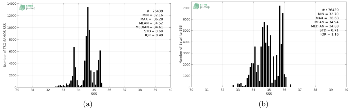
Figure 2: Histograms of SSS from TSG-SAMOS (a) and SMAP-L3-JPL-V4-8DAY-RUNNING-60KM (b) considering all match-up pairs per bins of 0.1 over the Indian Ocean Pi-MEP region and for the full satellite product period.
