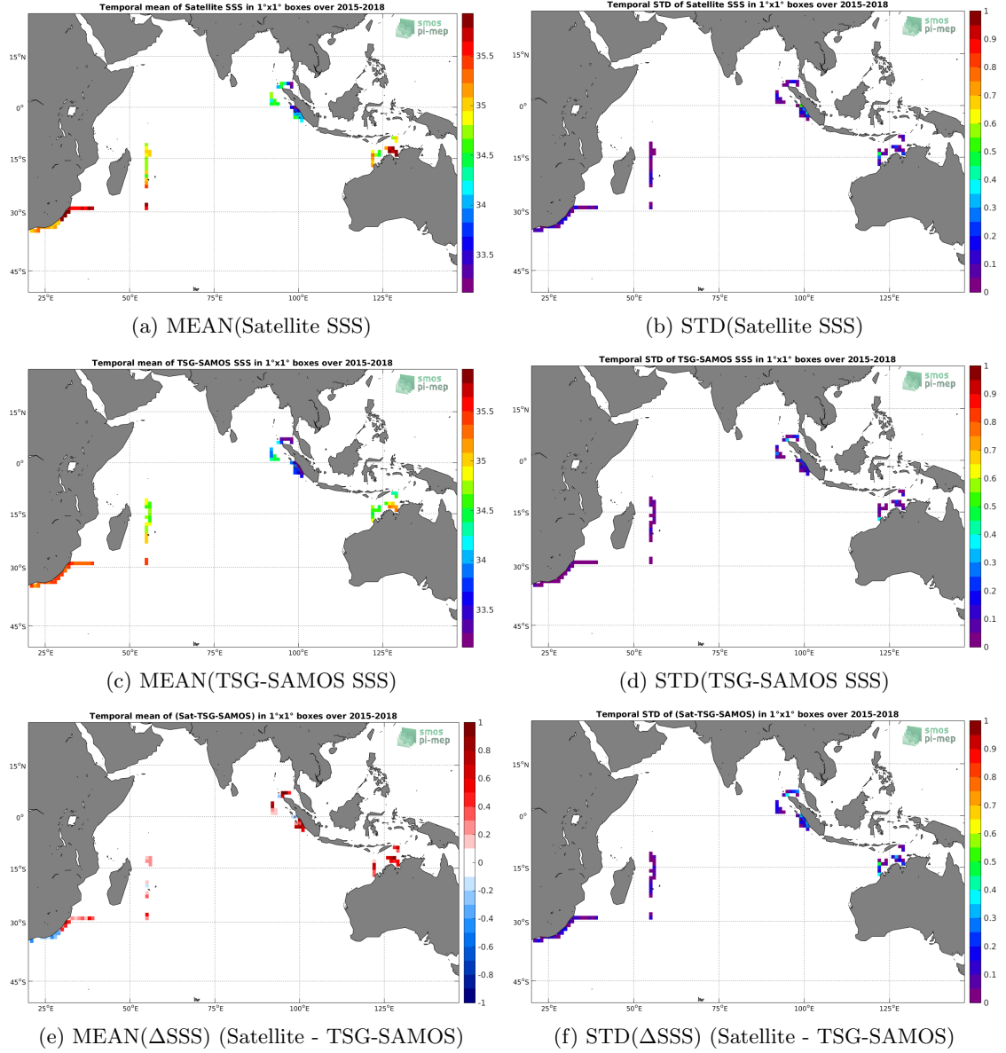
Figure 6: Temporal mean (left) and STD (right) of SSS from SMAP-L3-JPL-V4-8DAY-RUNNING-60KM (top), TSG-SAMOS (middle), and of \Delta SSS (Satellite - TSG-SAMOS). Only match-up pairs are used to generate these maps.
