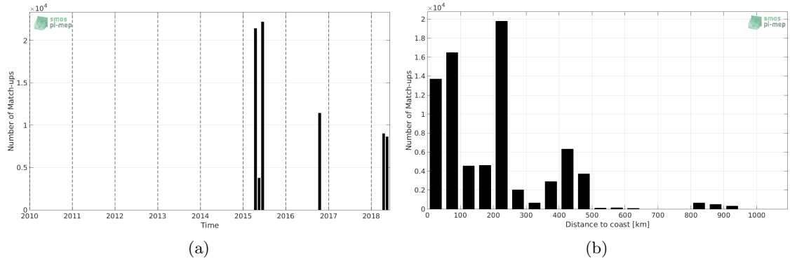
Figure 1: Number of match-ups between TSG-SAMOS and SMAP-L3-JPL-V4-8DAY-RUNNING-60KM SSS as a function of time (a) and as function of the distance to coast (b) over the Indian Ocean Pi-MEP region and for the full satellite product period.
