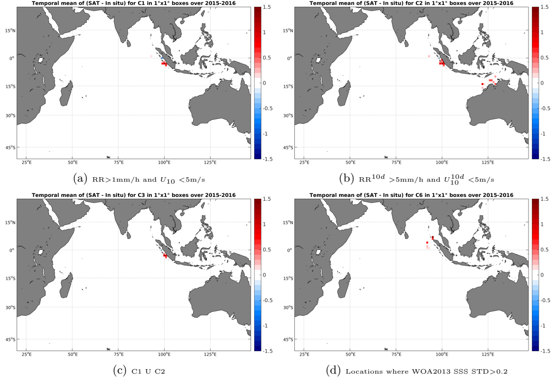
Figure 12: Temporal mean gridded over spatial boxes of size 1^\circ \times 1^\circ of \Delta SSS (SMAP-L3-JPL-V4-8DAY-RUNNING-60KM - TSG-SAMOS) for 4 different subdatasets corresponding to: RR > 1 mm/h and U_{10} < 5 m/s (a), RR^{10d} > 5 mm/h and U_{10}^{10d} < 5 m/s (b), C1 U C2 (c), Locations where WOA2013 SSS STD > 0.2 (d).
