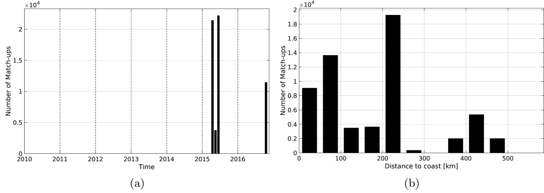
Figure 1: Number of match-ups between TSG-SAMOS and SMAP-L3-JPL-V4-8DAY-RUNNING-60KM SSS as a function of time (a) and as function of the distance to coast (b) over the Indian Ocean Pi-MEP region and for the full satellite product period.
