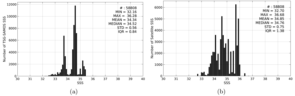
Figure 2: Histograms of SSS from TSG-SAMOS (a) and SMAP-L3-JPL-V4-8DAY-RUNNING-60KM (b) considering all match-up pairs per bins of 0.1 over the Indian Ocean Pi-MEP region and for the full satellite product period.
