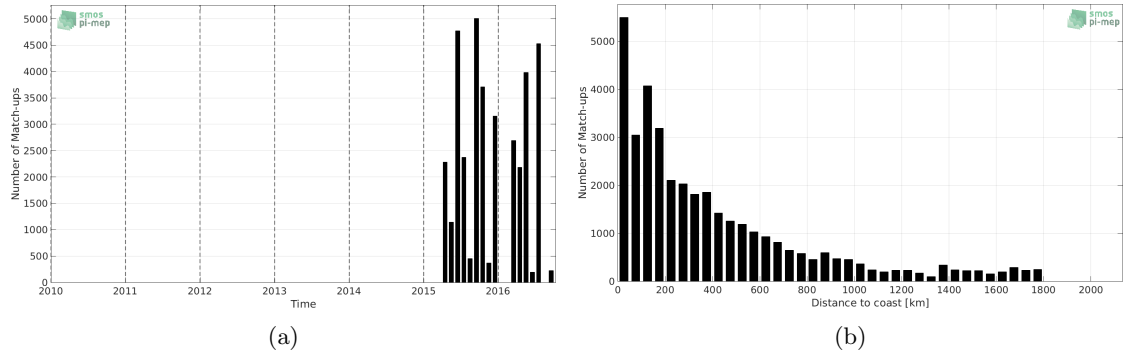
Figure 1: Number of match-ups between TSG-LEGOS-DM and SMAP-L3-JPL-V4-8DAY-RUNNING-60KM SSS as a function of time (a) and as function of the distance to coast (b) over the Indian Ocean Pi-MEP region and for the full satellite product period.
