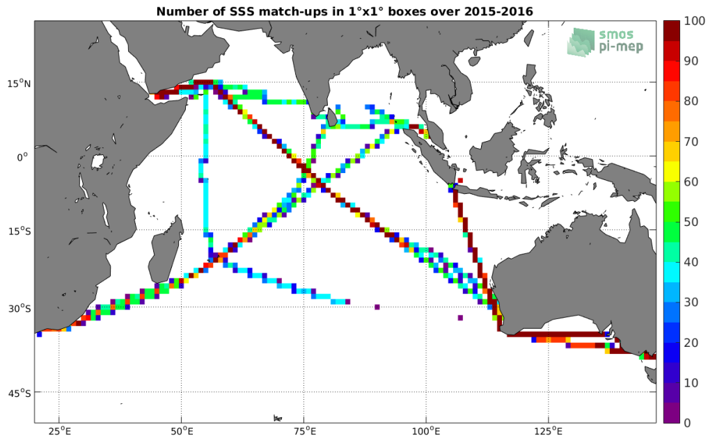
Figure 4: Number of SSS match-ups between TSG-LEGOS-DM SSS and the SMAP-L3-JPL-V4-8DAY-RUNNING-60KM SSS product for the Indian Ocean Pi-MEP region over 1^\circ \times 1^\circ boxes and for the full satellite product period.
