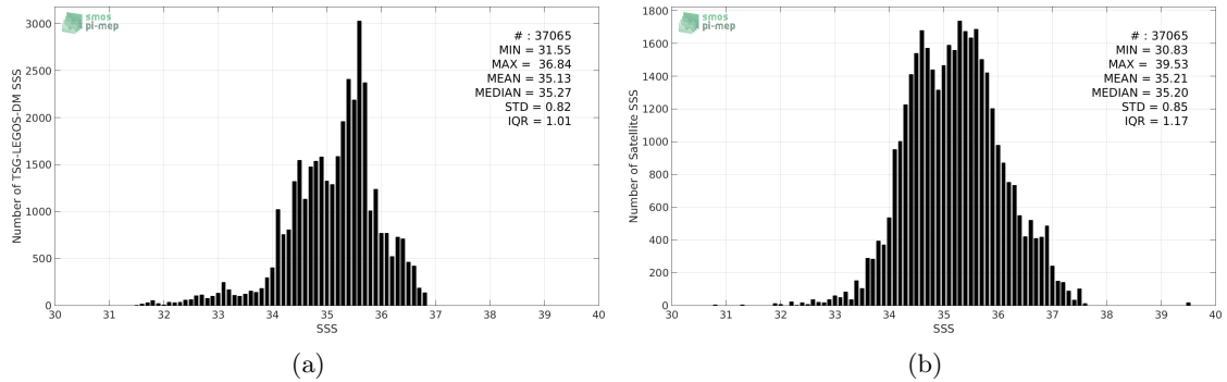
Figure 2: Histograms of SSS from TSG-LEGOS-DM (a) and SMAP-L3-JPL-V4-8DAY-RUNNING-60KM (b) considering all match-up pairs per bins of 0.1 over the Indian Ocean Pi-MEP region and for the full satellite product period.
