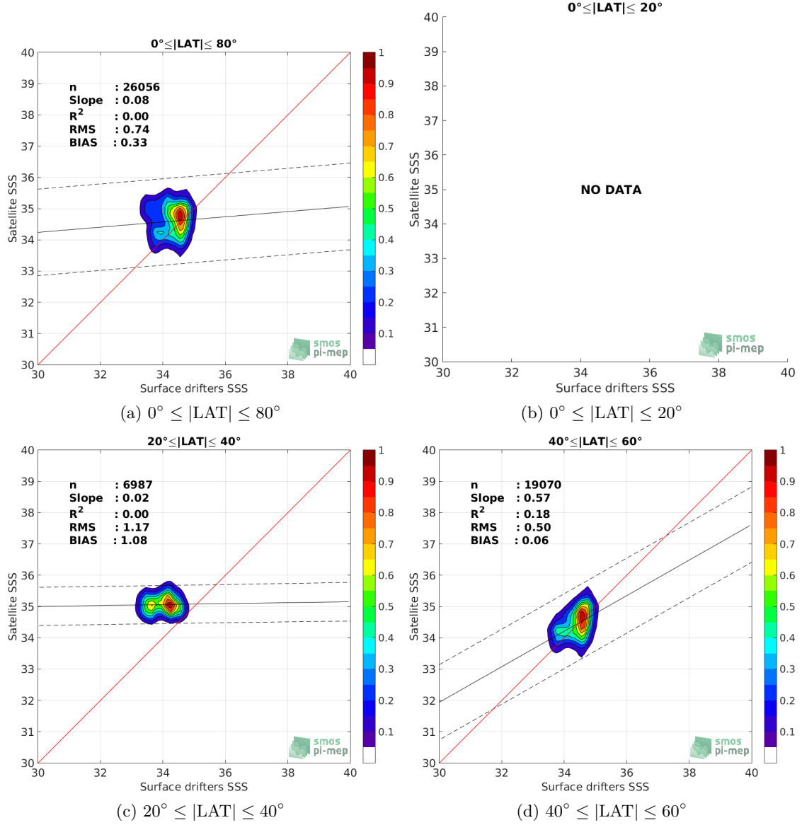
Figure 8: Contour maps of the concentration of SMAP-L3-JPL-V4-8DAY-RUNNING-60KM SSS (y-axis) versus Surface drifters SSS (x-axis) at match-up pairs for different latitudinal bands. For each plot, the red line shows x=y . The black thin and dashed lines indicate a linear fit through the data cloud and the \pm 95\% confidence levels, respectively. The number match-up pairs n , the slope and R^2 coefficient of the linear fit, the root mean square (RMS) and the mean bias between satellite and in situ data are indicated for each latitude band in each plots.
