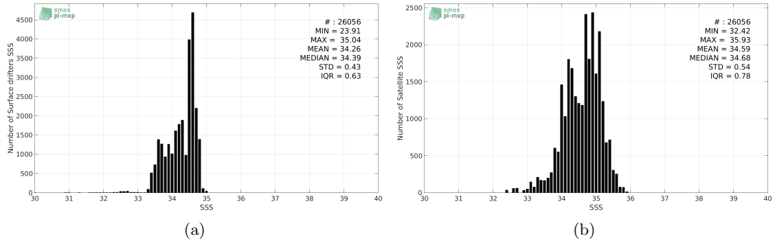
Figure 2: Histograms of SSS from Surface drifters (a) and SMAP-L3-JPL-V4-8DAY-RUNNING-60KM (b) considering all match-up pairs per bins of 0.1 over the Indian Ocean Pi-MEP region and for the full satellite product period.
