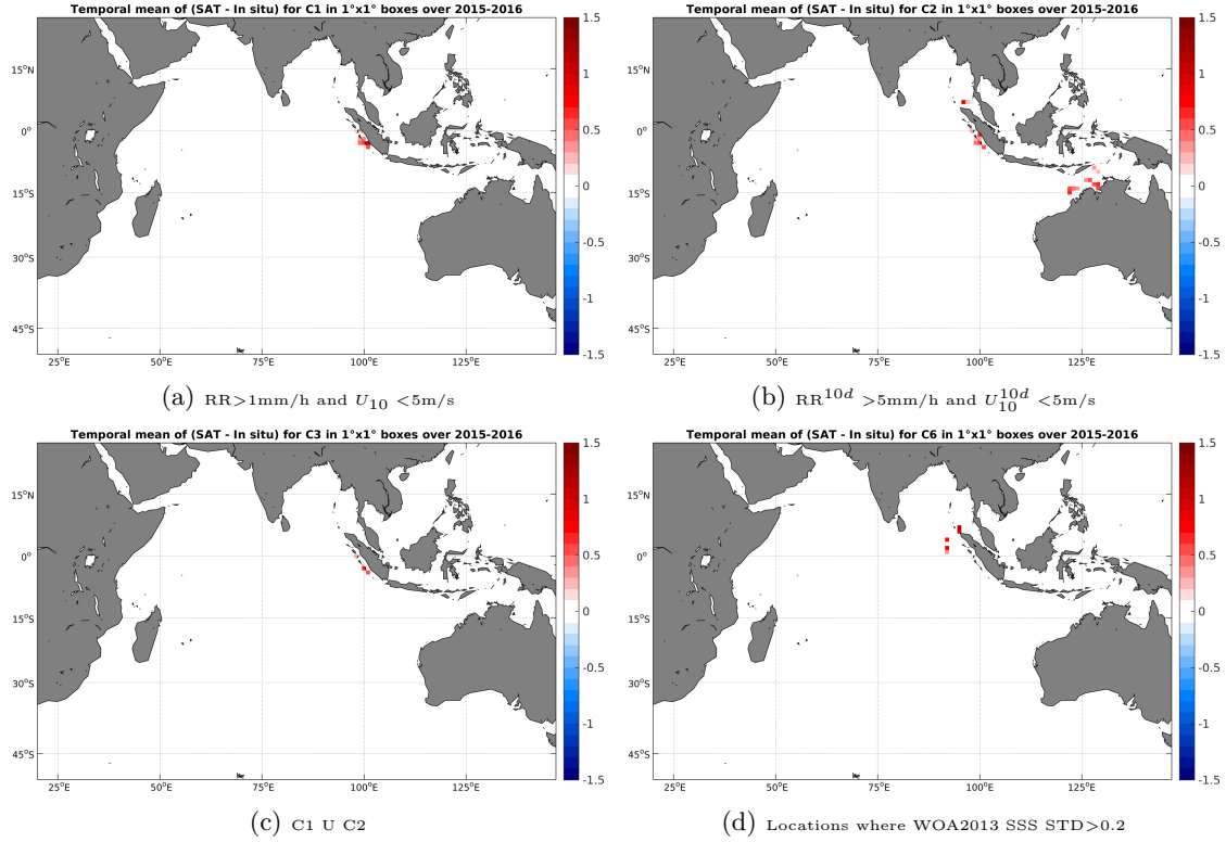
Figure 12: Temporal mean gridded over spatial boxes of size 1^\circ \times 1^\circ of \Delta SSS (SMAP-L3-JPL-V4-MONTHLY-60KM - TSG-SAMOS) for 4 different subdatasets corresponding to: RR > 1 mm/h and U_{10} < 5 m/s (a), RR^{10d} > 5 mm/h and U_{10}^{10d} < 5 m/s (b), C1 U C2 (c), Locations where WOA2013 SSS STD > 0.2 (d).
