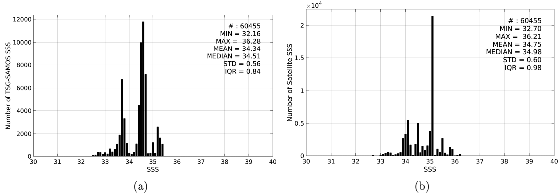
Figure 2: Histograms of SSS from TSG-SAMOS (a) and SMAP-L3-JPL-V4-MONTHLY-60KM (b) considering all match-up pairs per bins of 0.1 over the Indian Ocean Pi-MEP region and for the full satellite product period.
