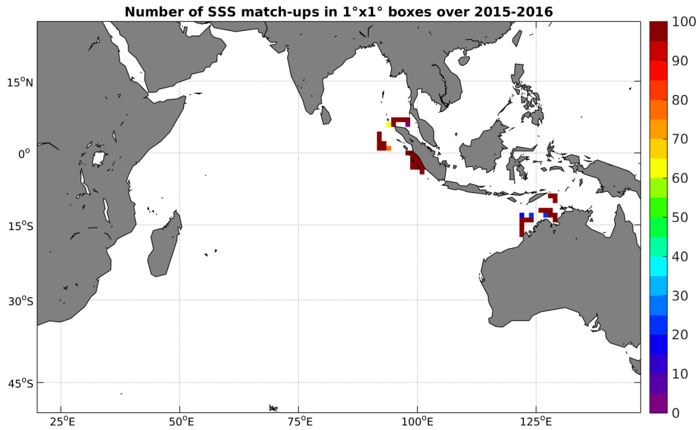
Figure 4: Number of SSS match-ups between TSG-SAMOS SSS and the SMAP-L3-JPL-V4-MONTHLY-60KM SSS product for the Indian Ocean Pi-MEP region over 1^\circ \times 1^\circ boxes and for the full satellite product period.
