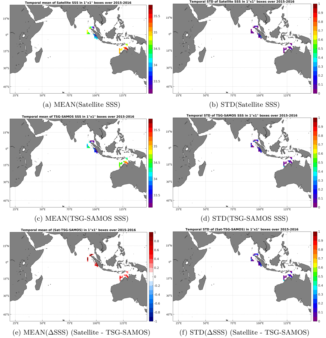
Figure 6: Temporal mean (left) and STD (right) of SSS from SMAP-L3-JPL-V4-MONTHLY-60KM (top), TSG-SAMOS (middle), and of \Delta SSS (Satellite - TSG-SAMOS). Only match-up pairs are used to generate these maps.
