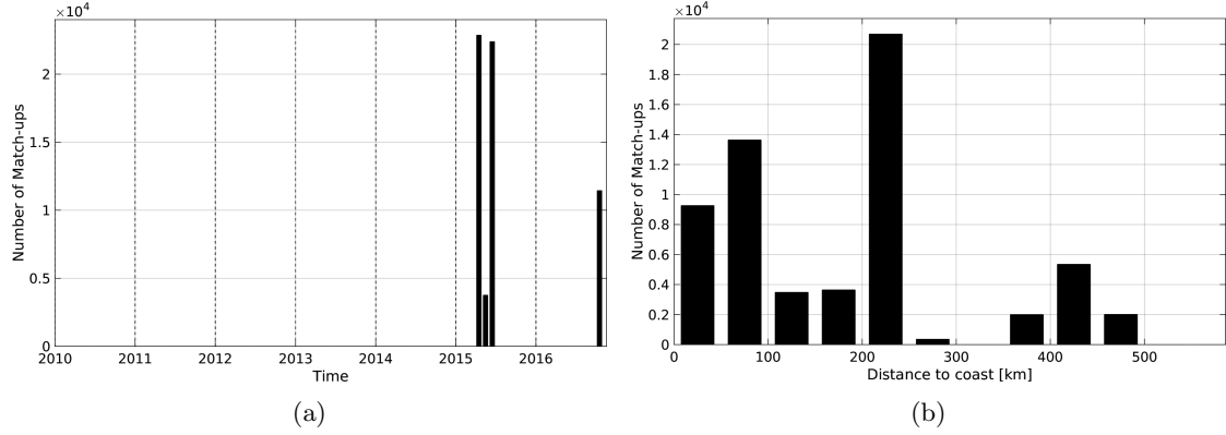
Figure 1: Number of match-ups between TSG-SAMOS and SMAP-L3-JPL-V4-MONTHLY-60KM SSS as a function of time (a) and as function of the distance to coast (b) over the Indian Ocean Pi-MEP region and for the full satellite product period.
