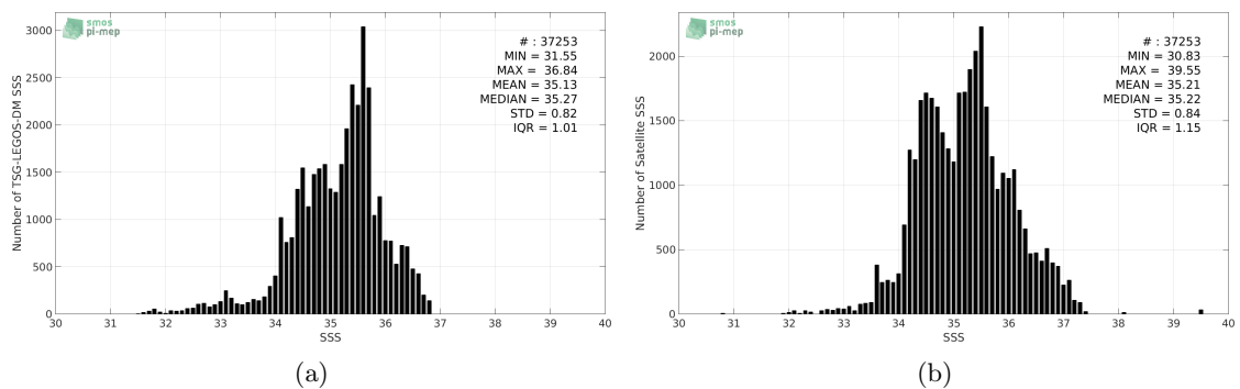
Figure 2: Histograms of SSS from TSG-LEGOS-DM (a) and SMAP-L3-JPL-V4-MONTHLY-60KM (b) considering all match-up pairs per bins of 0.1 over the Indian Ocean Pi-MEP region and for the full satellite product period.
