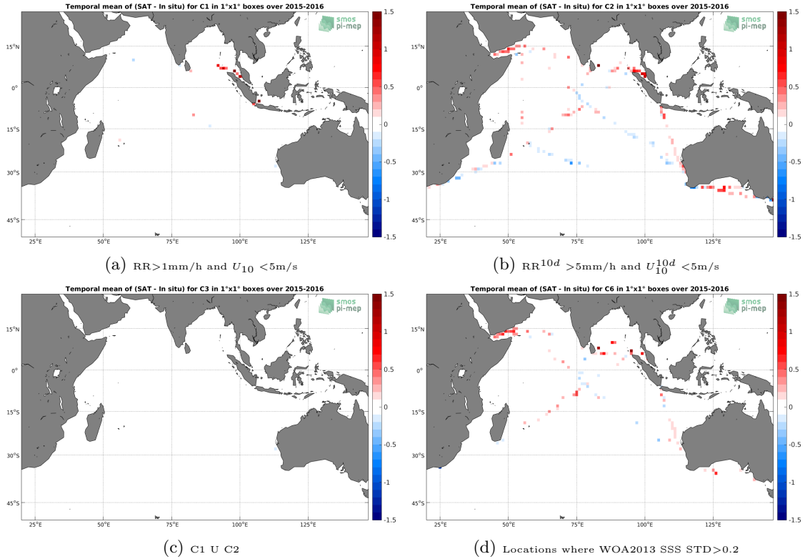
Figure 12: Temporal mean gridded over spatial boxes of size 1^\circ \times 1^\circ of \Delta SSS (SMAP-L3-JPL-V4-MONTHLY-60KM - TSG-LEGOS-DM) for 4 different subdatasets corresponding to: RR > 1mm/h and U_{10} < 5\text{m/s} (a), RR^{10d} > 5\text{mm/h} and U_{10}^{10d} < 5\text{m/s} (b), C1 U C2 (c), Locations where WOA2013 SSS STD > 0.2 (d).
