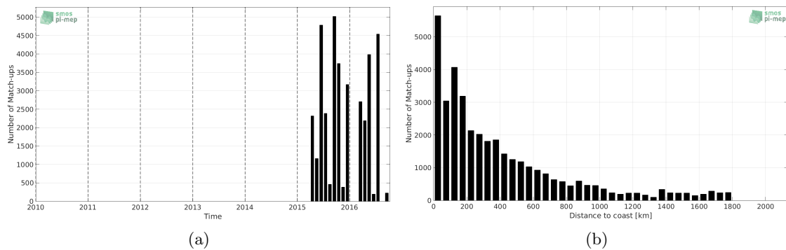
Figure 1: Number of match-ups between TSG-LEGOS-DM and SMAP-L3-JPL-V4-MONTHLY-60KM SSS as a function of time (a) and as function of the distance to coast (b) over the Indian Ocean Pi-MEP region and for the full satellite product period.
