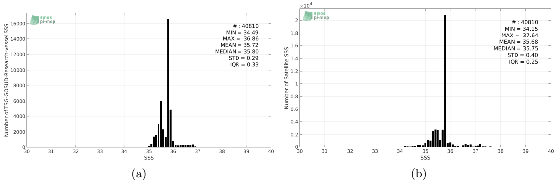
Figure 2: Histograms of SSS from TSG-GOSUD-Research-vessel (a) and SMAP-L3-JPL-V4-MONTHLY-60KM (b) considering all match-up pairs per bins of 0.1 over the Indian Ocean Pi-MEP region and for the full satellite product period.
