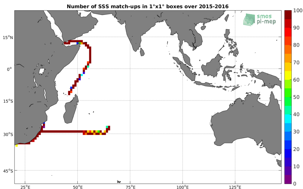
Figure 4: Number of SSS match-ups between TSG-GOSUD-Research-vessel SSS and the SMAP-L3-JPL-V4-MONTHLY-60KM SSS product for the Indian Ocean Pi-MEP region over 1°x1° boxes and for the full satellite product period.
