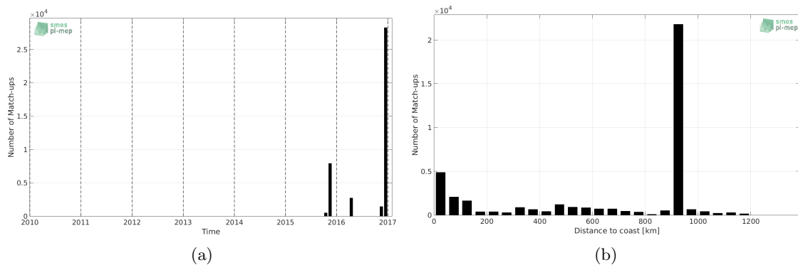
Figure 1: Number of match-ups between TSG-GOSUD-Research-vessel and SMAP-L3-JPL-V4-MONTHLY-60KM SSS as a function of time (a) and as function of the distance to coast (b) over the Indian Ocean Pi-MEP region and for the full satellite product period.
