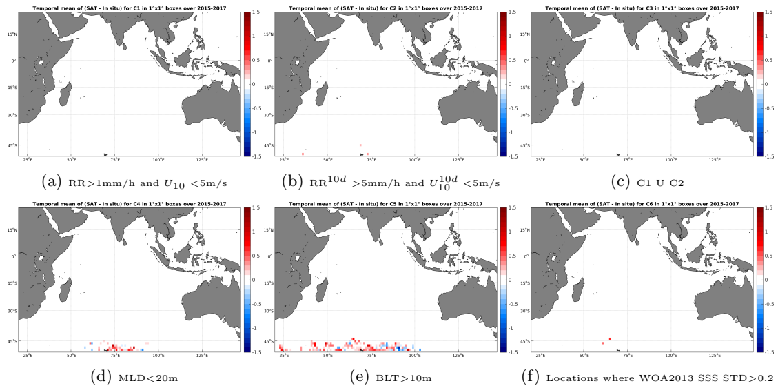
Figure 12: Temporal mean gridded over spatial boxes of size 1^\circ \times 1^\circ of \Delta SSS (SMAP-L3-JPL-V4-MONTHLY-60KM - Sea mammals) for 6 different subdatasets corresponding to: RR > 1\text{mm/h} and U_{10} < 5\text{m/s} (a), RR^{10d} > 5\text{mm/h} and U_{10}^{10d} < 5\text{m/s} (b), C1 U C2 (c), MLD < 20\text{m} (d), BLT > 10\text{m} (e), Locations where WOA2013 SSS STD > 0.2 (f).
