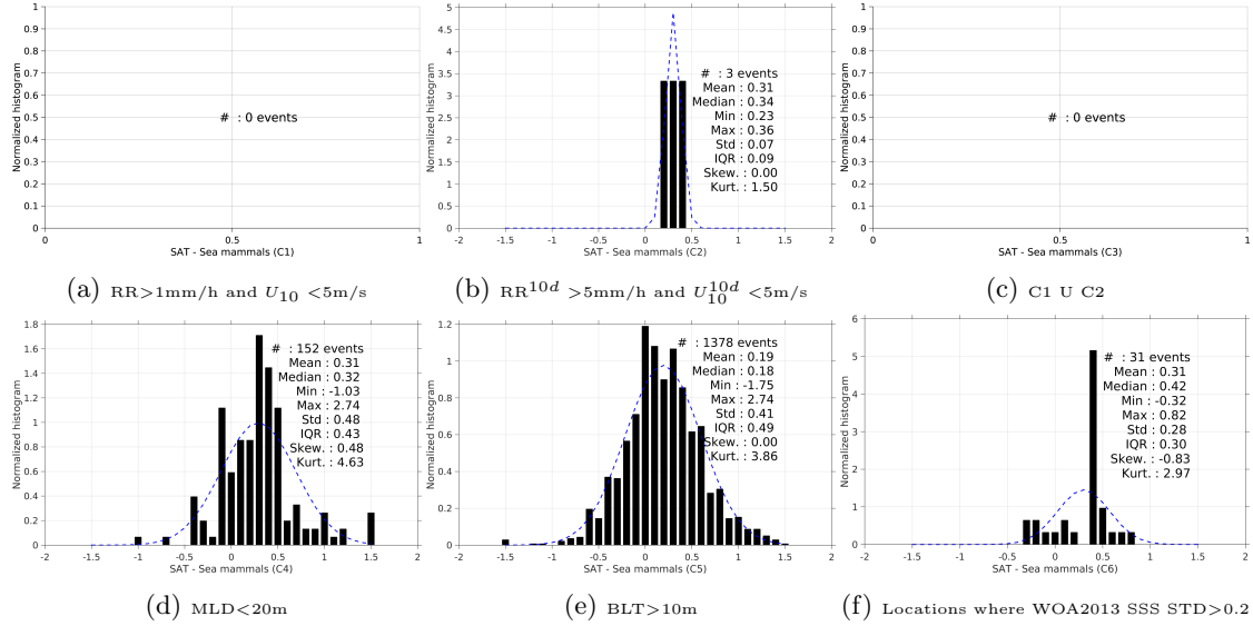
Figure 13: Normalized histogram of \Delta SSS (SMAP-L3-JPL-V4-MONTHLY-60KM - Sea mammals) for 6 different subdatasets corresponding to: RR>1mm/h and U_{10} < 5 m/s (a), RR 10d >5mm/h and U_{10}^{10d} < 5 m/s (b), C1 U C2 (c),MLD<20m (d),BLT>10m (e),Locations where WOA2013 SSS STD>0.2 (f).
