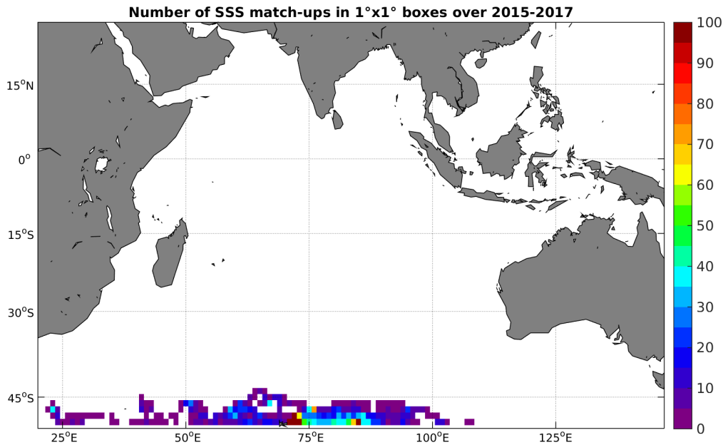
Figure 4: Number of SSS match-ups between Sea mammals SSS and the SMAP-L3-JPL-V4-MONTHLY-60KM SSS product for the Indian Ocean Pi-MEP region over 1^\circ \times 1^\circ boxes and for the full satellite product period.
