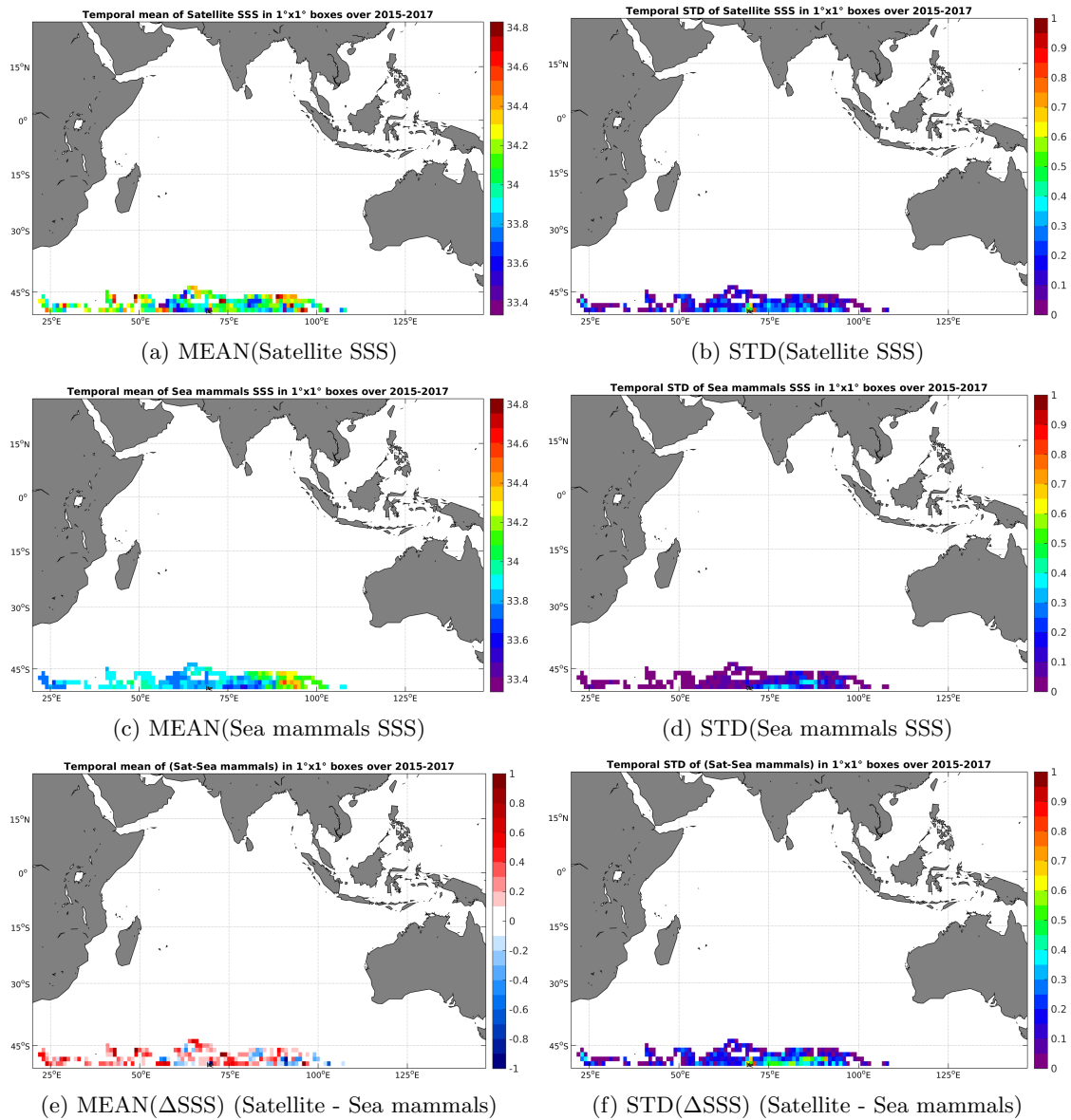
Figure 6: Temporal mean (left) and STD (right) of SSS from SMAP-L3-JPL-V4-MONTHLY-60KM (top), Sea mammals (middle), and of \Delta SSS (Satellite - Sea mammals). Only match-up pairs are used to generate these maps.
