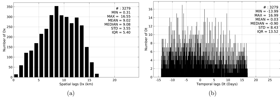
Figure 5: Histograms of the spatial (a) and temporal (b) lags between the time of the Sea mammals measurements and the date of the corresponding SMAP-L3-JPL-V4-MONTHLY-60KM SSS product.
