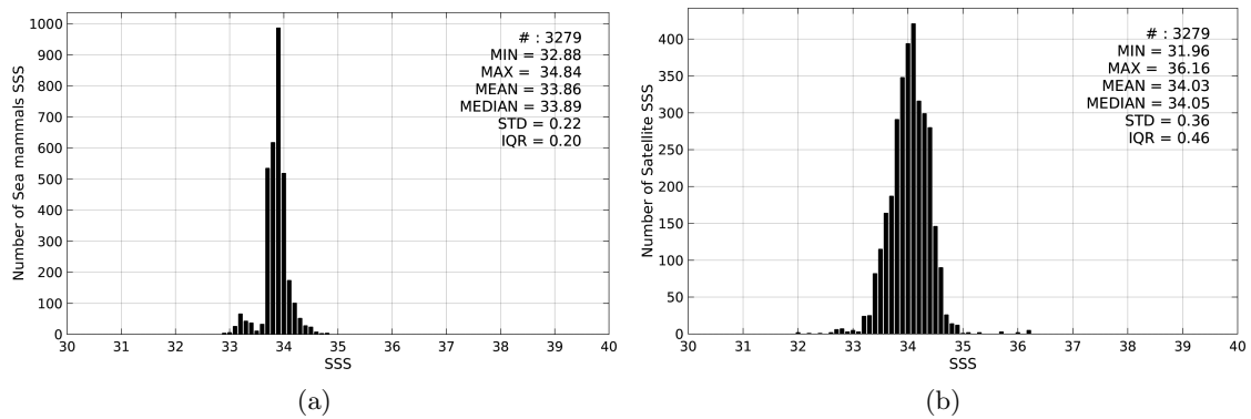
Figure 2: Histograms of SSS from Sea mammals (a) and SMAP-L3-JPL-V4-MONTHLY-60KM (b) considering all match-up pairs per bins of 0.1 over the Indian Ocean Pi-MEP region and for the full satellite product period.
