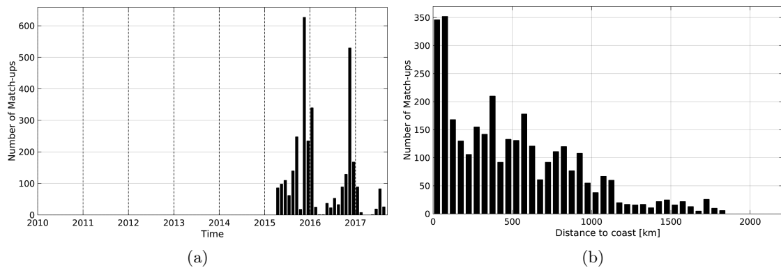
Figure 1: Number of match-ups between Sea mammals and SMAP-L3-JPL-V4-MONTHLY-60KM SSS as a function of time (a) and as function of the distance to coast (b) over the Indian Ocean Pi-MEP region and for the full satellite product period.
