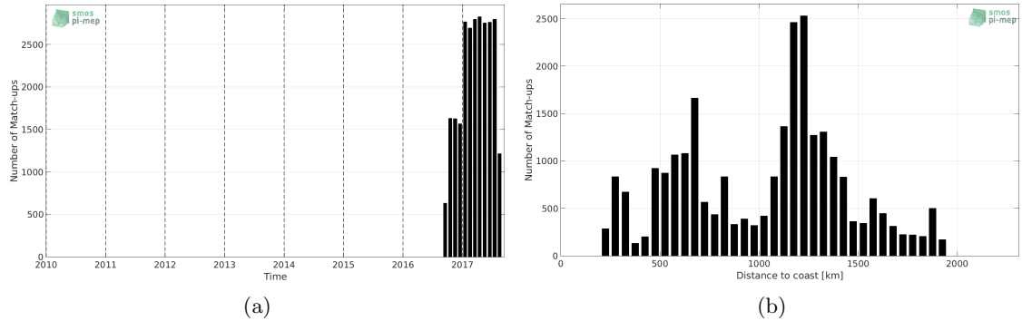
Figure 1: Number of match-ups between Surface drifters and SMAP-L3-JPL-V4-MONTHLY-60KM SSS as a function of time (a) and as function of the distance to coast (b) over the Indian Ocean Pi-MEP region and for the full satellite product period.
