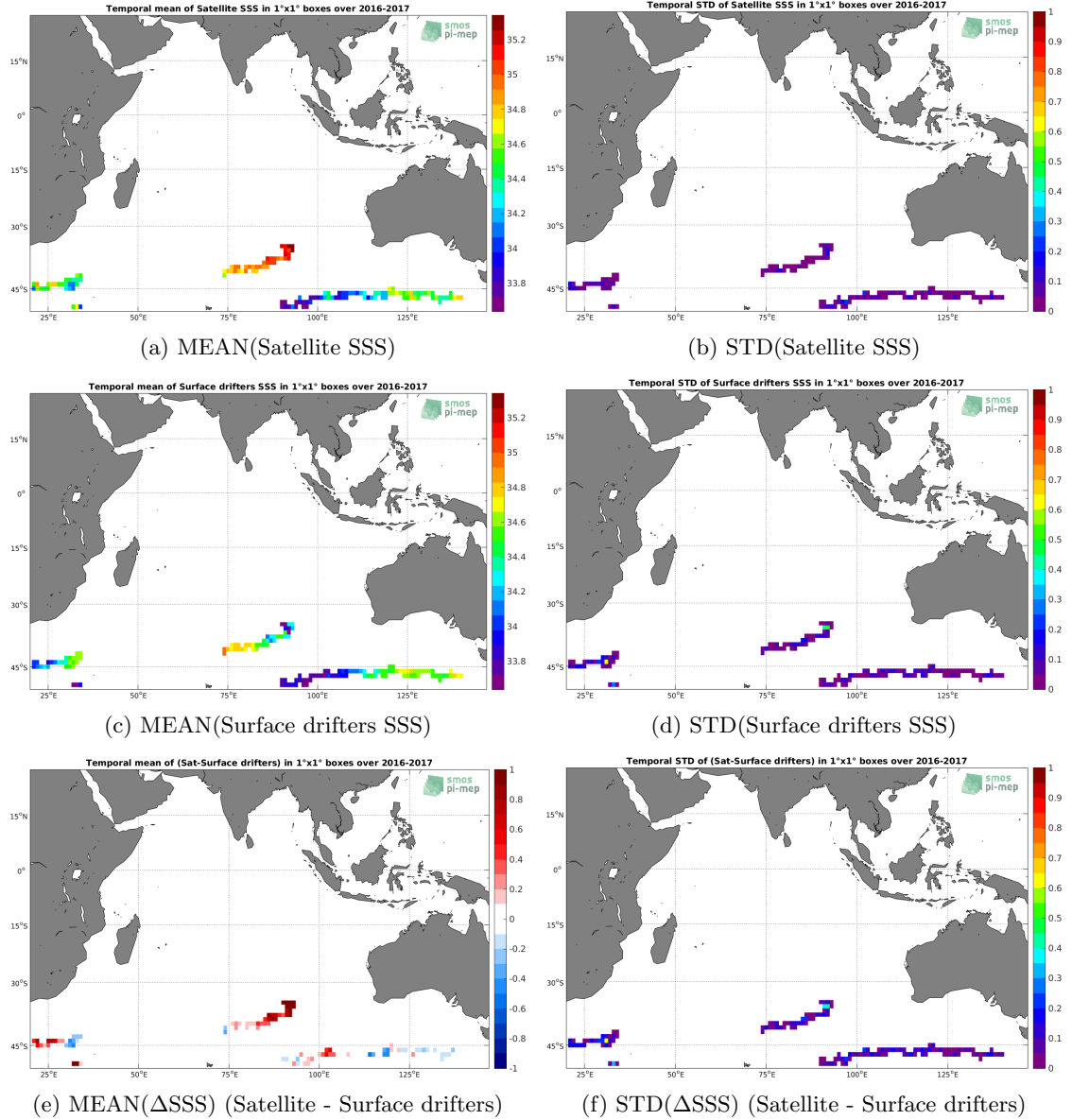
Figure 5: Temporal mean (left) and STD (right) of SSS from SMAP-L3-JPL-V4-MONTHLY-60KM (top), Surface drifters (middle), and of \Delta SSS (Satellite - Surface drifters). Only match-up pairs are used to generate these maps.
