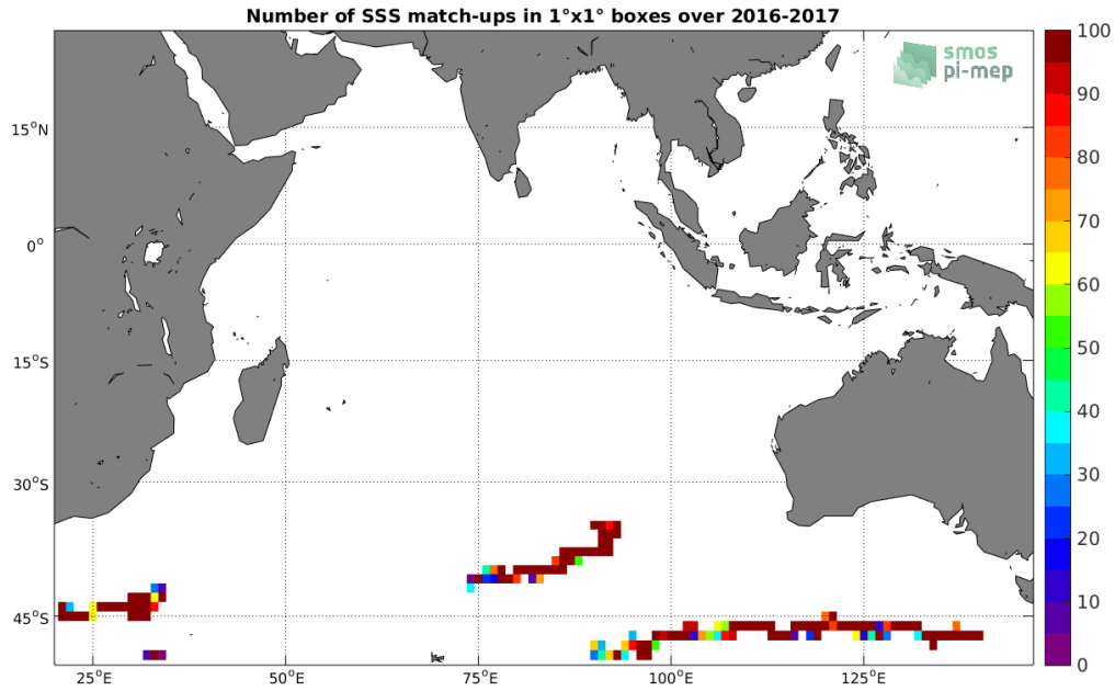
Figure 3: Number of SSS match-ups between Surface drifters SSS and the SMAP-L3-JPL-V4-MONTHLY-60KM SSS product for the Indian Ocean Pi-MEP region over 1°x1° boxes and for the full satellite product period.
