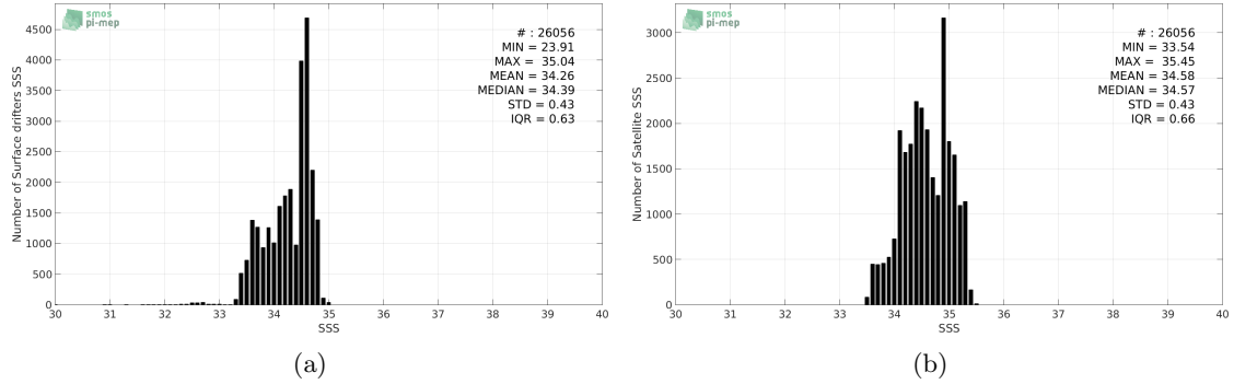
Figure 2: Histograms of SSS from Surface drifters (a) and SMAP-L3-JPL-V4-MONTHLY-60KM (b) considering all match-up pairs per bins of 0.1 over the Indian Ocean Pi-MEP region and for the full satellite product period.
