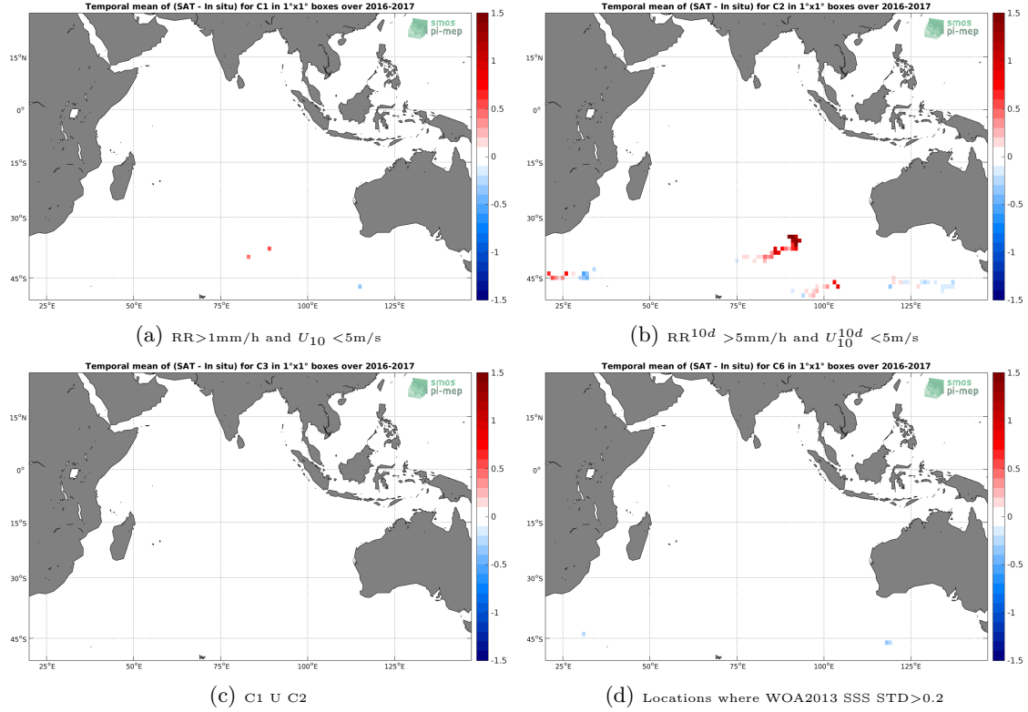
Figure 11: Temporal mean gridded over spatial boxes of size 1^\circ \times 1^\circ of \Delta SSS (SMAP-L3-JPL-V4-MONTHLY-60KM - Surface drifters) for 4 different subdatasets corresponding to: RR > 1\text{mm/h} and U_{10} < 5\text{m/s} (a), RR^{10d} > 5\text{mm/h} and U_{10}^{10d} < 5\text{m/s} (b), C1 U C2 (c), Locations where WOA2013 SSS STD > 0.2 (d).
