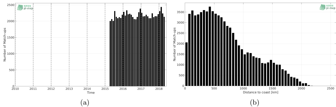
Figure 1: Number of match-ups between Argo and SMAP-L3-JPL-V4-MONTHLY-60KM SSS as a function of time (a) and as function of the distance to coast (b) over the Indian Ocean Pi-MEP region and for the full satellite product period.
