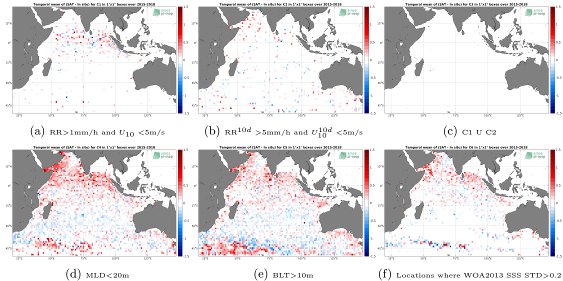
Figure 12: Temporal mean gridded over spatial boxes of size 1^\circ \times 1^\circ of \Delta\text{SSS} (SMAP-L3-JPL-V4-MONTHLY-60KM - Argo) for 6 different subdatasets corresponding to: RR > 1\text{mm/h} and U_{10} < 5\text{m/s} (a), RR^{10d} > 5\text{mm/h} and U_{10}^{10d} < 5\text{m/s} (b), C1 U C2 (c), MLD < 20\text{m} (d), BLT > 10\text{m} (e), Locations where WOA2013 SSS STD > 0.2 (f).
