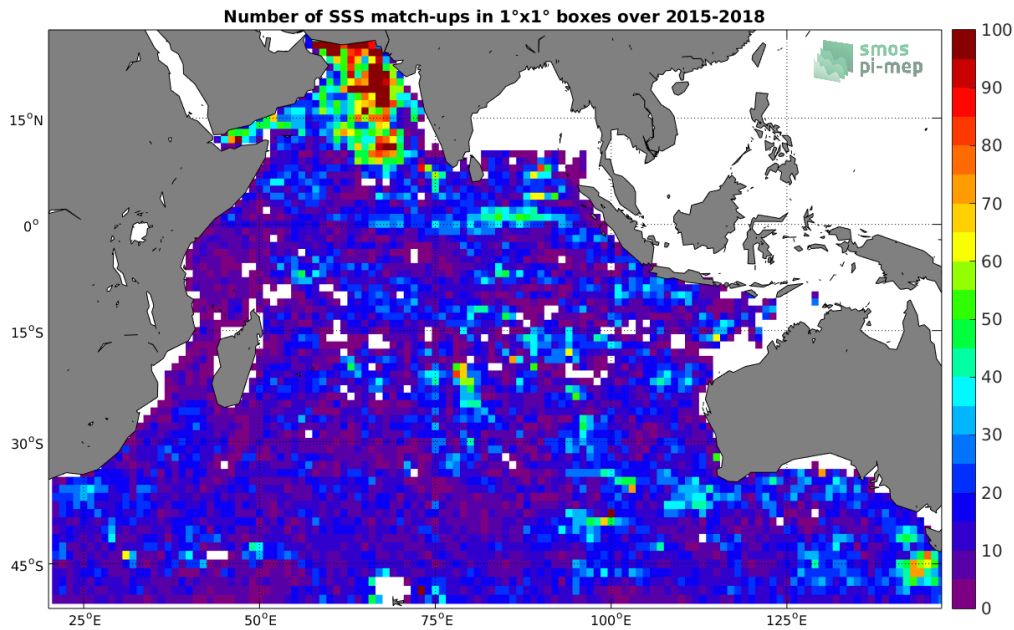
Figure 4: Number of SSS match-ups between Argo SSS and the SMAP-L3-JPL-V4-MONTHLY-60KM SSS product for the Indian Ocean Pi-MEP region over 1°x1° boxes and for the full satellite product period.
