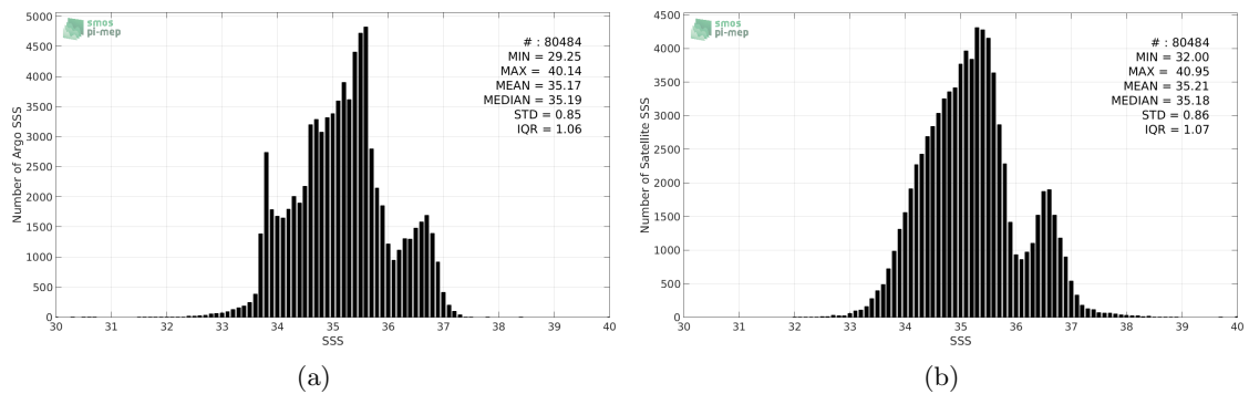
Figure 2: Histograms of SSS from Argo (a) and SMAP-L3-JPL-V4-MONTHLY-60KM (b) considering all match-up pairs per bins of 0.1 over the Indian Ocean Pi-MEP region and for the full satellite product period.
