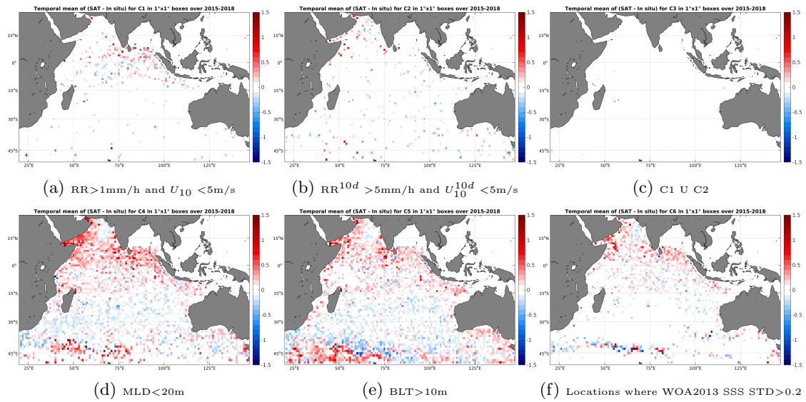
Figure 12: Temporal mean gridded over spatial boxes of size 1^\circ \times 1^\circ of \Delta SSS (SMAP-L3-JPL-V4-MONTHLY-60KM - Argo) for 6 different subdatasets corresponding to:RR>1mm/h and U_{10} < 5\text{m/s} (a), RR^{10d} > 5\text{mm/h} and U_{10}^{10d} < 5\text{m/s} (b), C1 U C2 (c),MLD<20m (d),BLT>10m (e),Locations where WOA2013 SSS STD>0.2 (f).
