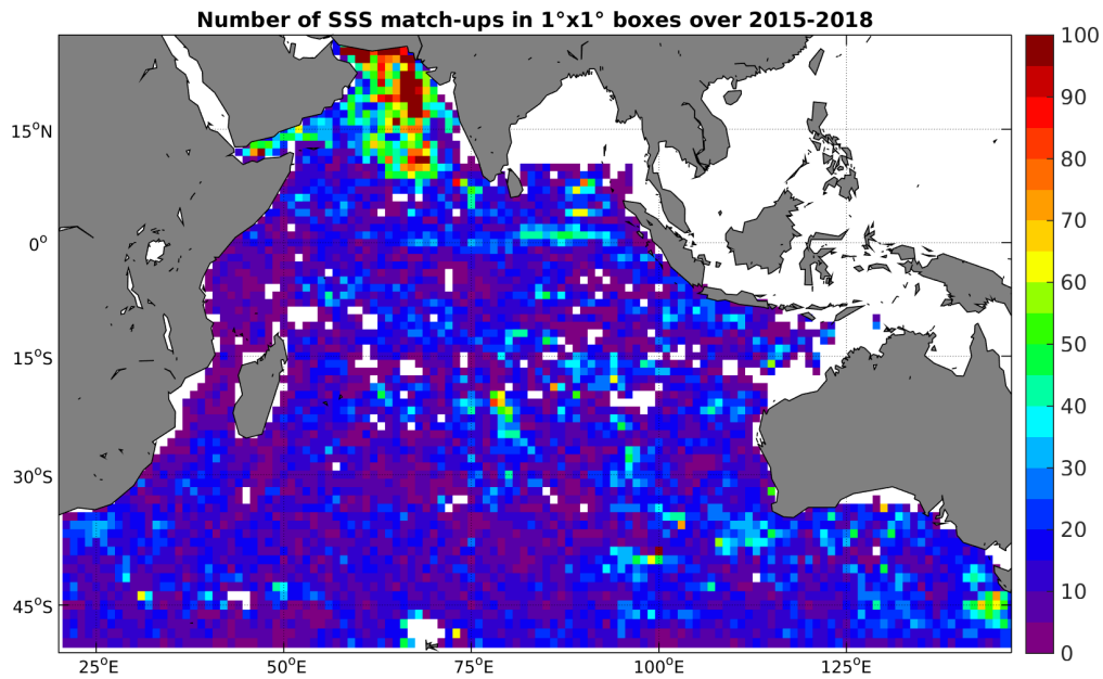
Figure 4: Number of SSS match-ups between Argo SSS and the SMAP-L3-JPL-V4-MONTHLY-60KM SSS product for the Indian Ocean Pi-MEP region over 1^\circ \times 1^\circ boxes and for the full satellite product period.
