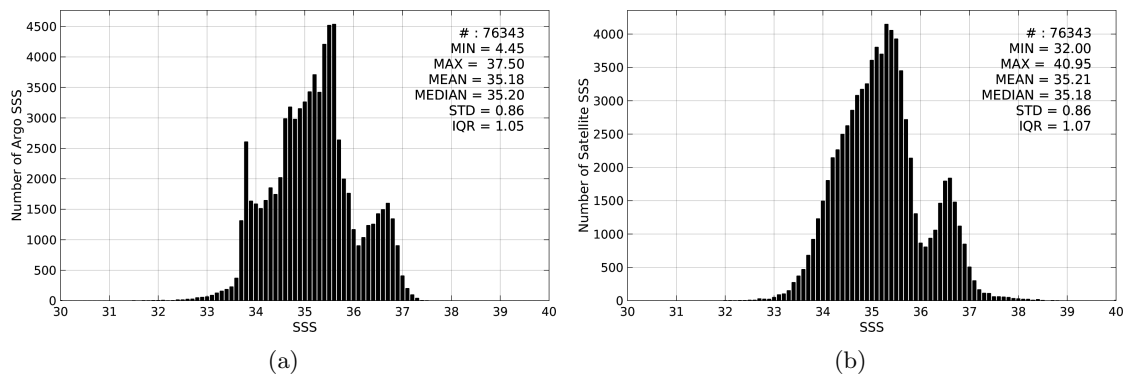
Figure 2: Histograms of SSS from Argo (a) and SMAP-L3-JPL-V4-MONTHLY-60KM (b) considering all match-up pairs per bins of 0.1 over the Indian Ocean Pi-MEP region and for the full satellite product period.
