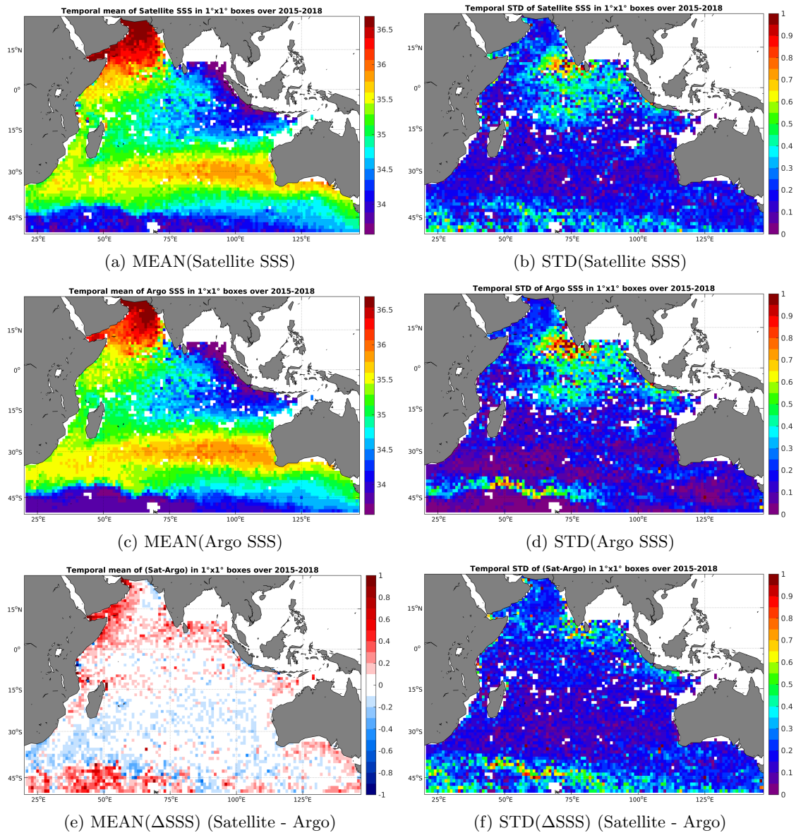
Figure 6: Temporal mean (left) and STD (right) of SSS from SMAP-L3-JPL-V4-MONTHLY-60KM (top), Argo (middle), and of \Delta SSS (Satellite - Argo). Only match-up pairs are used to generate these maps.
