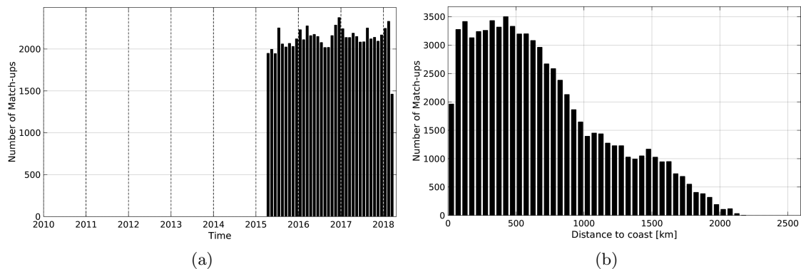
Figure 1: Number of match-ups between Argo and SMAP-L3-JPL-V4-MONTHLY-60KM SSS as a function of time (a) and as function of the distance to coast (b) over the Indian Ocean Pi-MEP region and for the full satellite product period.
