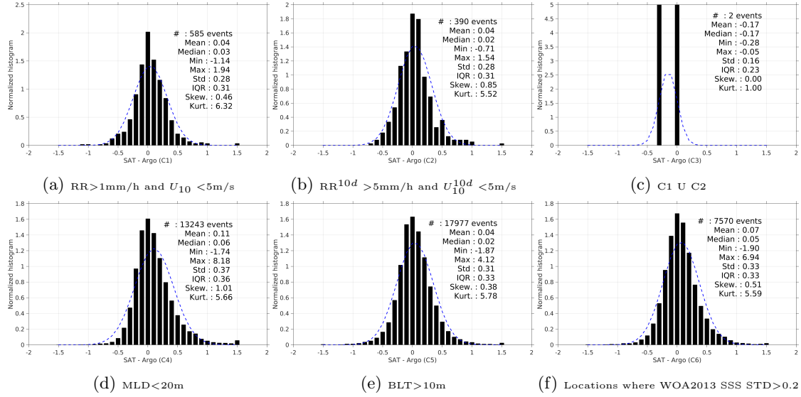
Figure 13: Normalized histogram of \Delta SSS (SMAP-L3-JPL-V4-MONTHLY-60KM - Argo) for 6 different subdatasets corresponding to: RR > 1mm/h and U_{10} < 5 m/s (a), RR^{10d} > 5 mm/h and U_{10}^{10d} < 5 m/s (b), C1 U C2 (c), MLD < 20m (d), BLT > 10m (e), Locations where WOA2013 SSS STD > 0.2 (f).
