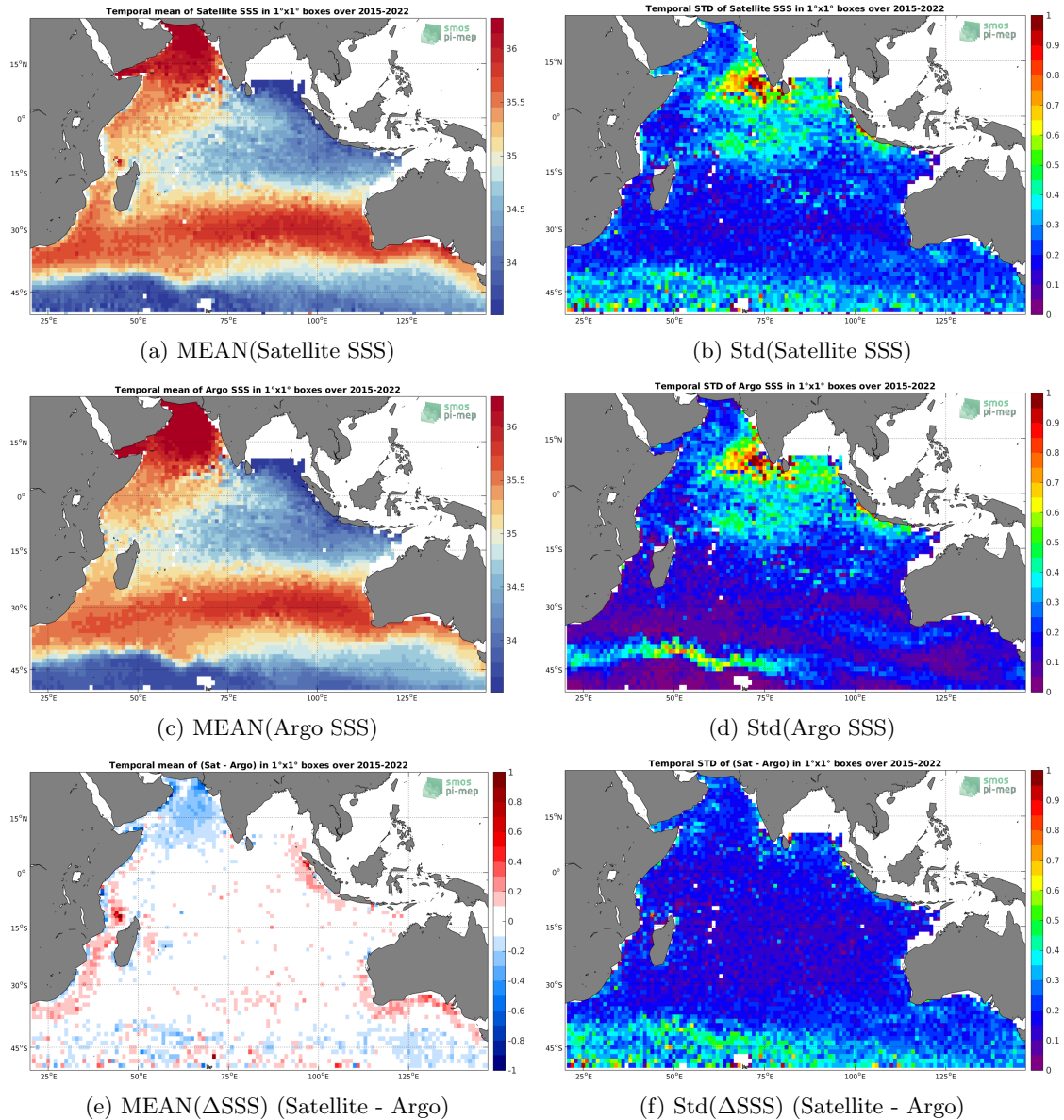
Figure 6: Temporal mean (left) and Std (right) of SSS from SMAP SSS L2-AVERAGED v5 (RSS) (top), Argo (middle), and of \Delta SSS (Satellite - Argo). Only match-up pairs are used to generate these maps.
