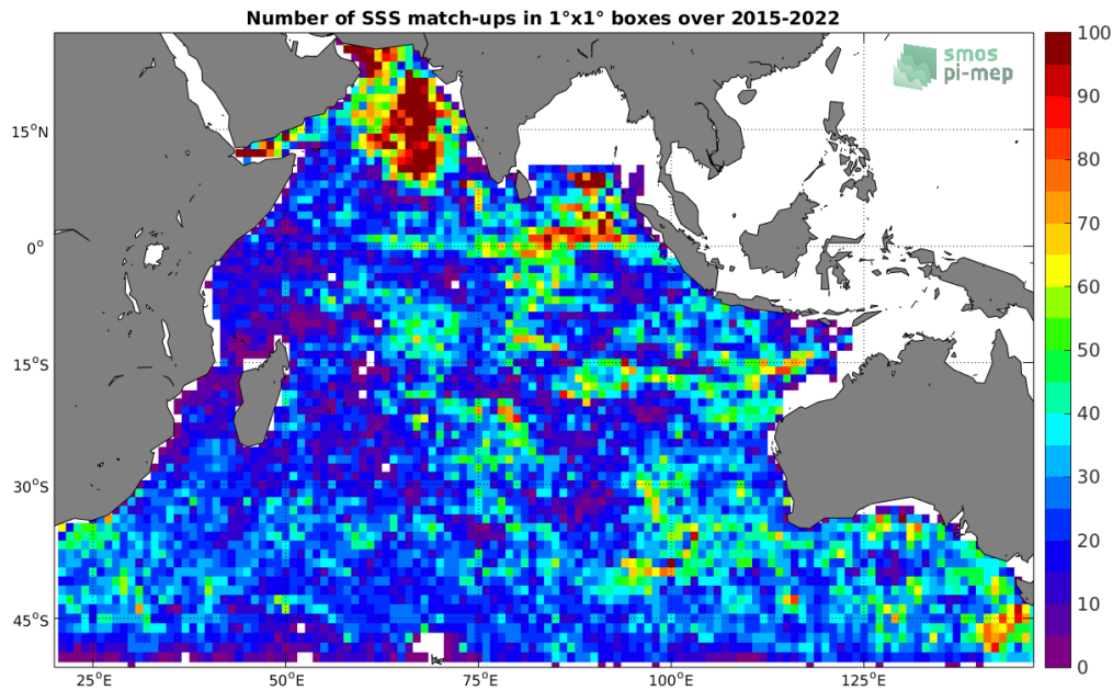
Figure 4: Number of SSS match-ups between Argo SSS and the SMAP SSS L2-AVERAGED v5 (RSS) SSS product for the Indian Ocean Pi-MEP region over 1^\circ \times 1^\circ boxes and for the full satellite product period.
