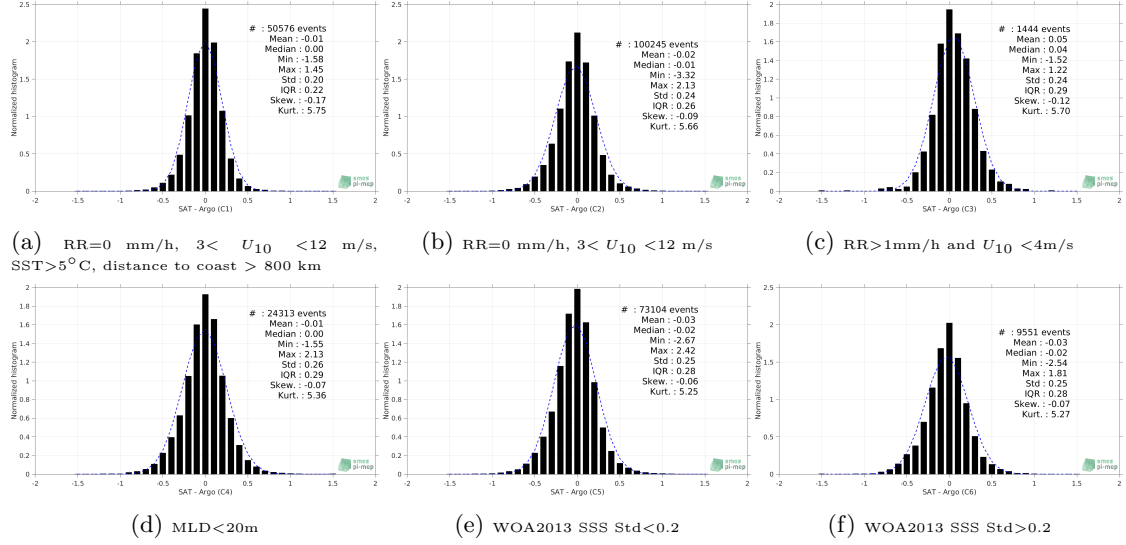
Figure 13: Normalized histogram of \Delta SSS (SMAP SSS L2-AVERAGED v5 (RSS) - Argo) for 6 different subdatasets corresponding to: RR=0 mm/h, 3 < U_{10} < 12 m/s, SST>5°C, distance to coast > 800 km (a), RR=0 mm/h, 3 < U_{10} < 12 m/s (b), RR>1mm/h and U_{10} < 4 m/s (c), MLD<20m (d), WOA2013 SSS Std<0.2 (e), WOA2013 SSS Std>0.2 (f).
