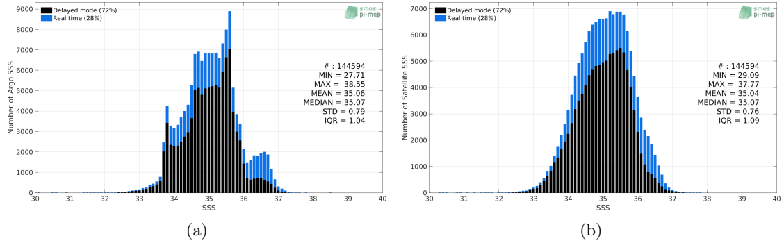
Figure 2: Histograms of SSS from Argo (a) and SMAP SSS L2-AVERAGED v5 (RSS) (b) considering all match-up pairs per bins of 0.1 over the Indian Ocean Pi-MEP region and for the full satellite product period.
