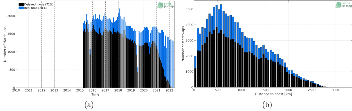
Figure 1: Number of match-ups between Argo and SMAP SSS L2-AVERAGED v5 (RSS) SSS as a function of time (a) and as function of the distance to coast (b) over the Indian Ocean Pi-MEP region and for the full satellite product period.
