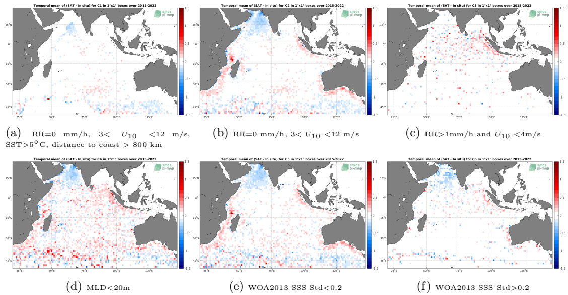
Figure 12: Temporal mean gridded over spatial boxes of size 1^\circ \times 1^\circ of \Delta SSS (SMAP SSS L2-AVERAGED v5 (RSS) - Argo) for 6 different subdatasets corresponding to:RR=0 mm/h, 3 < U_{10} < 12 m/s, SST >5^\circ C, distance to coast > 800 km (a), RR=0 mm/h, 3 < U_{10} < 12 m/s (b), RR >1 mm/h and U_{10} < 4 m/s (c),MLD <20 m (d),WOA2013 SSS Std <0.2 (e),WOA2013 SSS Std >0.2 (f).
