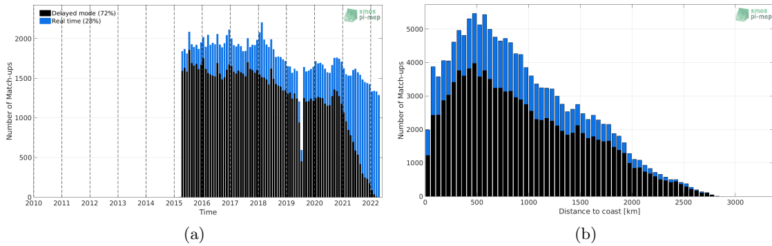
Figure 1: Number of match-ups between Argo and SMAP SSS L2-AVERAGED v5.0 (JPL) SSS as a function of time (a) and as function of the distance to coast (b) over the Indian Ocean Pi-MEP region and for the full satellite product period.
