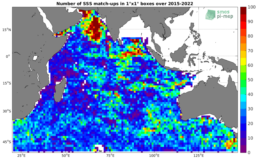
Figure 4: Number of SSS match-ups between Argo SSS and the SMAP SSS L2-AVERAGED v5.0 (JPL) SSS product for the Indian Ocean Pi-MEP region over 1^\circ \times 1^\circ boxes and for the full satellite product period.
