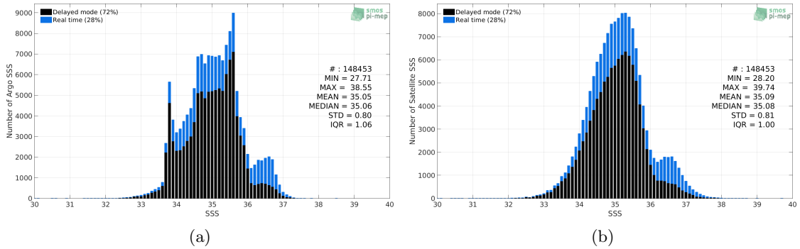
Figure 2: Histograms of SSS from Argo (a) and SMAP SSS L2-AVERAGED v5.0 (JPL) (b) considering all match-up pairs per bins of 0.1 over the Indian Ocean Pi-MEP region and for the full satellite product period.
