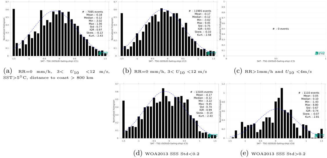
Figure 15: Normalized histogram of \Delta SSS (SMAP SSS L2 v6 (RSS) - TSG (GOSUD-Sailing-ship)) for 5 different subdatasets corresponding to: RR=0 mm/h, 3 < U_{10} < 12 m/s, SST > 5°C, distance to coast > 800 km (a), RR=0 mm/h, 3 < U_{10} < 12 m/s (b), RR > 1mm/h and U_{10} < 4 m/s (c), WOA2013 SSS Std < 0.2 (d), WOA2013 SSS Std > 0.2 (e).
