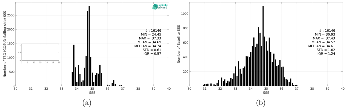
Figure 3: Histograms of SSS from TSG (GOSUD-Sailing-ship) (a) and SMAP SSS L2 v6 (RSS) (b) considering all match-up pairs per bins of 0.1 over the Indian Ocean Pi-MEP region and for the full satellite product period.
