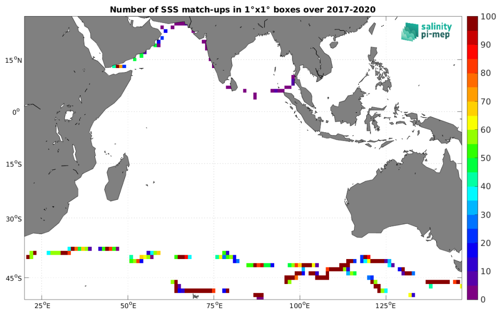
Figure 5: Number of SSS match-ups between TSG (GOSUD-Sailing-ship) SSS and the SMAP SSS L2 v6 (RSS) SSS product for the Indian Ocean Pi-MEP region over 1^\circ \times 1^\circ boxes and for the full satellite product period.
