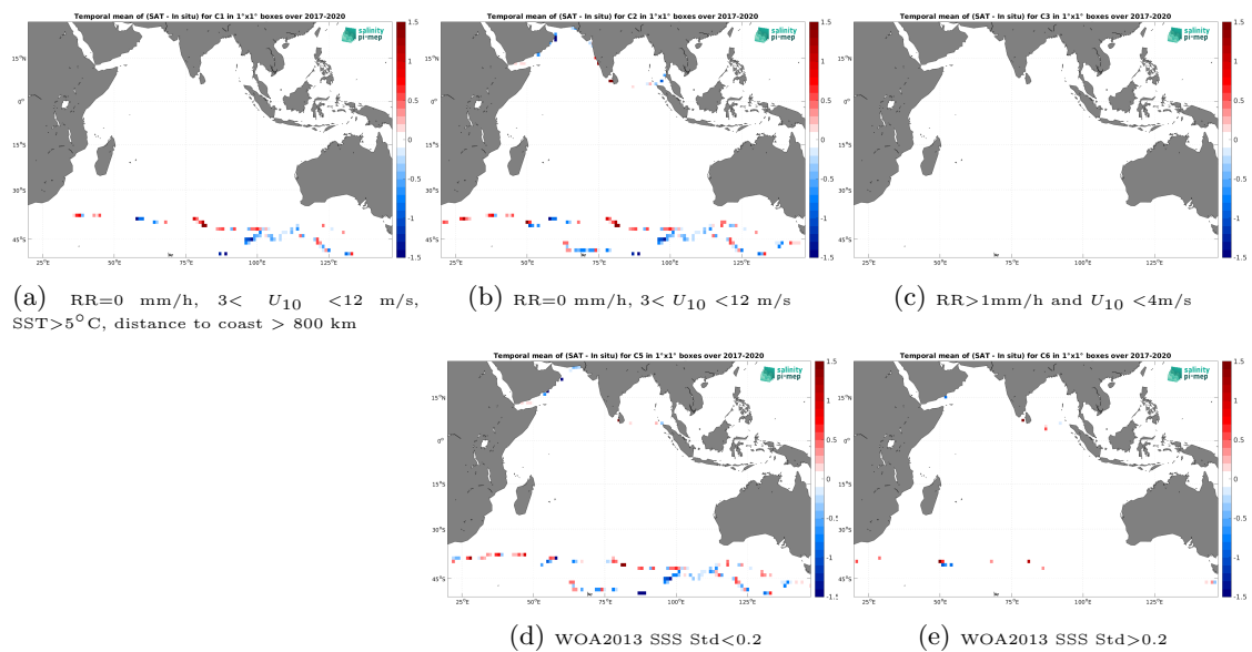
Figure 14: Temporal mean gridded over spatial boxes of size 1^\circ \times 1^\circ of \Delta SSS (SMAP SSS L2 v6 (RSS) - TSG (GOSUD-Sailing-ship)) for 5 different subdatasets corresponding to:RR=0 mm/h, 3 < U_{10} < 12 m/s, SST > 5^\circ\text{C} , distance to coast > 800 km (a), RR=0 mm/h, 3 < U_{10} < 12 m/s (b), RR > 1 mm/h and U_{10} < 4 m/s (c), WOA2013 SSS Std < 0.2 (d), WOA2013 SSS Std > 0.2 (e).
