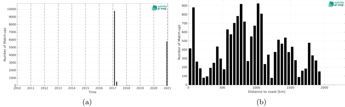
Figure 2: Number of match-ups between TSG (GOSUD-Sailing-ship) and SMAP SSS L2 v6 (RSS) SSS as a function of time (a) and as function of the distance to coast (b) over the Indian Ocean Pi-MEP region and for the full satellite product period.
