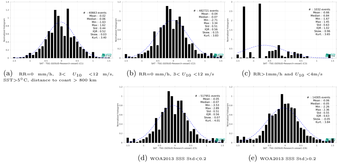
Figure 15: Normalized histogram of \Delta SSS (SMAP SSS L2 v6 (RSS) - TSG (GOSUD-Research-vessel)) for 5 different subdatasets corresponding to: RR=0 mm/h, 3 < U_{10} < 12 m/s, SST > 5°C, distance to coast > 800 km (a), RR=0 mm/h, 3 < U_{10} < 12 m/s (b), RR > 1mm/h and U_{10} < 4 m/s (c), WOA2013 SSS Std < 0.2 (d), WOA2013 SSS Std > 0.2 (e).
