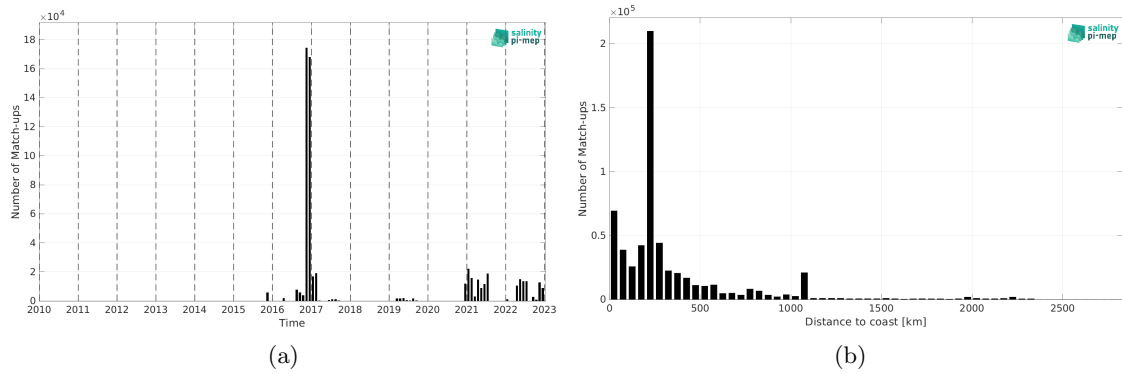
Figure 2: Number of match-ups between TSG (GOSUD-Research-vessel) and SMAP SSS L2 v6 (RSS) SSS as a function of time (a) and as function of the distance to coast (b) over the Indian Ocean Pi-MEP region and for the full satellite product period.
