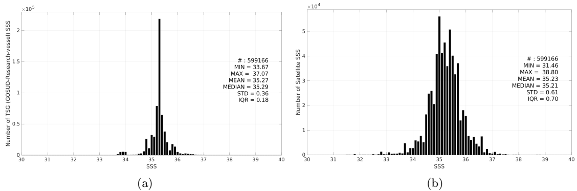
Figure 3: Histograms of SSS from TSG (GOSUD-Research-vessel) (a) and SMAP SSS L2 v6 (RSS) (b) considering all match-up pairs per bins of 0.1 over the Indian Ocean Pi-MEP region and for the full satellite product period.
