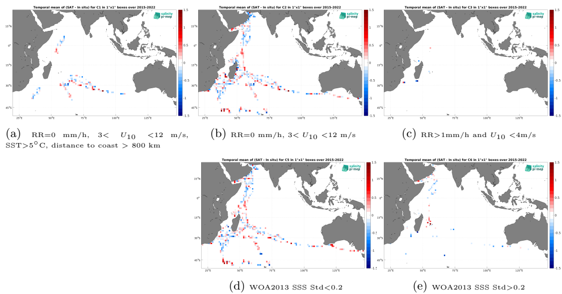
Figure 14: Temporal mean gridded over spatial boxes of size 1^\circ \times 1^\circ of \Delta SSS (SMAP SSS L2 v6 (RSS) - TSG (GOSUD-Research-vessel)) for 5 different subdatasets corresponding to:RR=0 mm/h, 3 < U_{10} < 12 m/s, SST > 5^\circ\text{C} , distance to coast > 800 km (a), RR=0 mm/h, 3 < U_{10} < 12 m/s (b), RR > 1 mm/h and U_{10} < 4 m/s (c), WOA2013 SSS Std < 0.2 (d), WOA2013 SSS Std > 0.2 (e).
