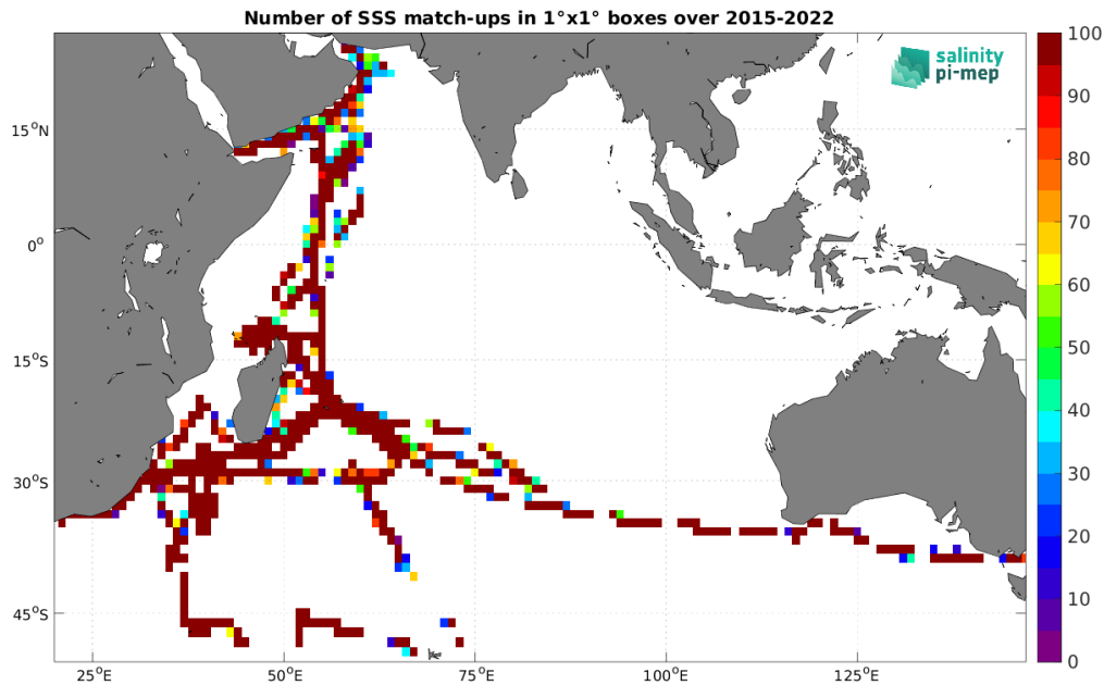
Figure 5: Number of SSS match-ups between TSG (GOSUD-Research-vessel) SSS and the SMAP SSS L2 v6 (RSS) SSS product for the Indian Ocean Pi-MEP region over 1^\circ \times 1^\circ boxes and for the full satellite product period.
