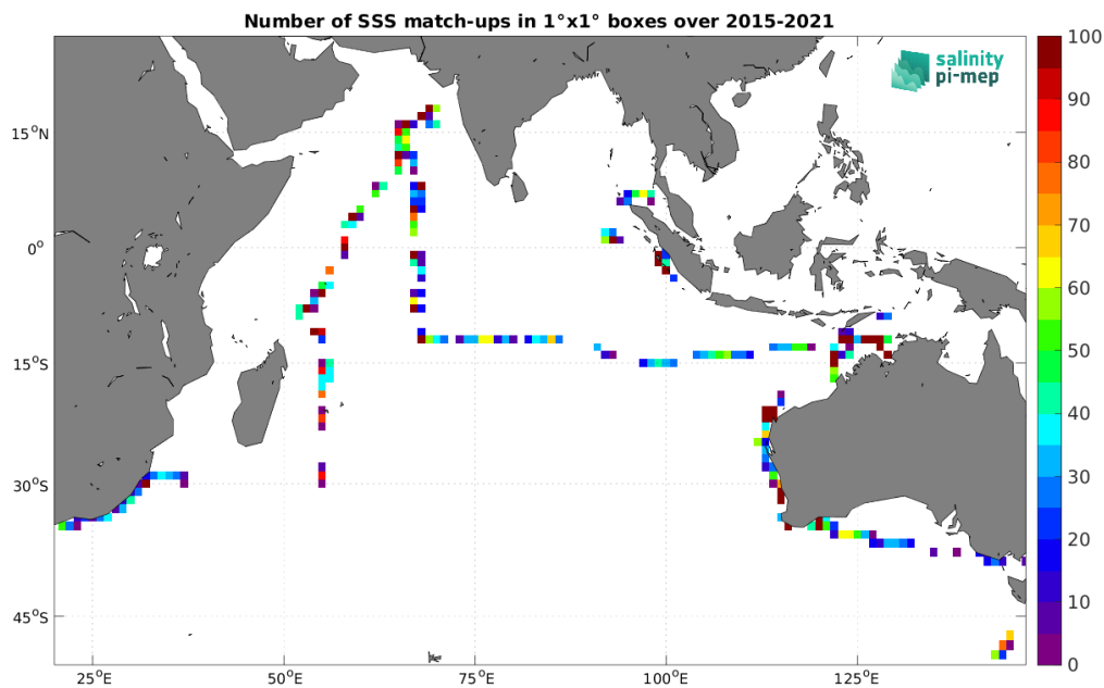
Figure 5: Number of SSS match-ups between TSG (SAMOS) SSS and the SMAP SSS L2 v6 - 40 km (RSS) SSS product for the Indian Ocean Pi-MEP region over 1^\circ \times 1^\circ boxes and for the full satellite product period.
