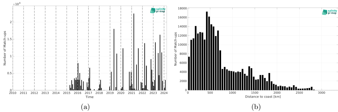
Figure 2: Number of match-ups between TSG (LEGOS-DM) and SMAP SSS L2 v6 - 40 km (RSS) SSS as a function of time (a) and as function of the distance to coast (b) over the Indian Ocean Pi-MEP region and for the full satellite product period.
