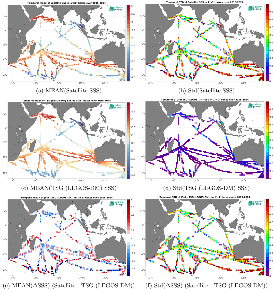
Figure 7: Temporal mean (left) and Std (right) of SSS from SMAP SSS L2 v6 - 40 km (RSS) (top), TSG (LEGOS-DM) (middle), and of \Delta SSS (Satellite - TSG (LEGOS-DM)). Only match-up pairs are used to generate these maps.
