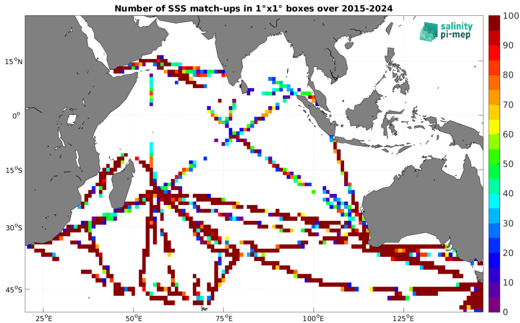
Figure 5: Number of SSS match-ups between TSG (LEGOS-DM) SSS and the SMAP SSS L2 v6 - 40 km (RSS) SSS product for the Indian Ocean Pi-MEP region over 1^\circ \times 1^\circ boxes and for the full satellite product period.
