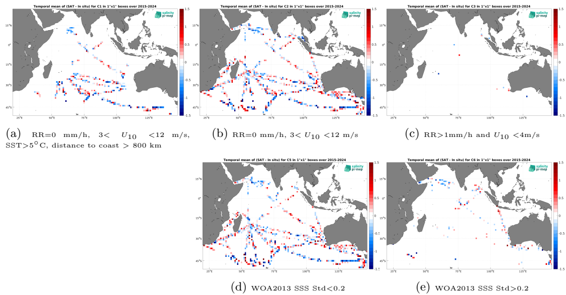
Figure 14: Temporal mean gridded over spatial boxes of size 1^\circ \times 1^\circ of \Delta SSS (SMAP SSS L2 v6 - 40 km (RSS) - TSG (LEGOS-DM)) for 5 different subdatasets corresponding to:RR=0 mm/h, 3 < U_{10} < 12 m/s, SST > 5^\circ\text{C} , distance to coast > 800 km (a), RR=0 mm/h, 3 < U_{10} < 12 m/s (b), RR > 1 mm/h and U_{10} < 4 m/s (c), WOA2013 SSS Std < 0.2 (d), WOA2013 SSS Std > 0.2 (e).
