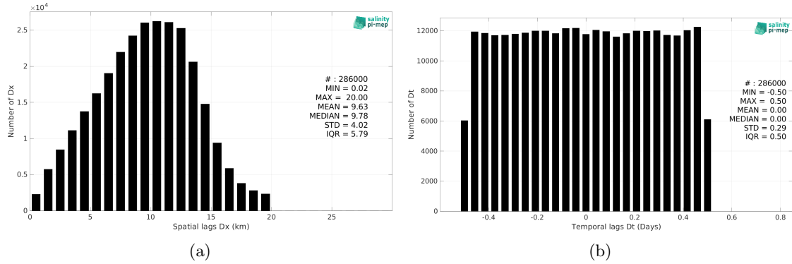
Figure 6: Histograms of the spatial (a) and temporal (b) lags between the location/time of the TSG (LEGOS-DM) measurement and the date of the corresponding SMAP SSS L2 v6 - 40 km (RSS) SSS pixel.
