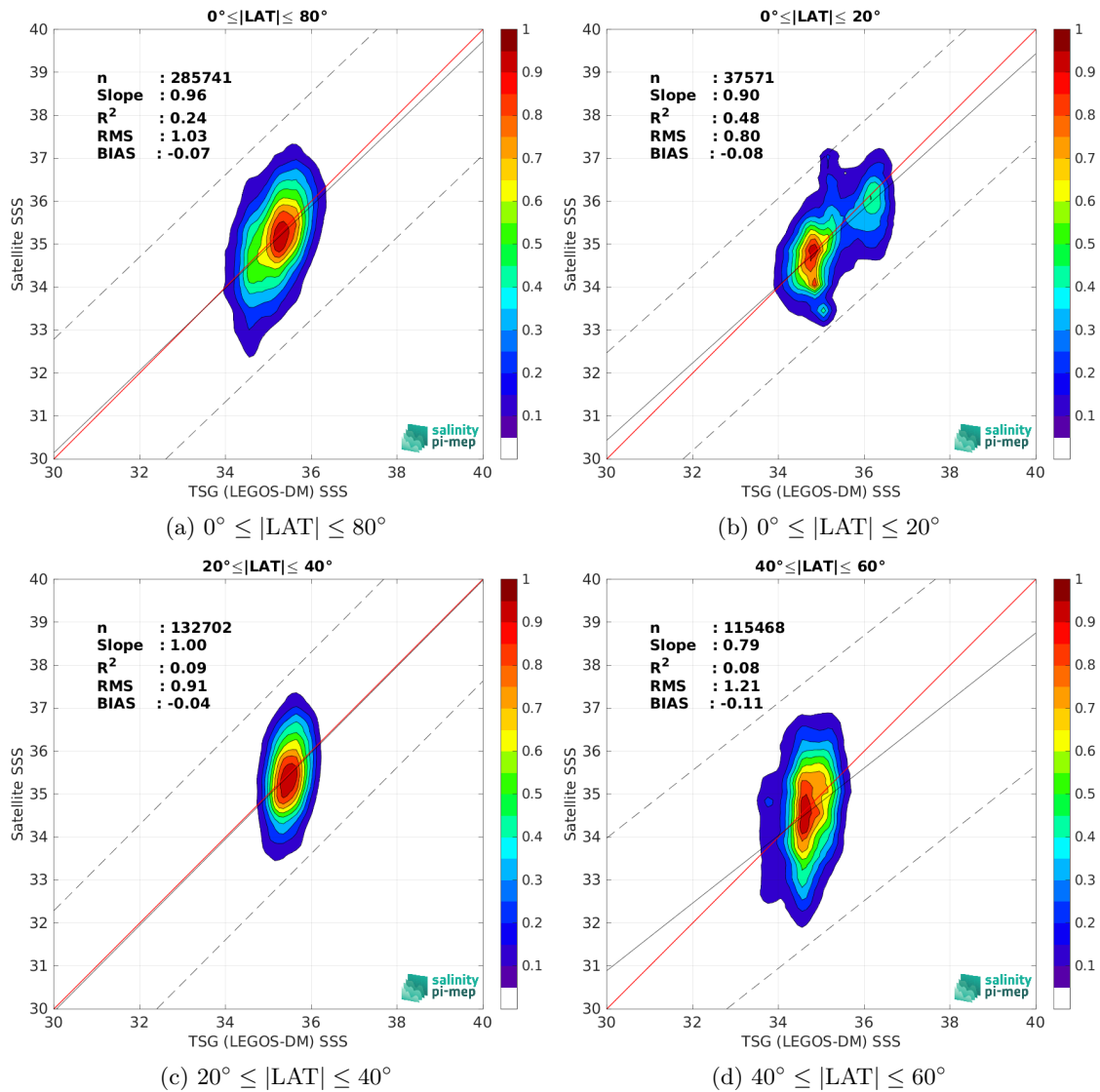
Figure 10: Contour maps of the concentration of SMAP SSS L2 v6 - 40 km (RSS) SSS (y-axis) versus TSG (LEGOS-DM) SSS (x-axis) at match-up pairs for different latitude bands. For each plot, the red line shows x=y . The black thin and dashed lines indicate a linear fit through the data cloud and the \pm 95\% confidence levels, respectively. The number match-up pairs n , the slope and R^2 coefficient of the linear fit, the root mean square (RMS) and the mean bias between satellite and in situ data are indicated for each latitude band in each plots.
