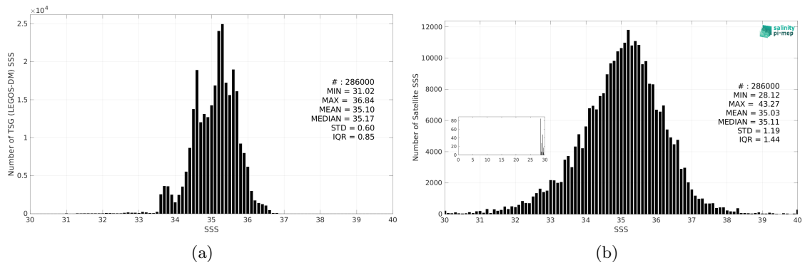
Figure 3: Histograms of SSS from TSG (LEGOS-DM) (a) and SMAP SSS L2 v6 - 40 km (RSS) (b) considering all match-up pairs per bins of 0.1 over the Indian Ocean Pi-MEP region and for the full satellite product period.
