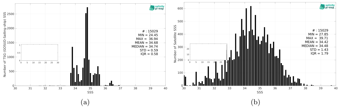
Figure 3: Histograms of SSS from TSG (GOSUD-Sailing-ship) (a) and SMAP SSS L2 v6 - 40 km (RSS) (b) considering all match-up pairs per bins of 0.1 over the Indian Ocean Pi-MEP region and for the full satellite product period.
