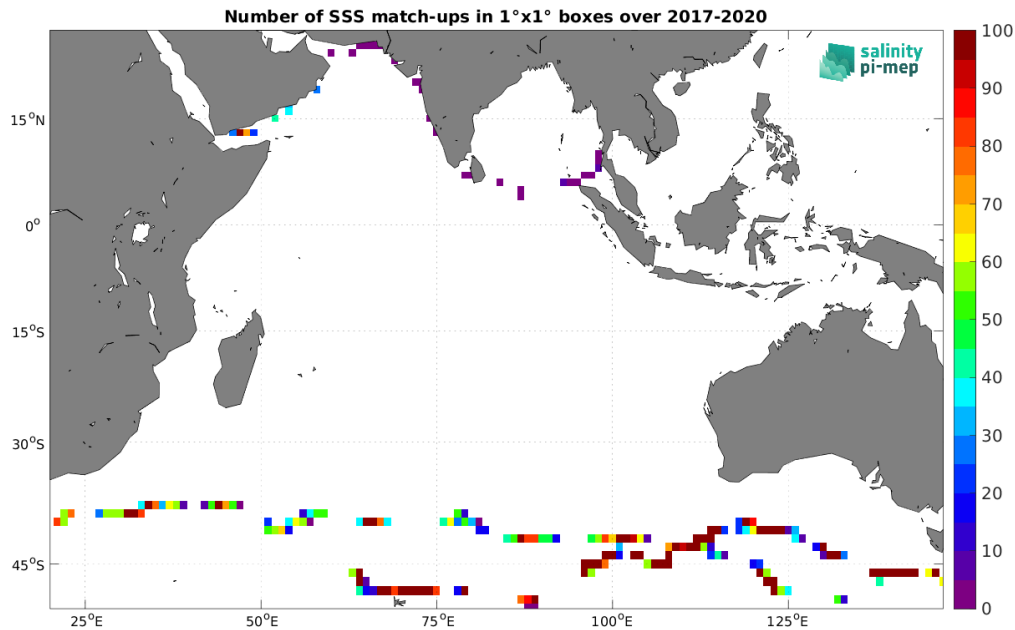
Figure 5: Number of SSS match-ups between TSG (GOSUD-Sailing-ship) SSS and the SMAP SSS L2 v6 - 40 km (RSS) SSS product for the Indian Ocean Pi-MEP region over 1^\circ \times 1^\circ boxes and for the full satellite product period.
