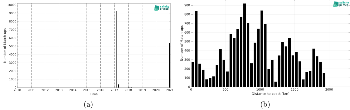
Figure 2: Number of match-ups between TSG (GOSUD-Sailing-ship) and SMAP SSS L2 v6 - 40 km (RSS) SSS as a function of time (a) and as function of the distance to coast (b) over the Indian Ocean Pi-MEP region and for the full satellite product period.
