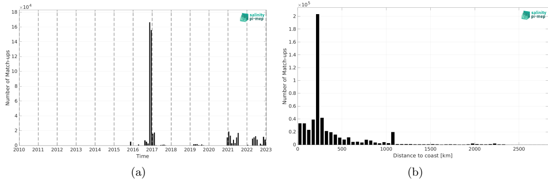
Figure 2: Number of match-ups between TSG (GOSUD-Research-vessel) and SMAP SSS L2 v6 - 40 km (RSS) SSS as a function of time (a) and as function of the distance to coast (b) over the Indian Ocean Pi-MEP region and for the full satellite product period.
