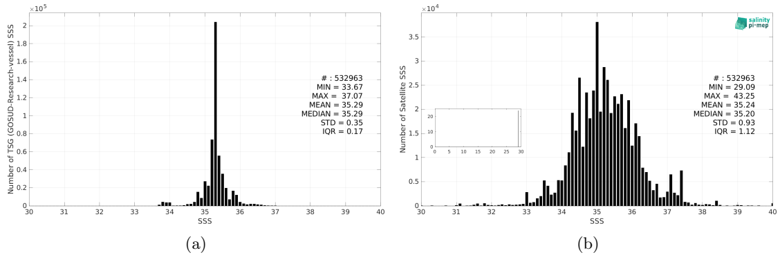
Figure 3: Histograms of SSS from TSG (GOSUD-Research-vessel) (a) and SMAP SSS L2 v6 - 40 km (RSS) (b) considering all match-up pairs per bins of 0.1 over the Indian Ocean Pi-MEP region and for the full satellite product period.
