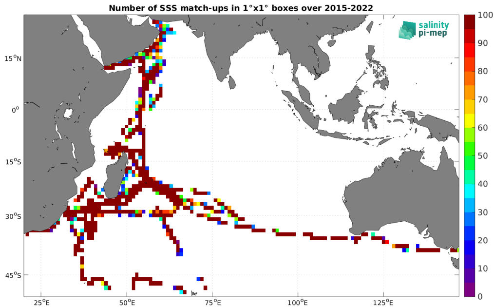
Figure 5: Number of SSS match-ups between TSG (GOSUD-Research-vessel) SSS and the SMAP SSS L2 v6 - 40 km (RSS) SSS product for the Indian Ocean Pi-MEP region over 1^\circ \times 1^\circ boxes and for the full satellite product period.
