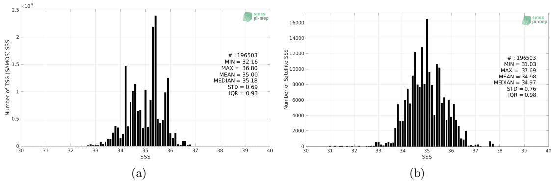
Figure 2: Histograms of SSS from TSG (SAMOS) (a) and SMAP SSS L2 v5 (RSS) (b) considering all match-up pairs per bins of 0.1 over the Indian Ocean Pi-MEP region and for the full satellite product period.
