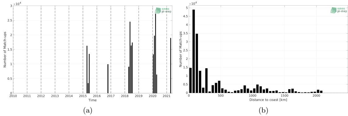
Figure 1: Number of match-ups between TSG (SAMOS) and SMAP SSS L2 v5 (RSS) SSS as a function of time (a) and as function of the distance to coast (b) over the Indian Ocean Pi-MEP region and for the full satellite product period.
