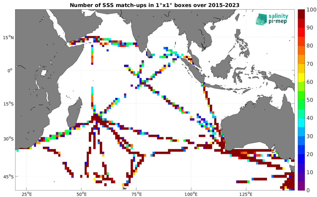
Figure 4: Number of SSS match-ups between TSG (LEGOS-DM) SSS and the SMAP SSS L2 v5 (RSS) SSS product for the Indian Ocean Pi-MEP region over 1^\circ \times 1^\circ boxes and for the full satellite product period.
