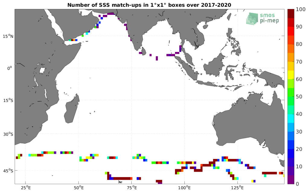
Figure 4: Number of SSS match-ups between TSG (GOSUD-Sailing-ship) SSS and the SMAP SSS L2 v5 (RSS) SSS product for the Indian Ocean Pi-MEP region over 1^\circ \times 1^\circ boxes and for the full satellite product period.
