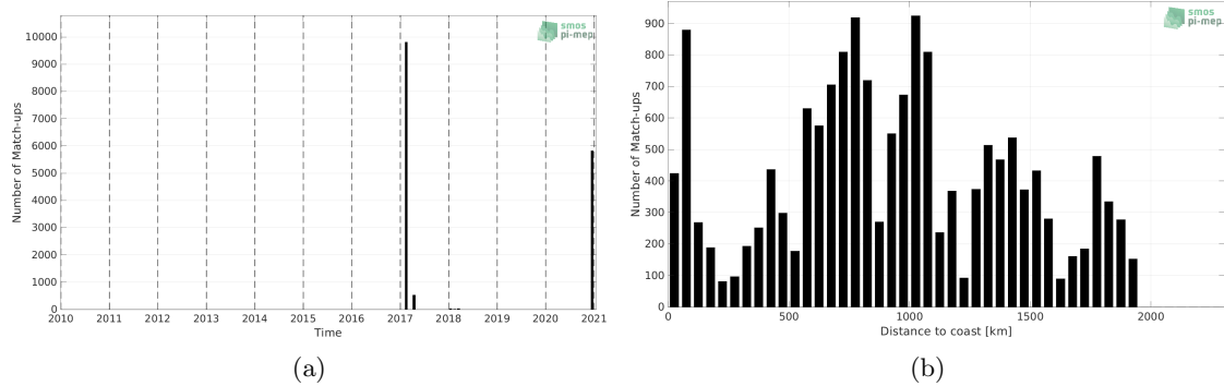
Figure 1: Number of match-ups between TSG (GOSUD-Sailing-ship) and SMAP SSS L2 v5 (RSS) SSS as a function of time (a) and as function of the distance to coast (b) over the Indian Ocean Pi-MEP region and for the full satellite product period.
