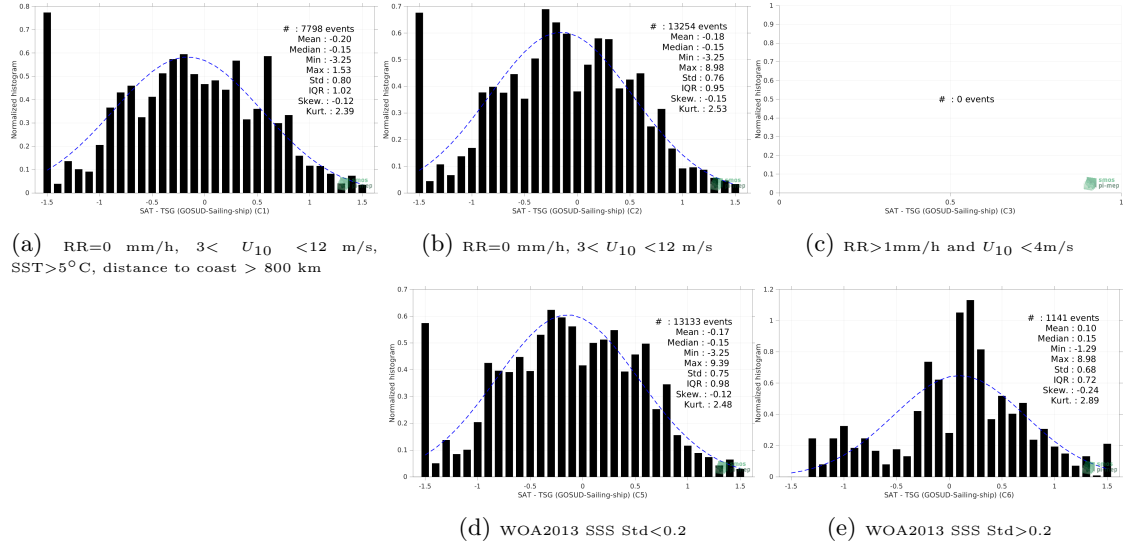
Figure 13: Normalized histogram of \Delta SSS (SMAP SSS L2 v5 (RSS) - TSG (GOSUD-Sailing-ship)) for 5 different subdatasets corresponding to: RR=0 mm/h, 3 < U_{10} < 12 m/s, SST > 5°C, distance to coast > 800 km (a), RR=0 mm/h, 3 < U_{10} < 12 m/s (b), RR > 1mm/h and U_{10} < 4 m/s (c), WOA2013 SSS Std < 0.2 (d), WOA2013 SSS Std > 0.2 (e).
