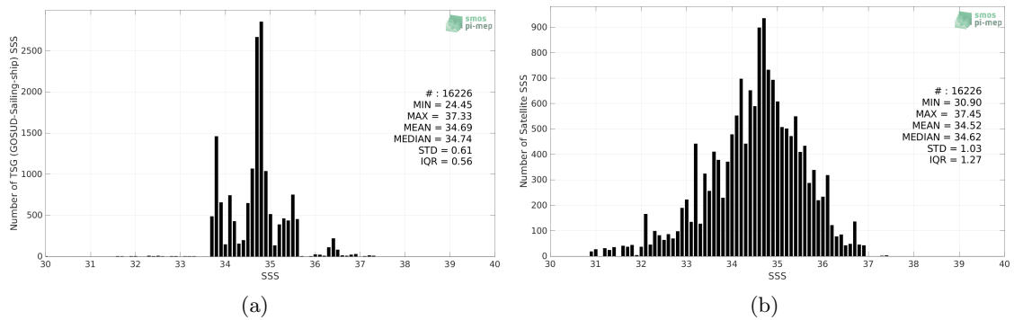
Figure 2: Histograms of SSS from TSG (GOSUD-Sailing-ship) (a) and SMAP SSS L2 v5 (RSS) (b) considering all match-up pairs per bins of 0.1 over the Indian Ocean Pi-MEP region and for the full satellite product period.
